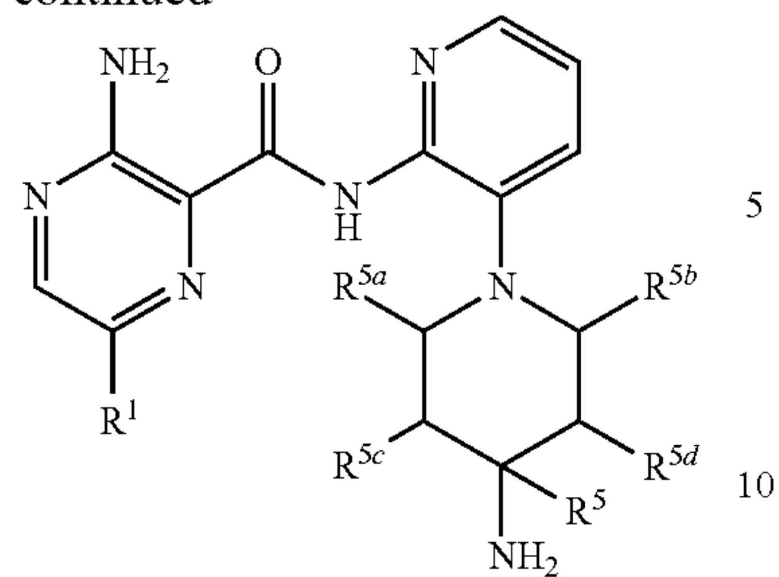
Compound of Formula I
