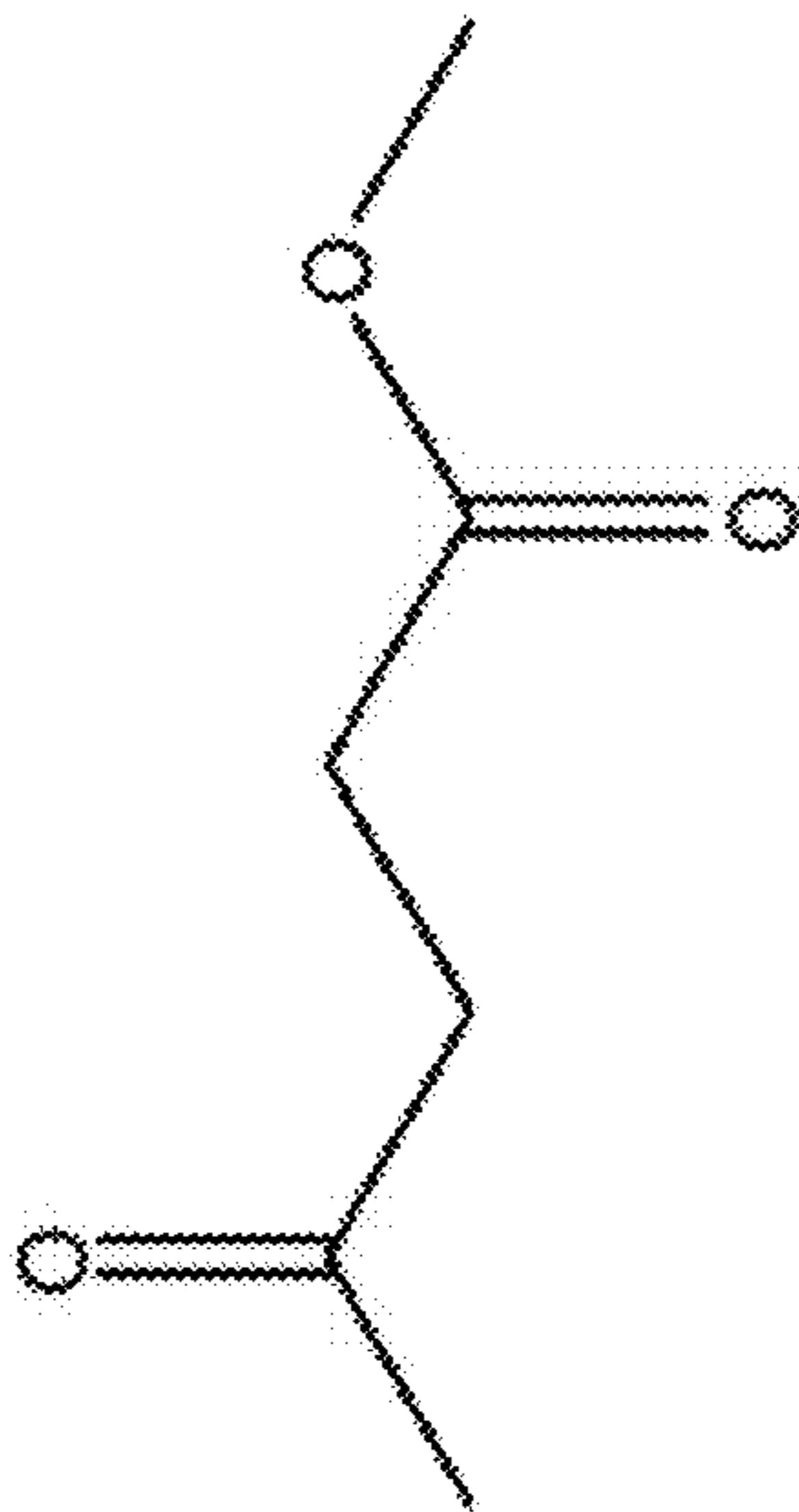
Methyl levulinate
