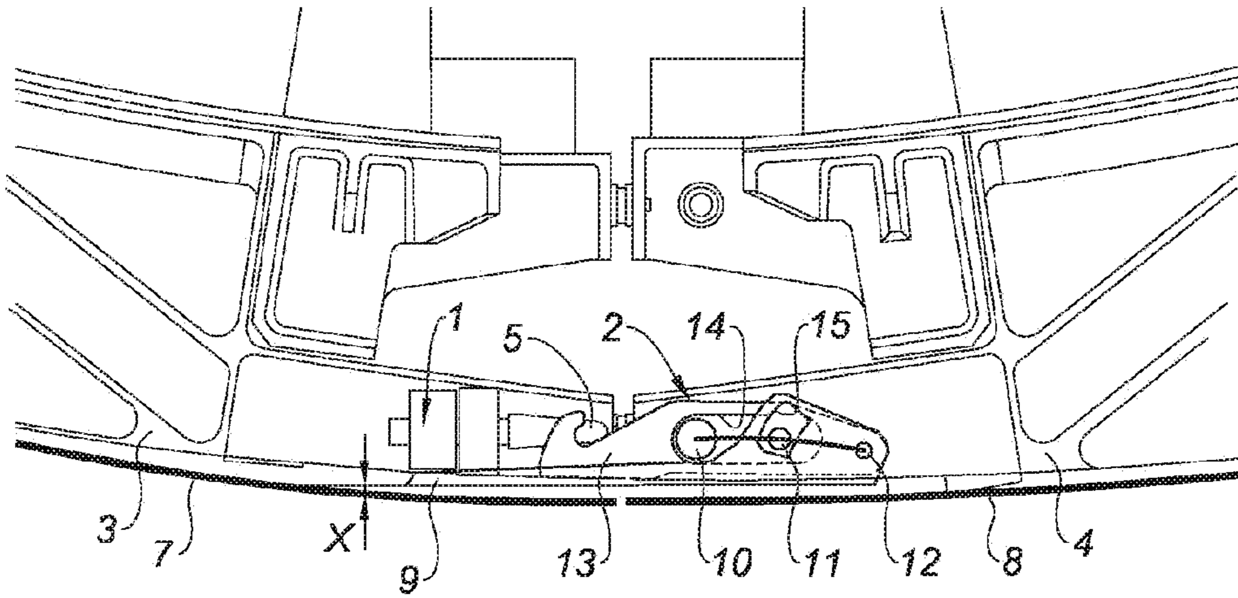
Fig. 1 PRIOR ART
