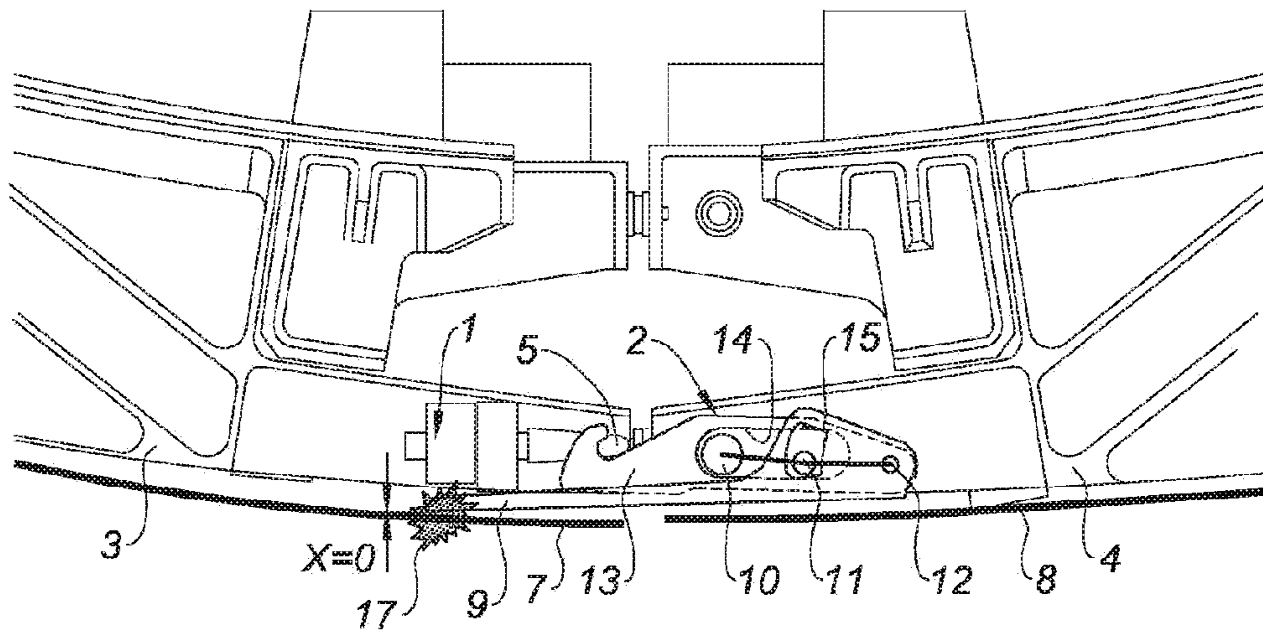
Fig. 5 PRIOR ART
