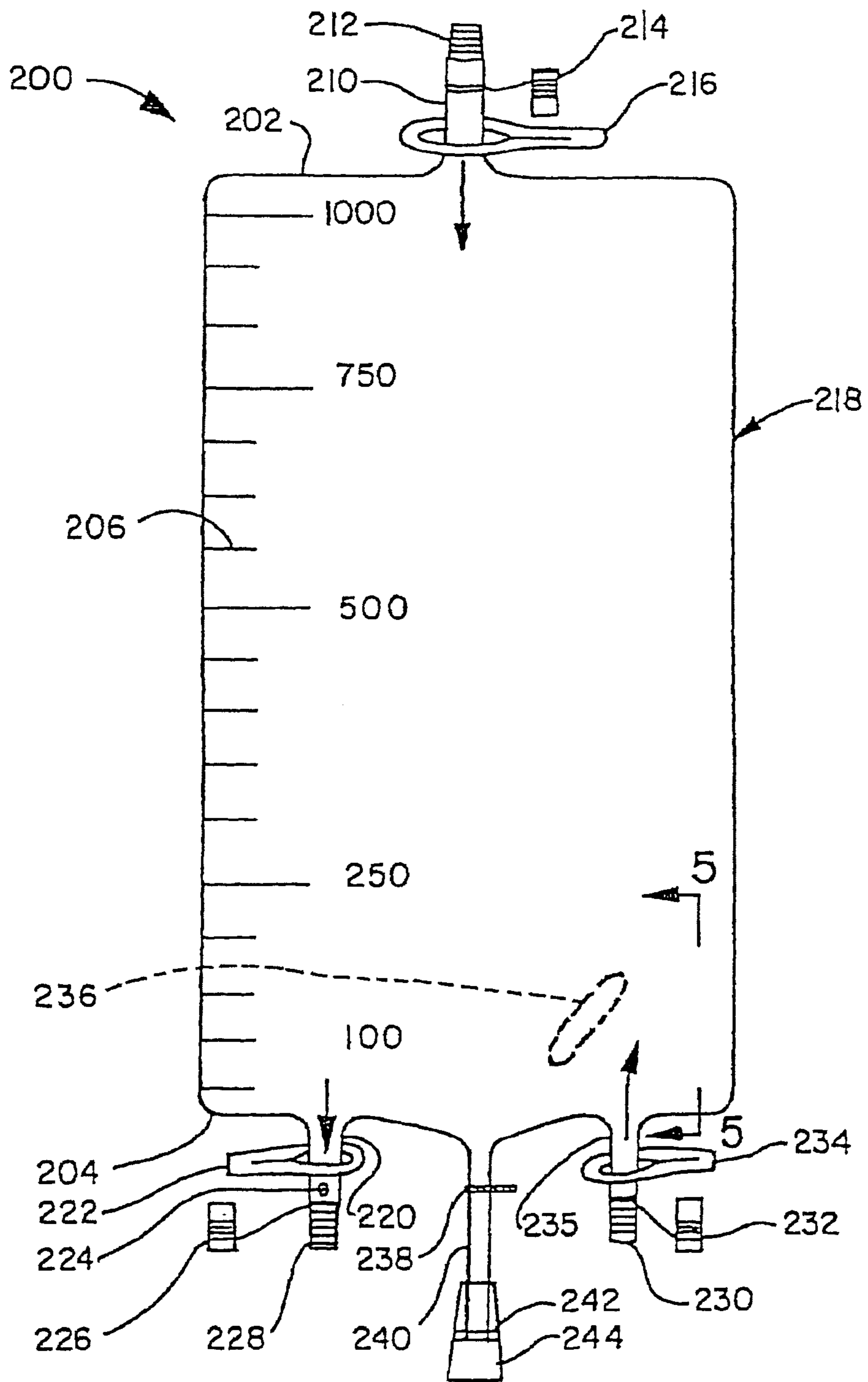
FIG. 4 (PRIOR ART)
