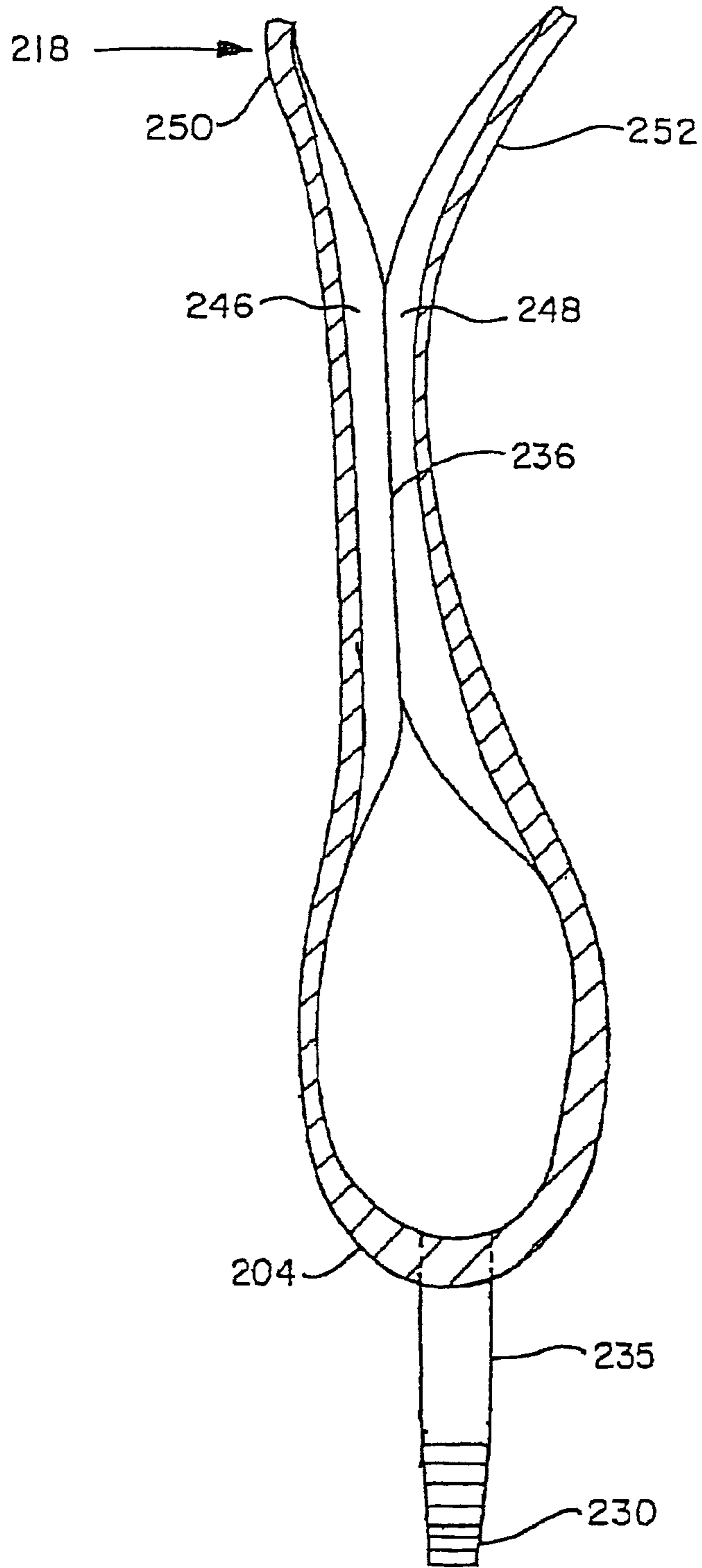
FIG. 5 (PRIOR ART)
