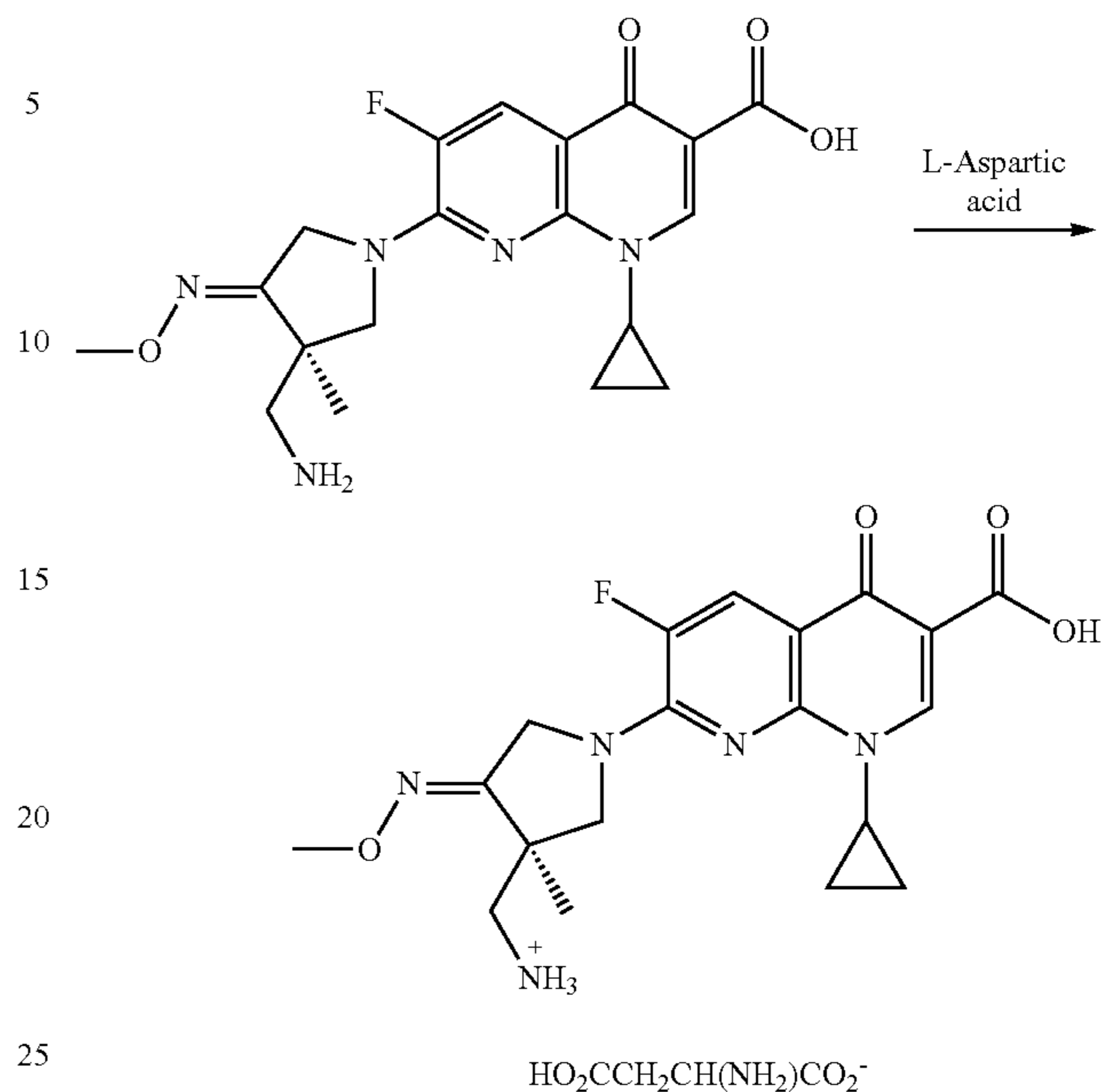
[Reaction FIG. 1]
