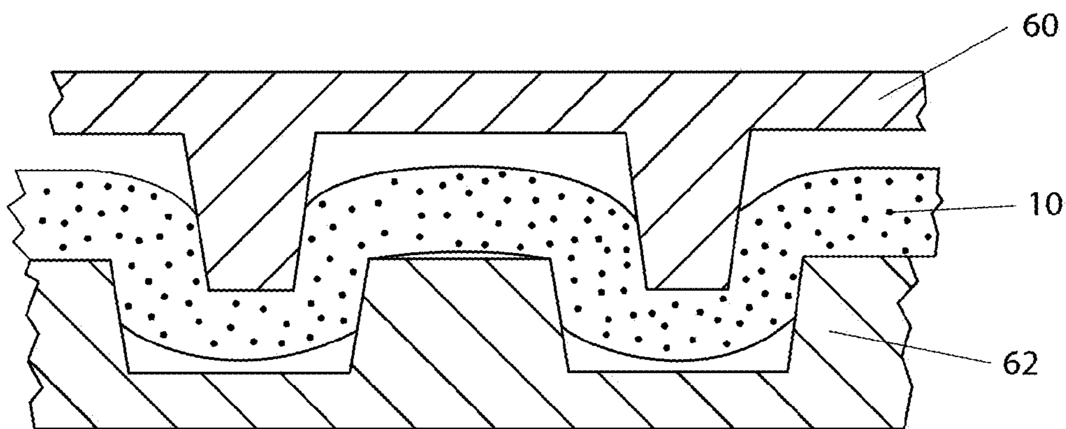
Fig. 14 Prior Art
