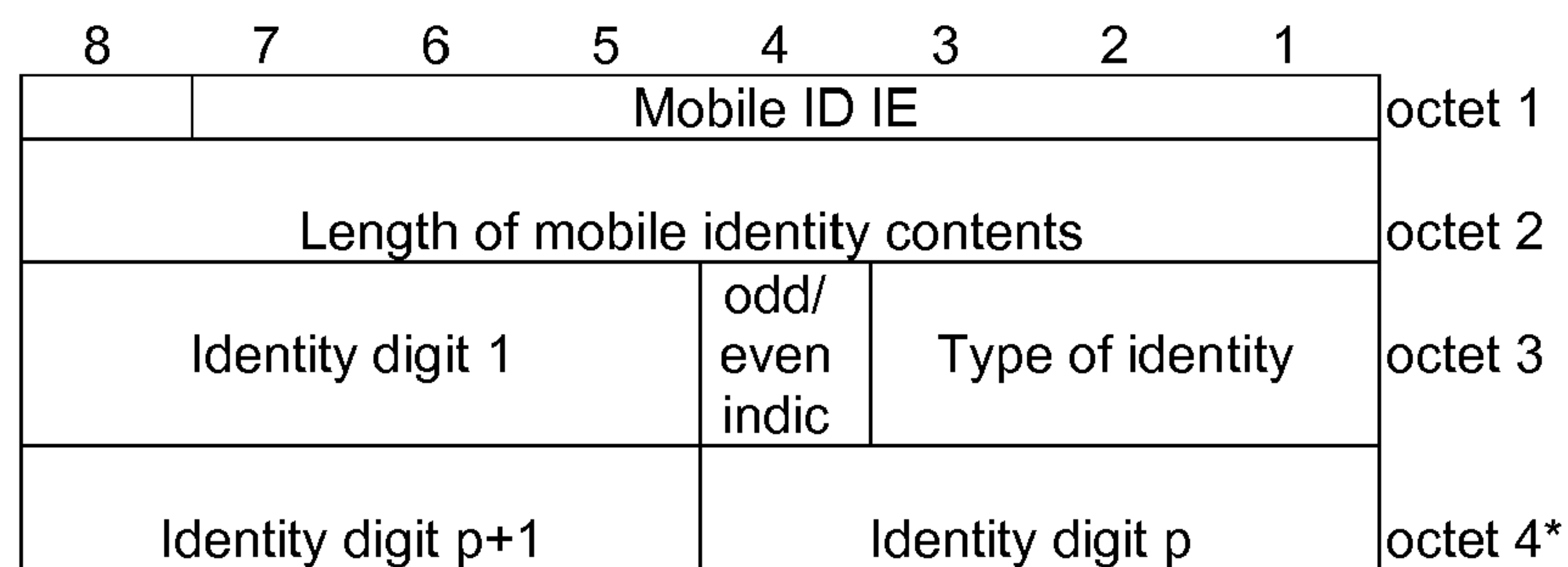
Figure 10.5.4/3GPP TS 24.008 Mobile Identity information element
