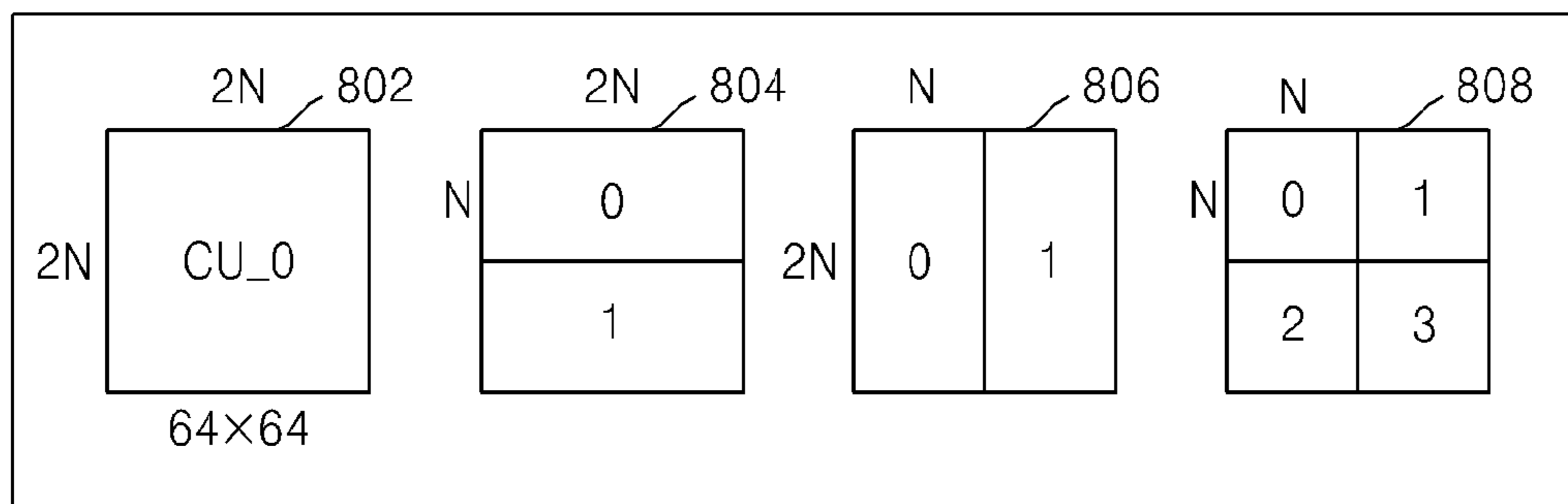
PARTITION TYPE (800)
