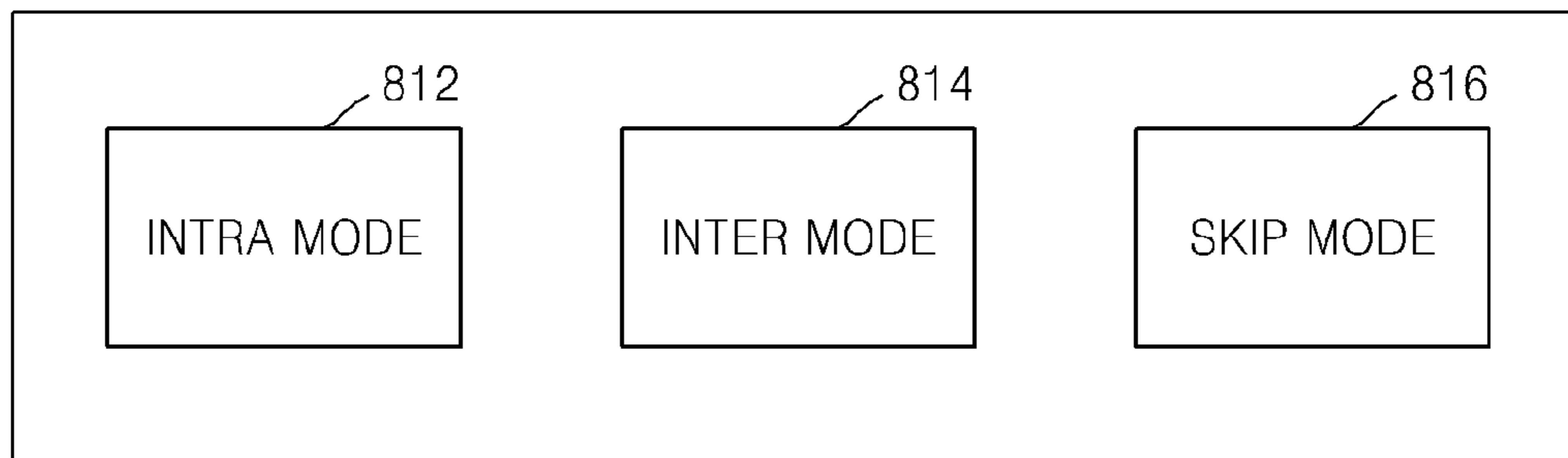
PREDICTION MODE (810)
