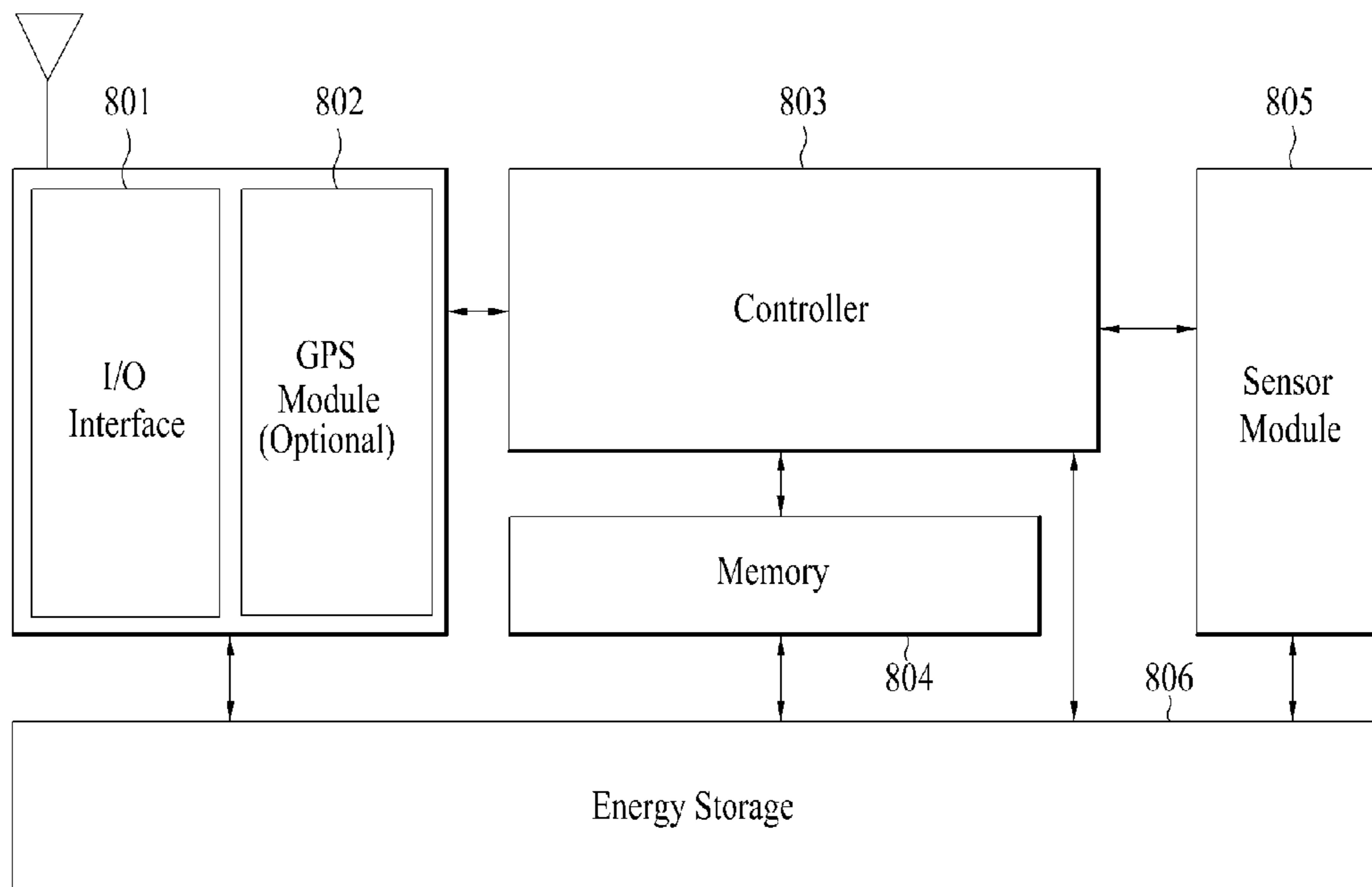
Hybrid V-MIMO Device Block Diagram
