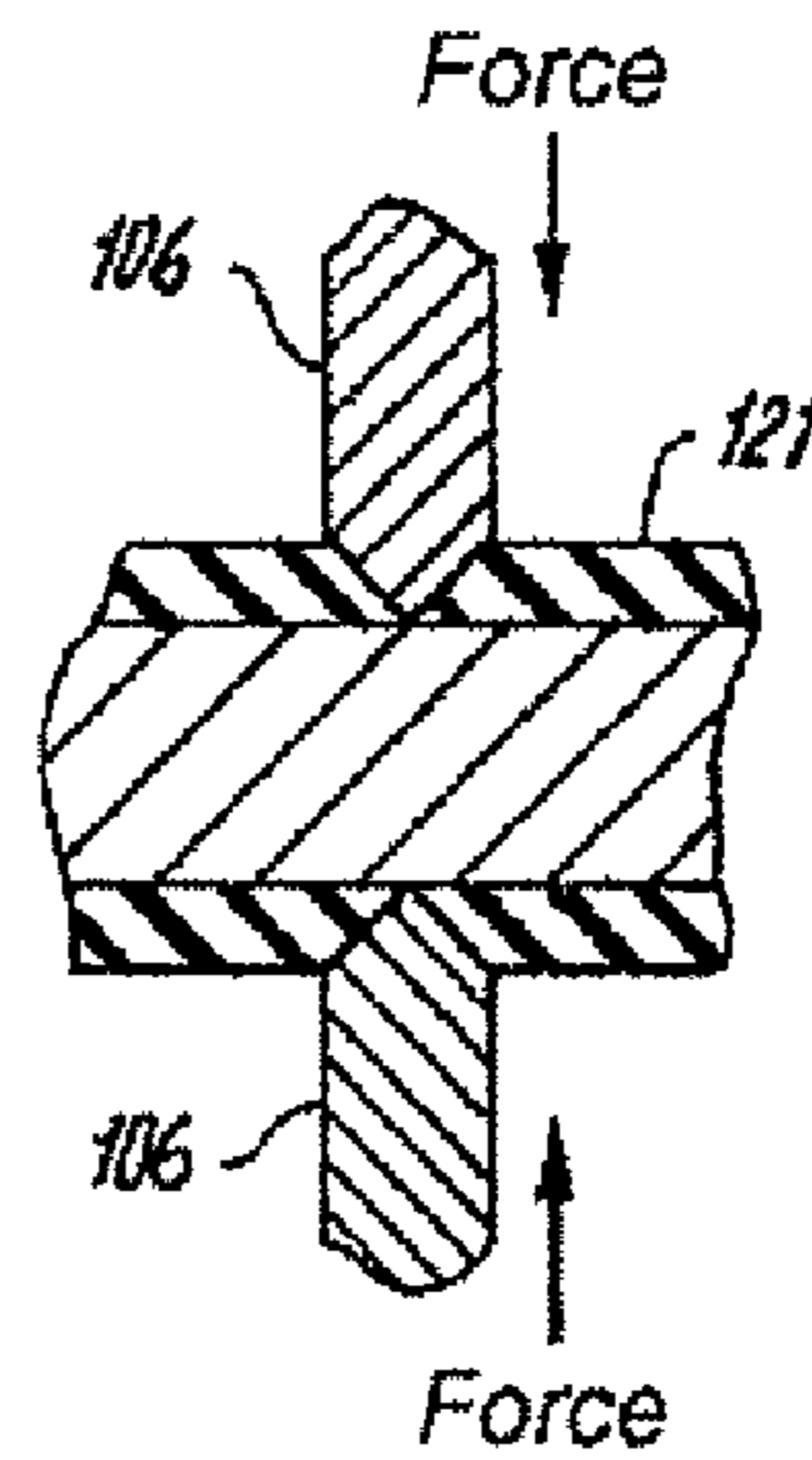
Fig. 3 (Prior Art)
