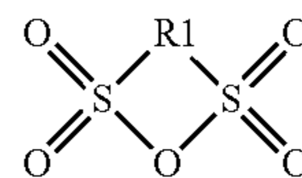
5 [Chemical formula 1]
