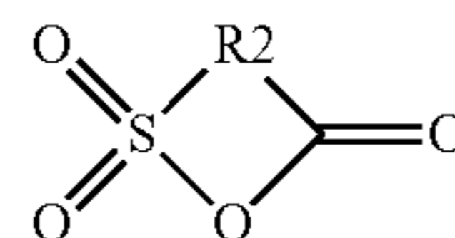
[Chemical formula 2]
