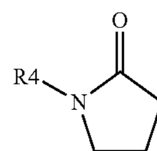
40 [Chemical formula 4]
