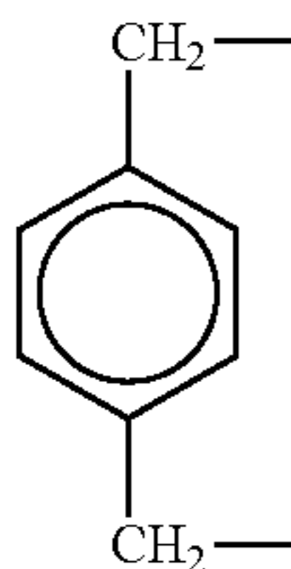
[Chemical formula 23]
