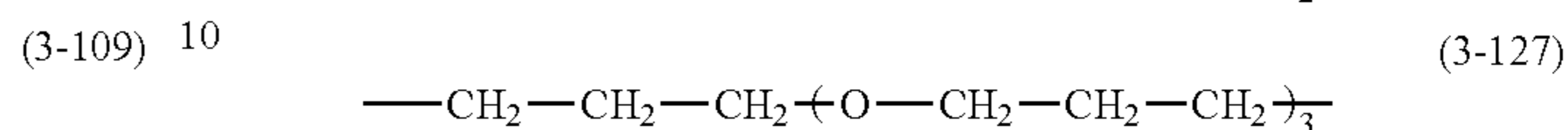
[Chemical formula 24]
