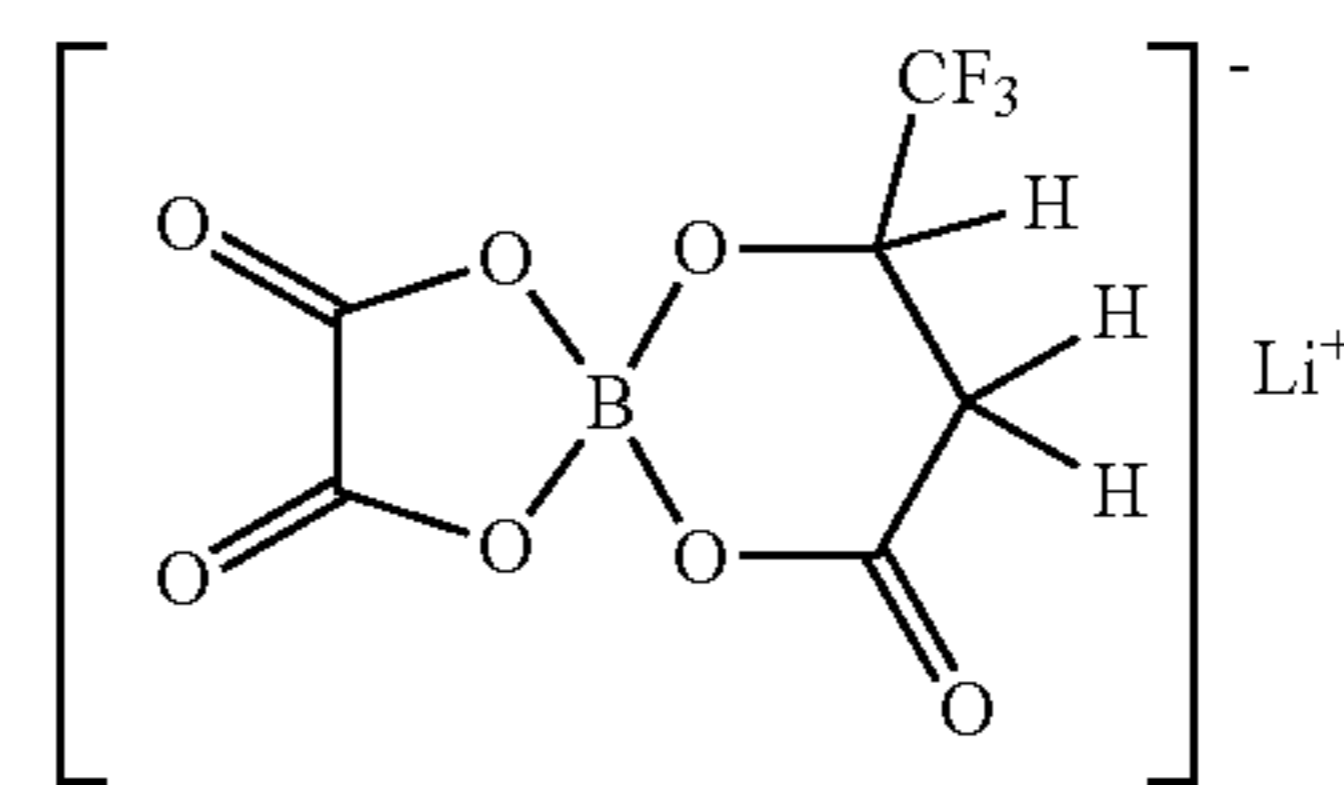
[Chemical formula 13-1]
