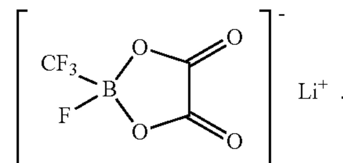
[Chemical formula 13-1]
