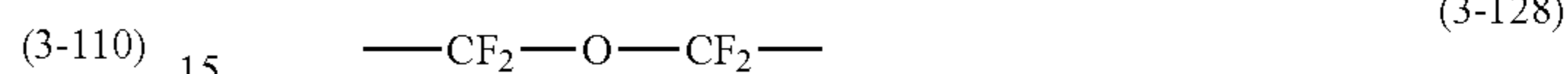
[Chemical formula 24]
