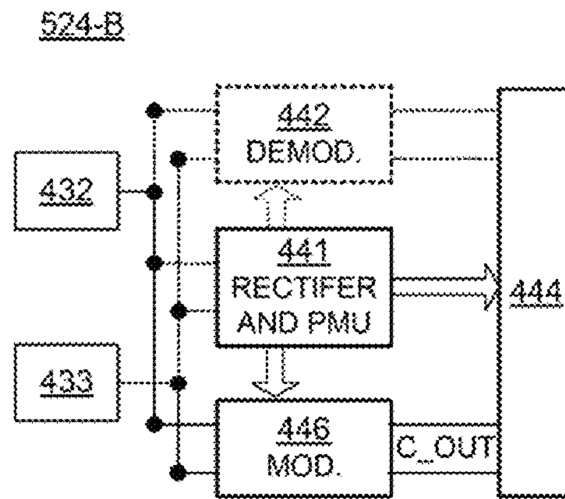
SIGNAL PATH DURING T → R
