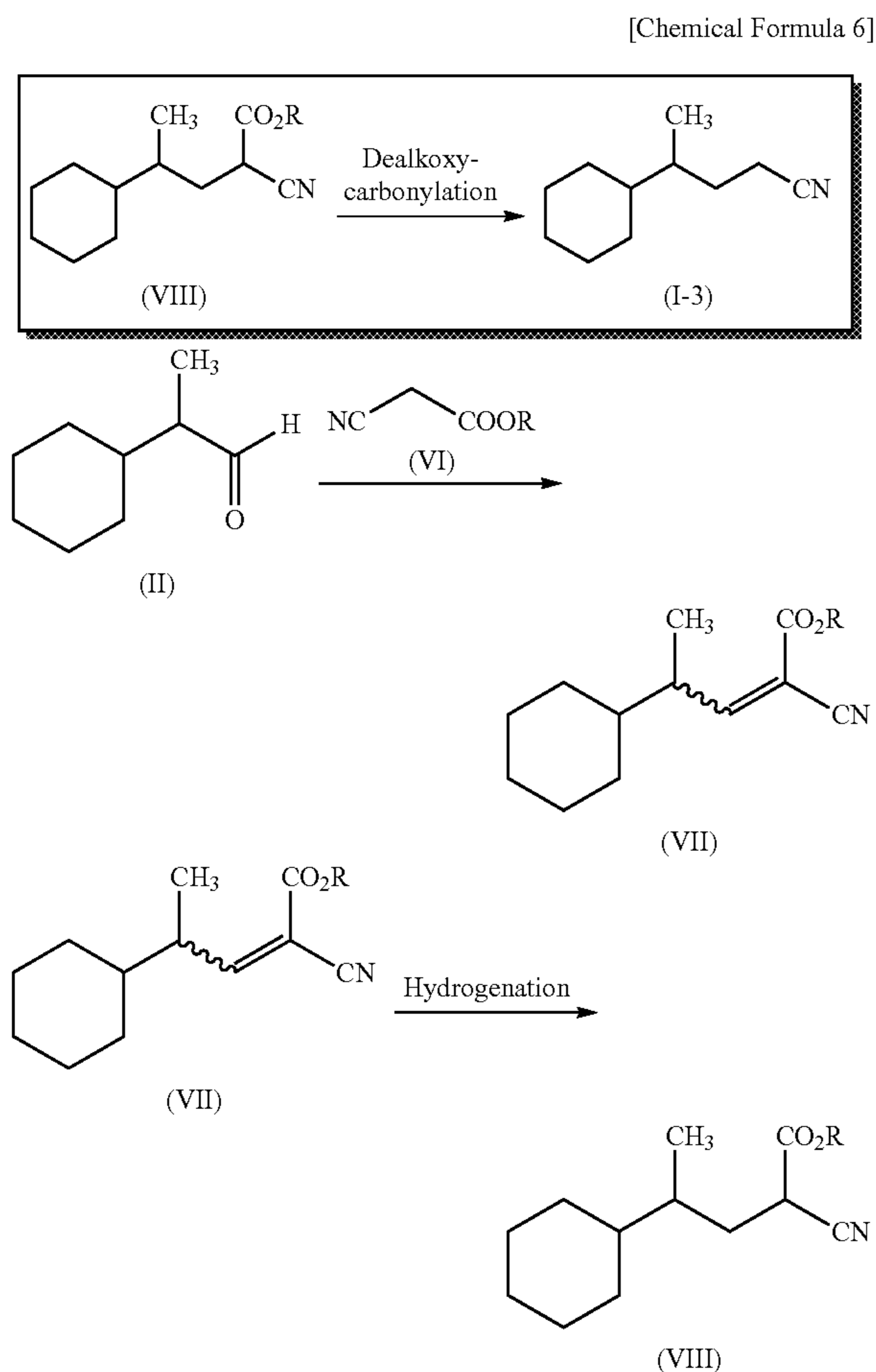
Scheme 2
