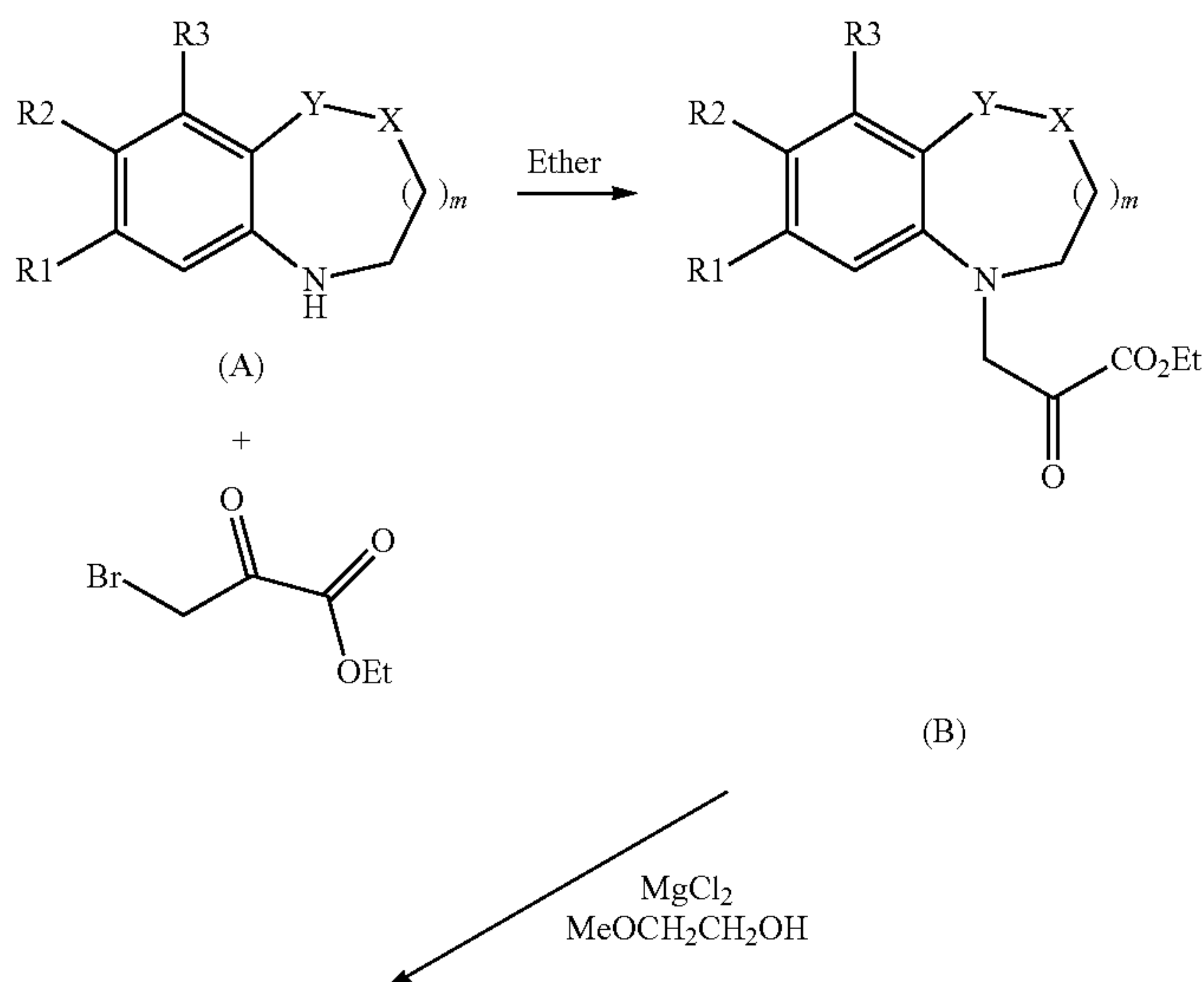
Scheme 3. Preparation of Compounds of Formula (I) where Y is a bond
