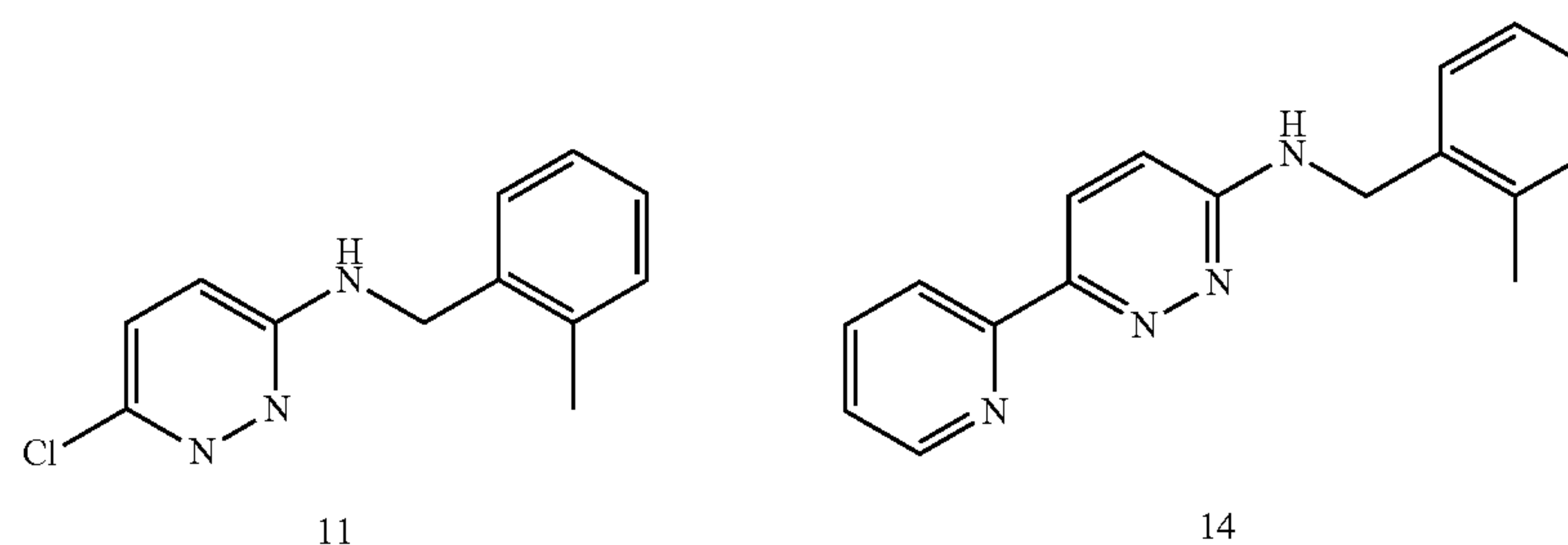
Scheme 2.
