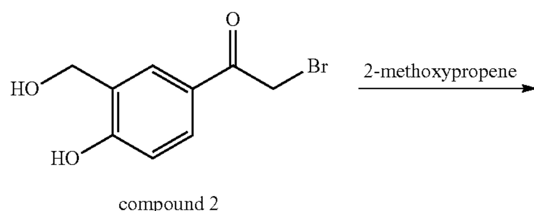
Reaction Scheme 1: a synthesis route of an embodiment of preparing intermediate Compound 1 of salmeterol
