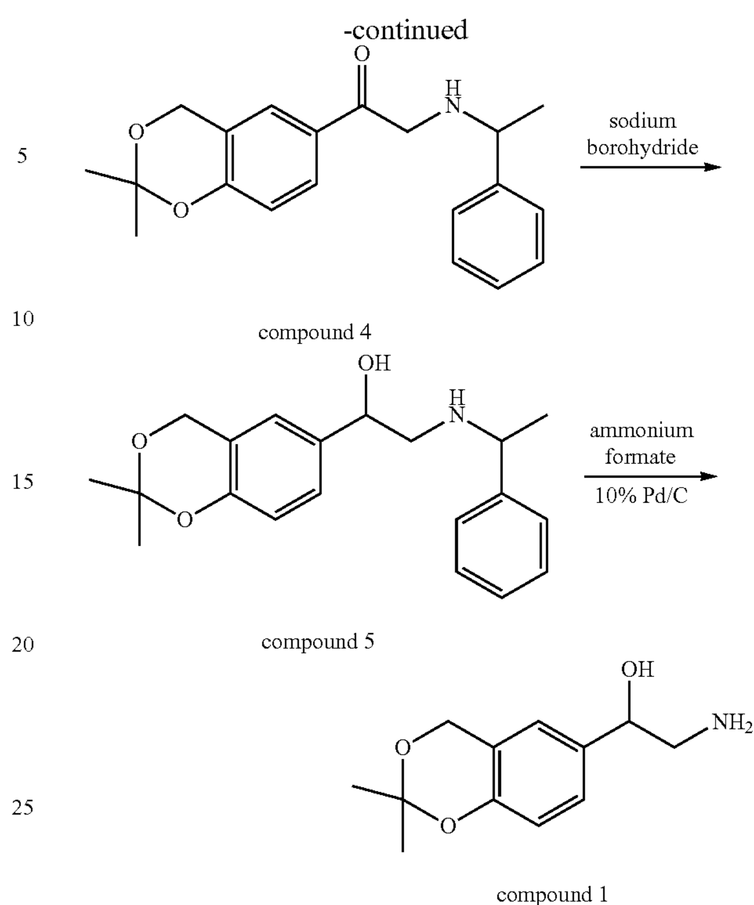
compound 1
