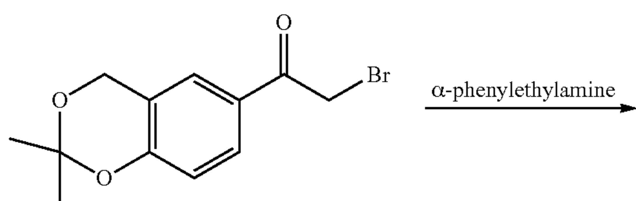
compound 3
