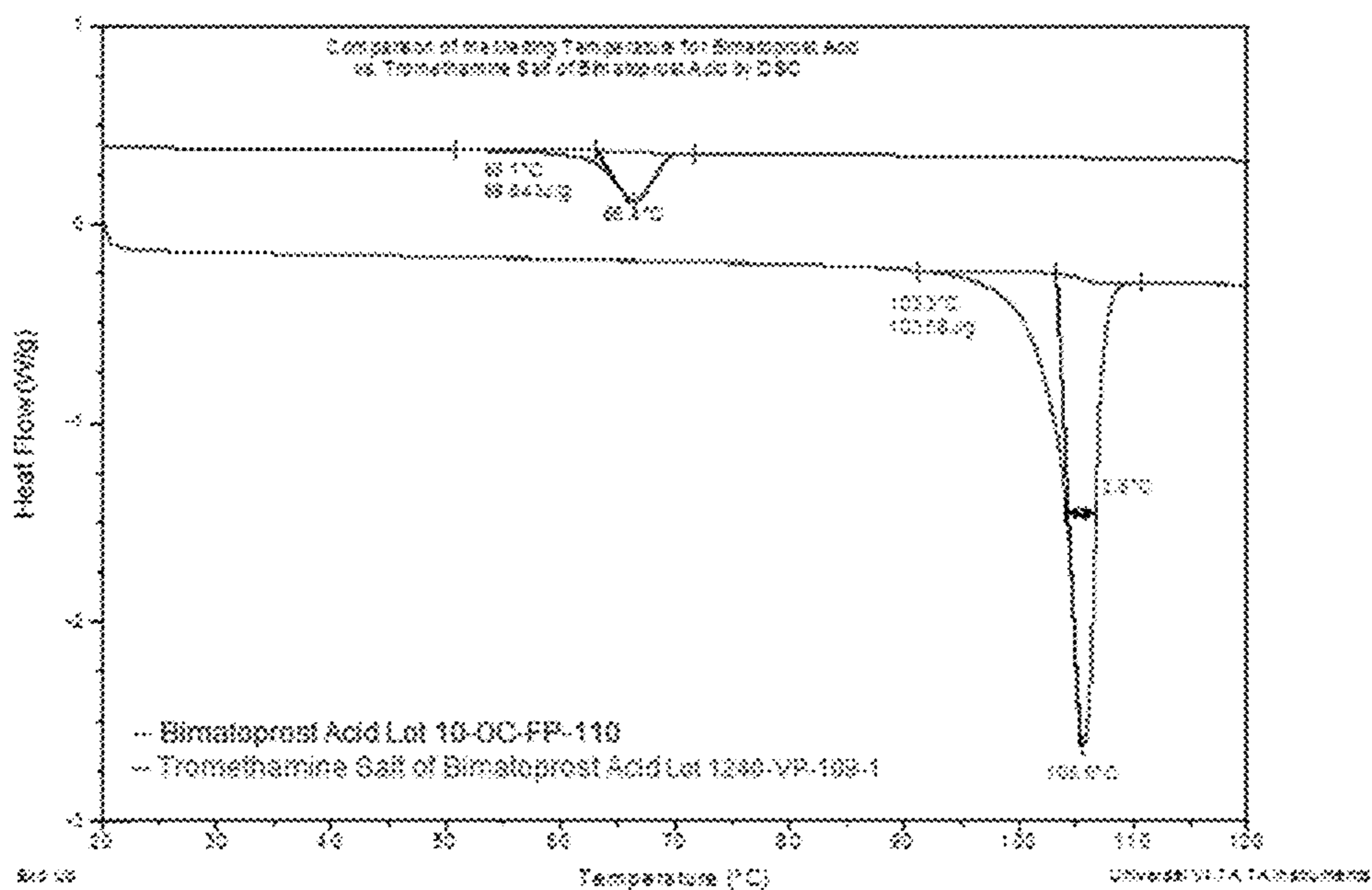
Figure 1: DSC data for Bimatoprost Acid (crystalline anhydrous) compared to the Tromethamine Salt of Bimatoprost Acid (crystalline Form 1) that is indicating a melting temperature for the salt at about ~40°C higher than melting temperature of the free acid.
