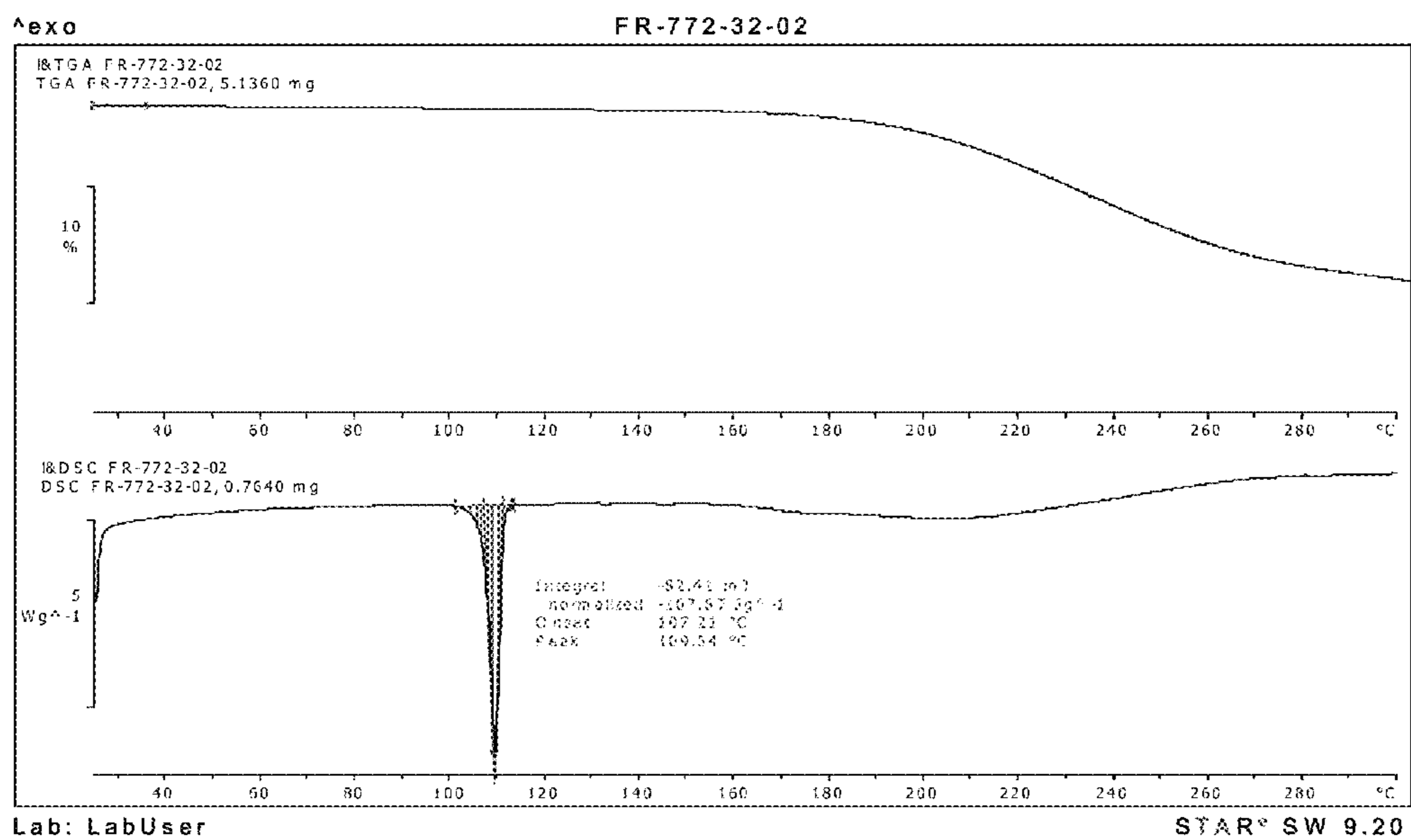
Figure 2: DSC/TGA analyses of Tromethamine Salt of Bimatoprost Acid (Form 1)
