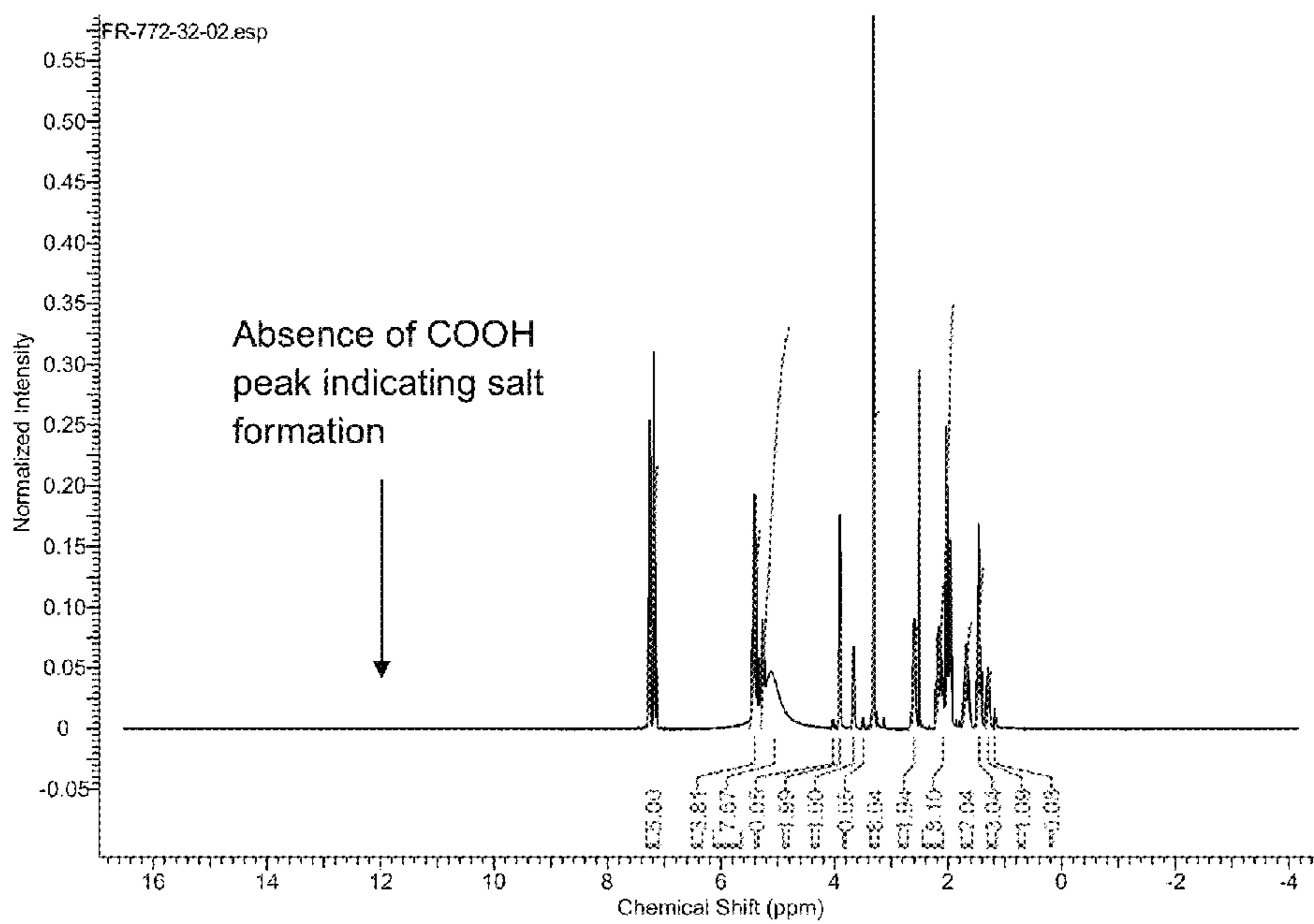
Figure 4: 1 H-NMR of Tromethamine Salt of Bimatoprost Acid (Form 1 dissolved in DMSO). The absence of 1 H-NMR peak for the -COOH proton at about 12 ppm indicates formation of the salt.
