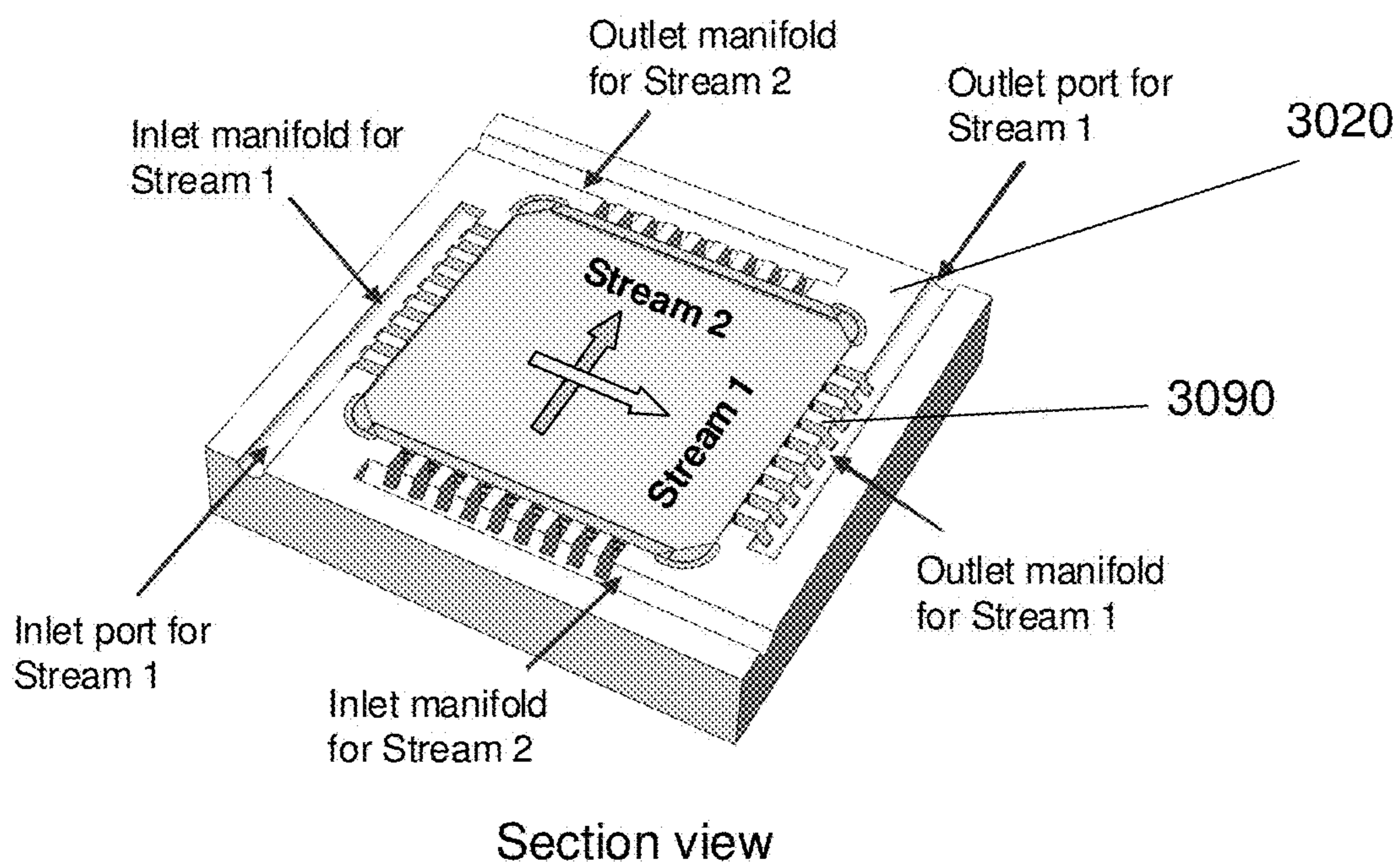
Section view FIG. 30
