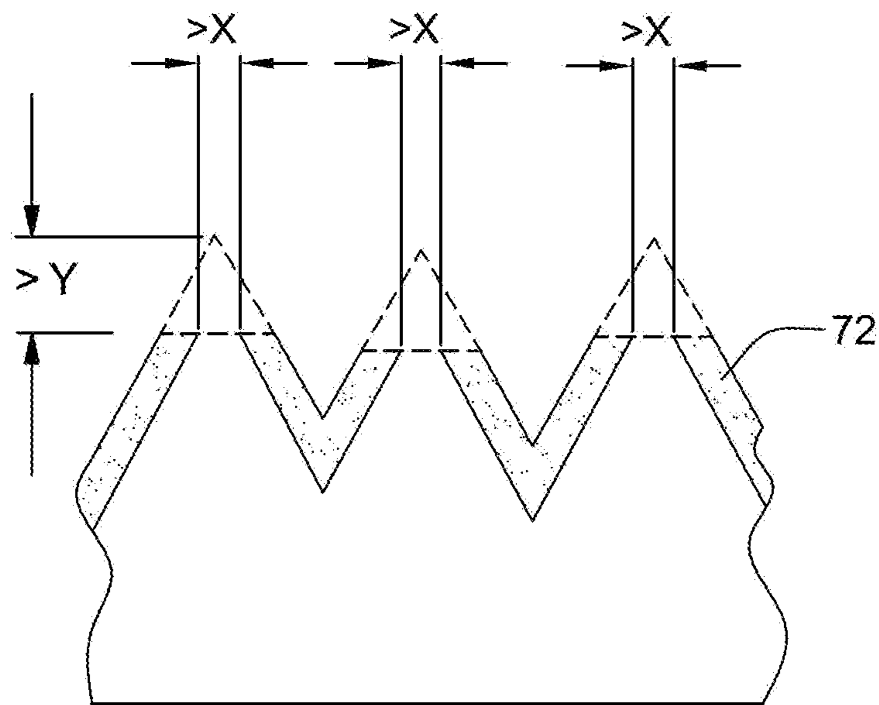
RF BIAS FIG. 7b
