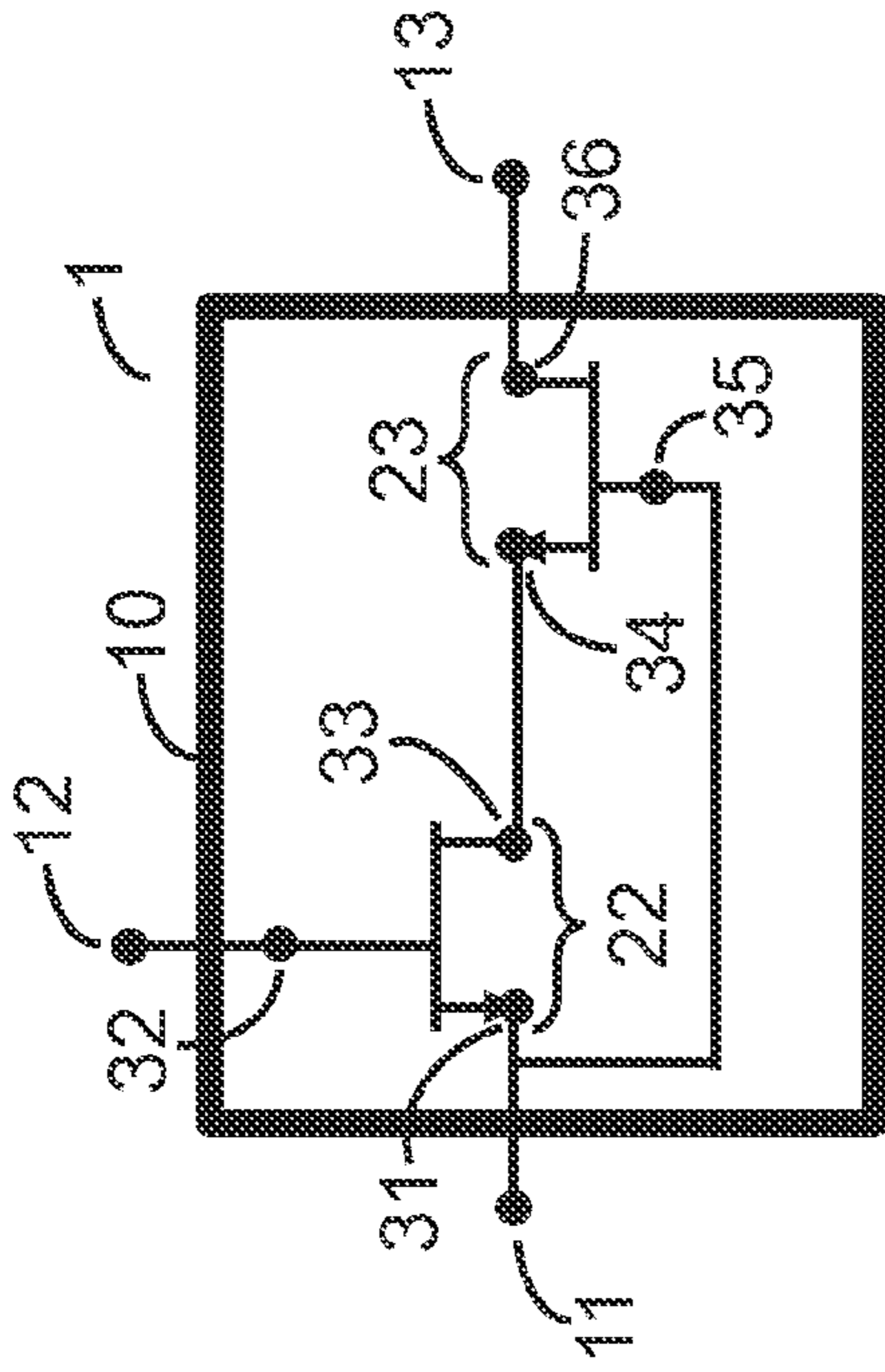
Figure 1 (prior art)
