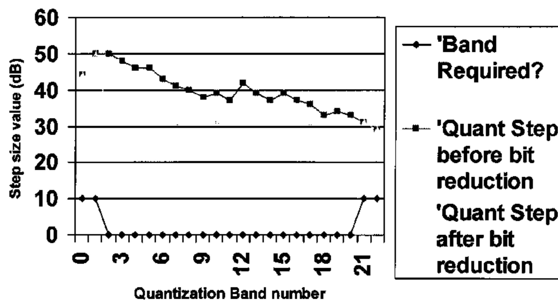
1200 → Quantizer step size modification to reduce bits
