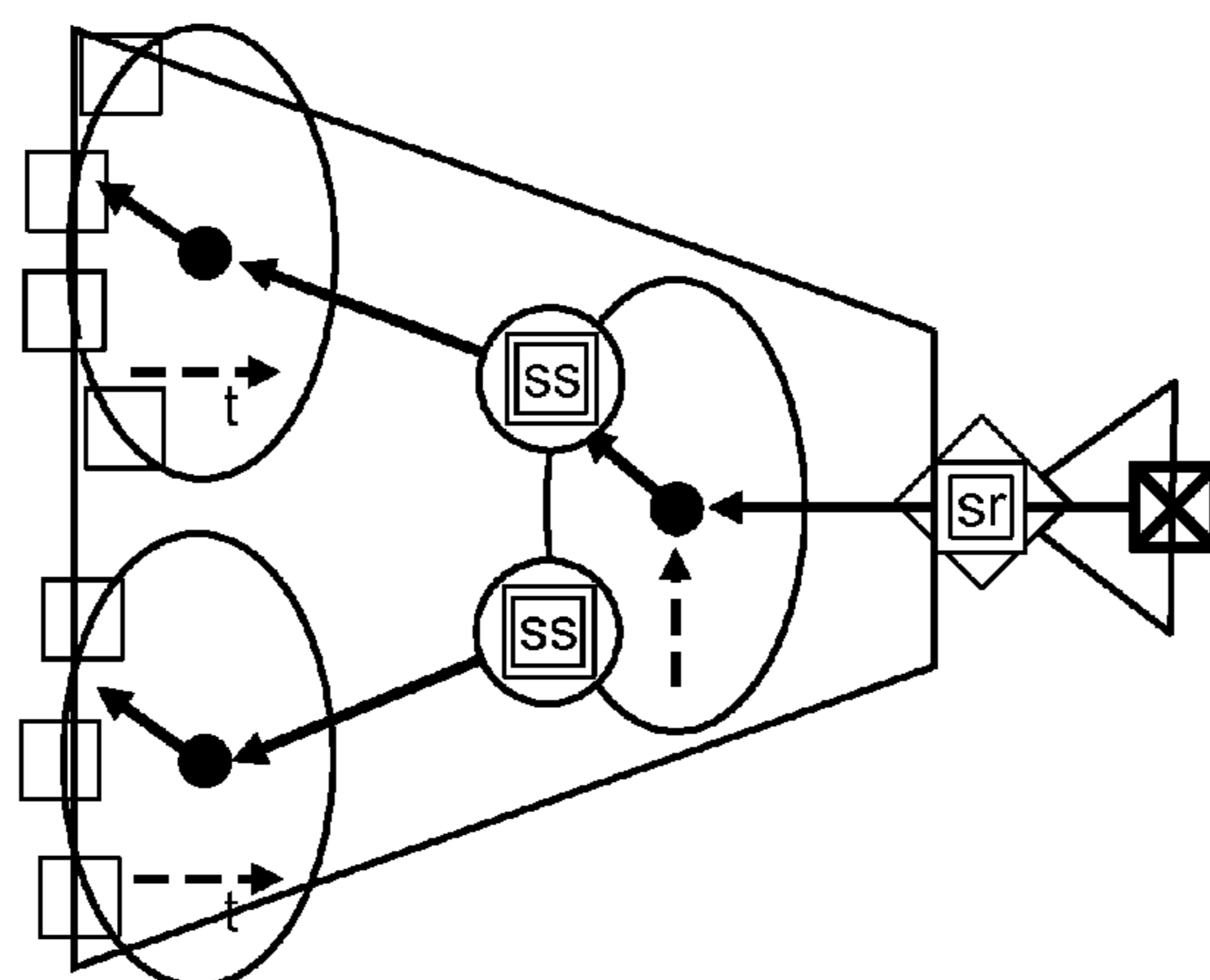
Figure 11: Example single Processing Resource Instance scheduling hierarchy
