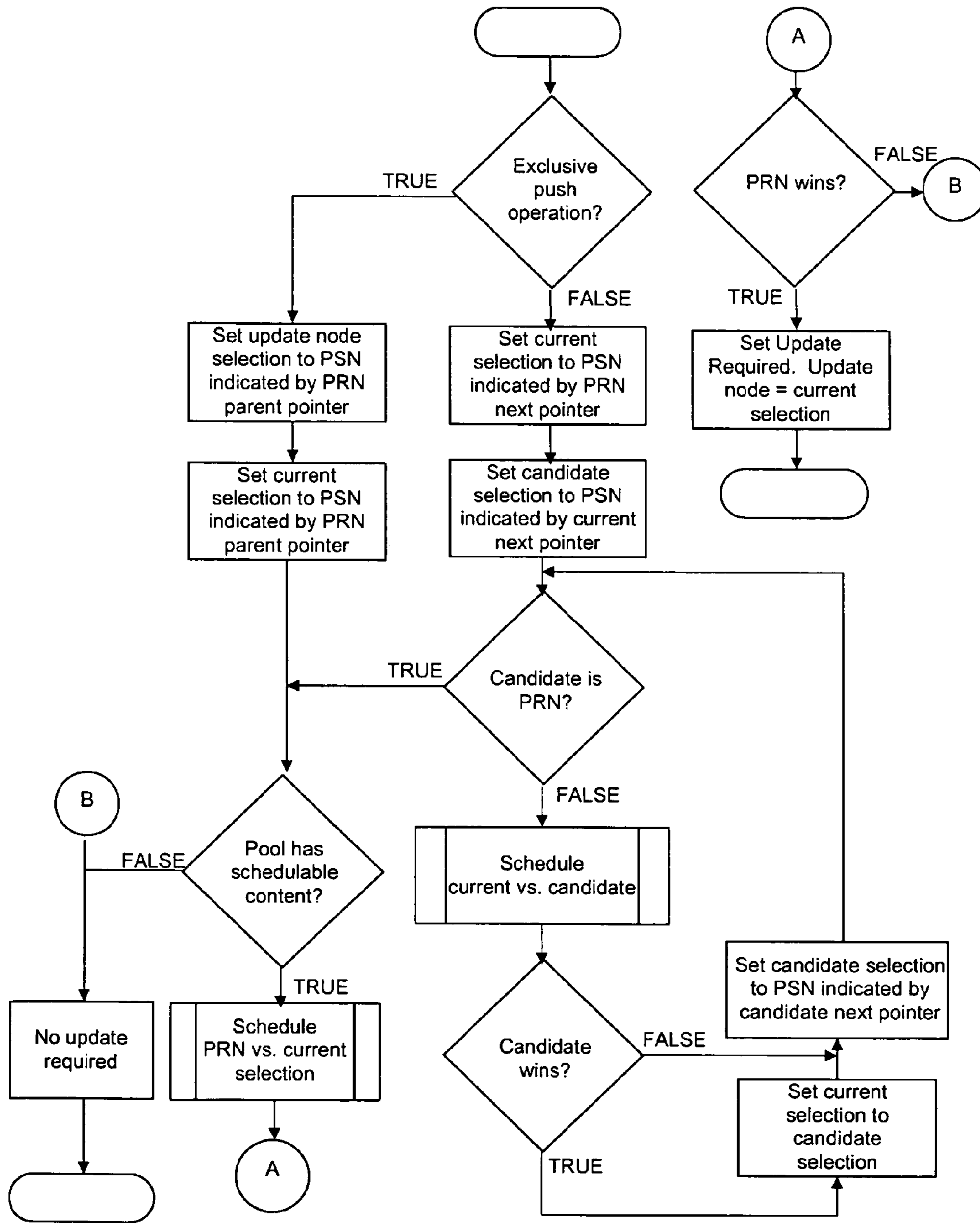
Figure 67: Intra-pool tier scheduler processing
