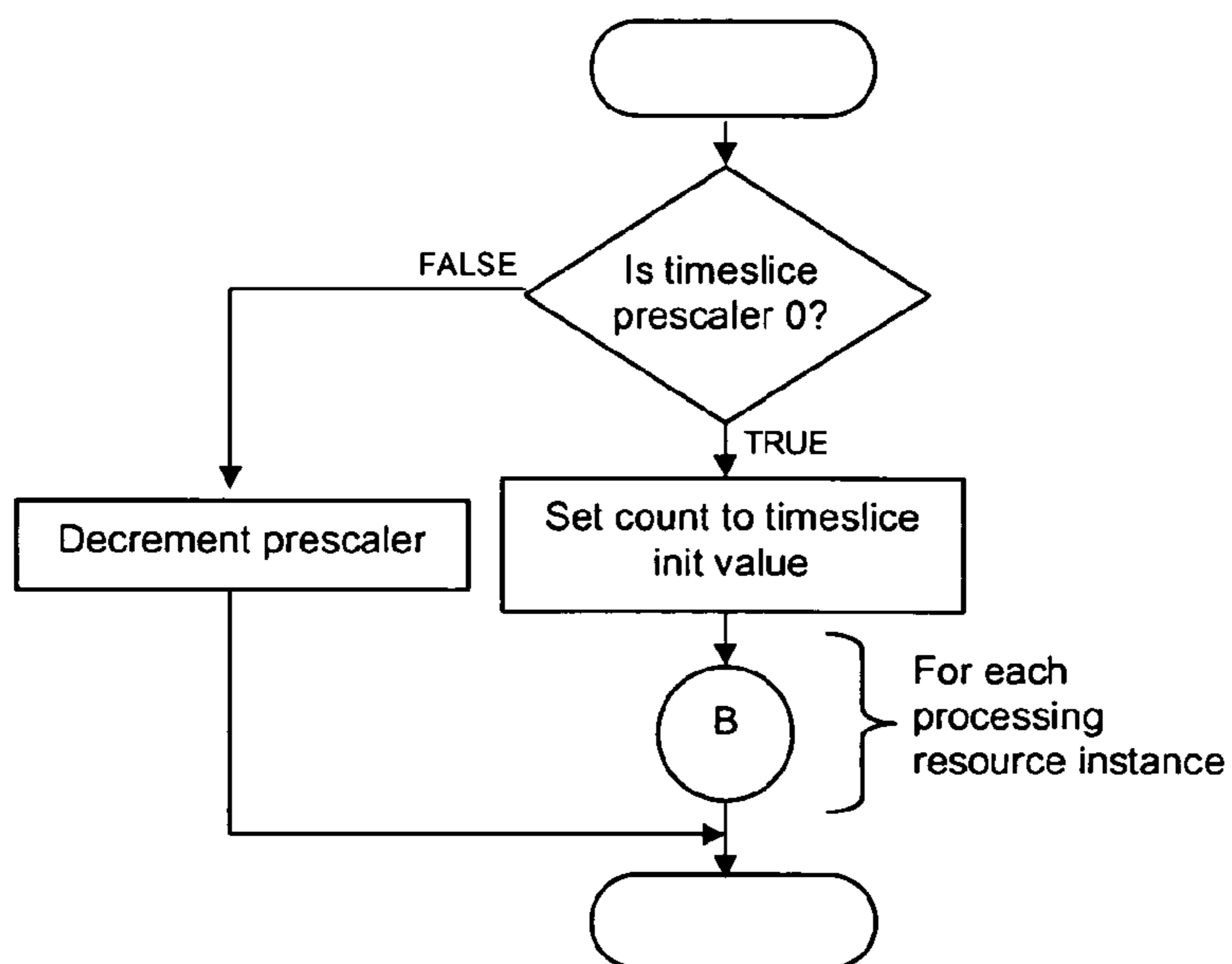
Figure 45: Timeslice control
