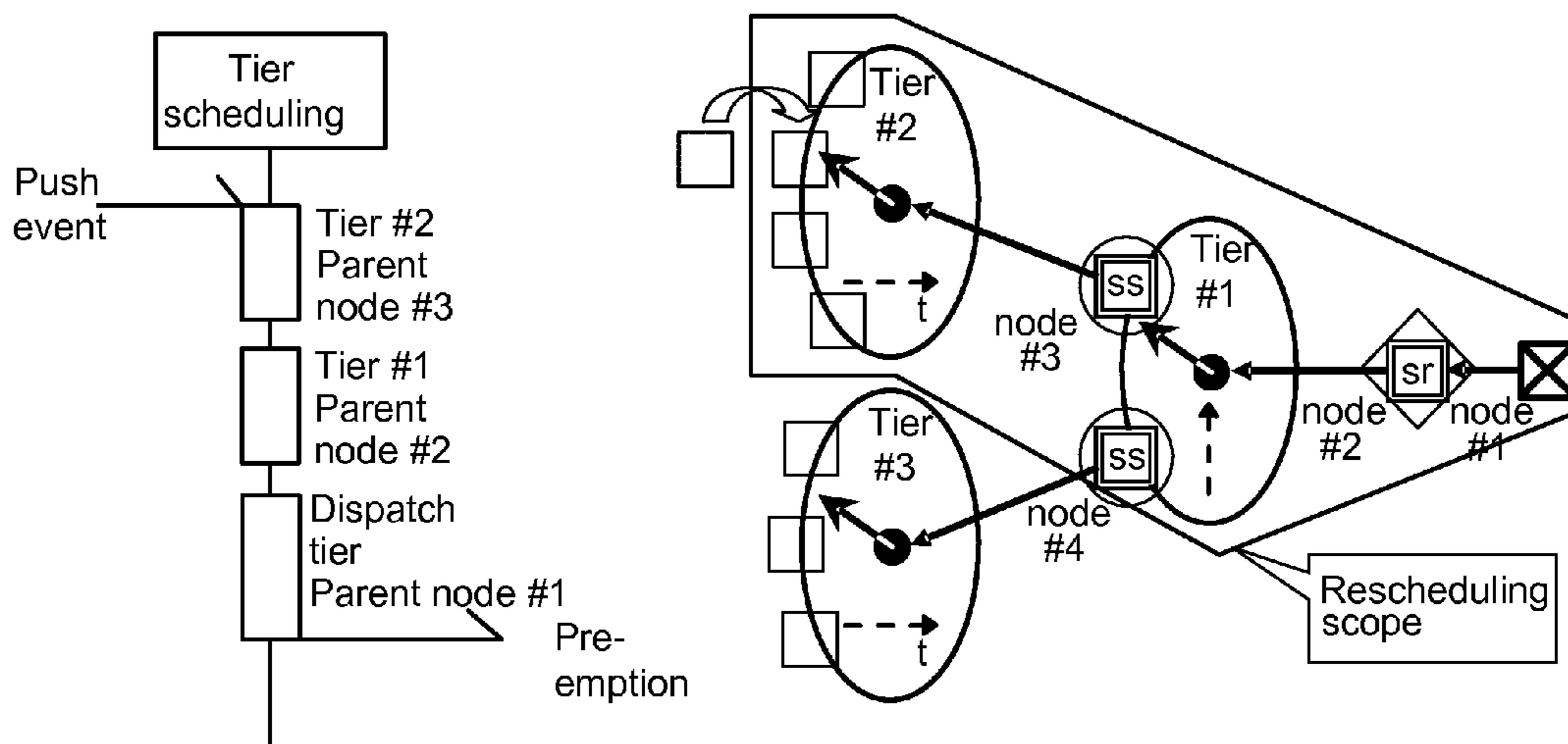
Figure 19: Rescheduling scope for a simple push operation
