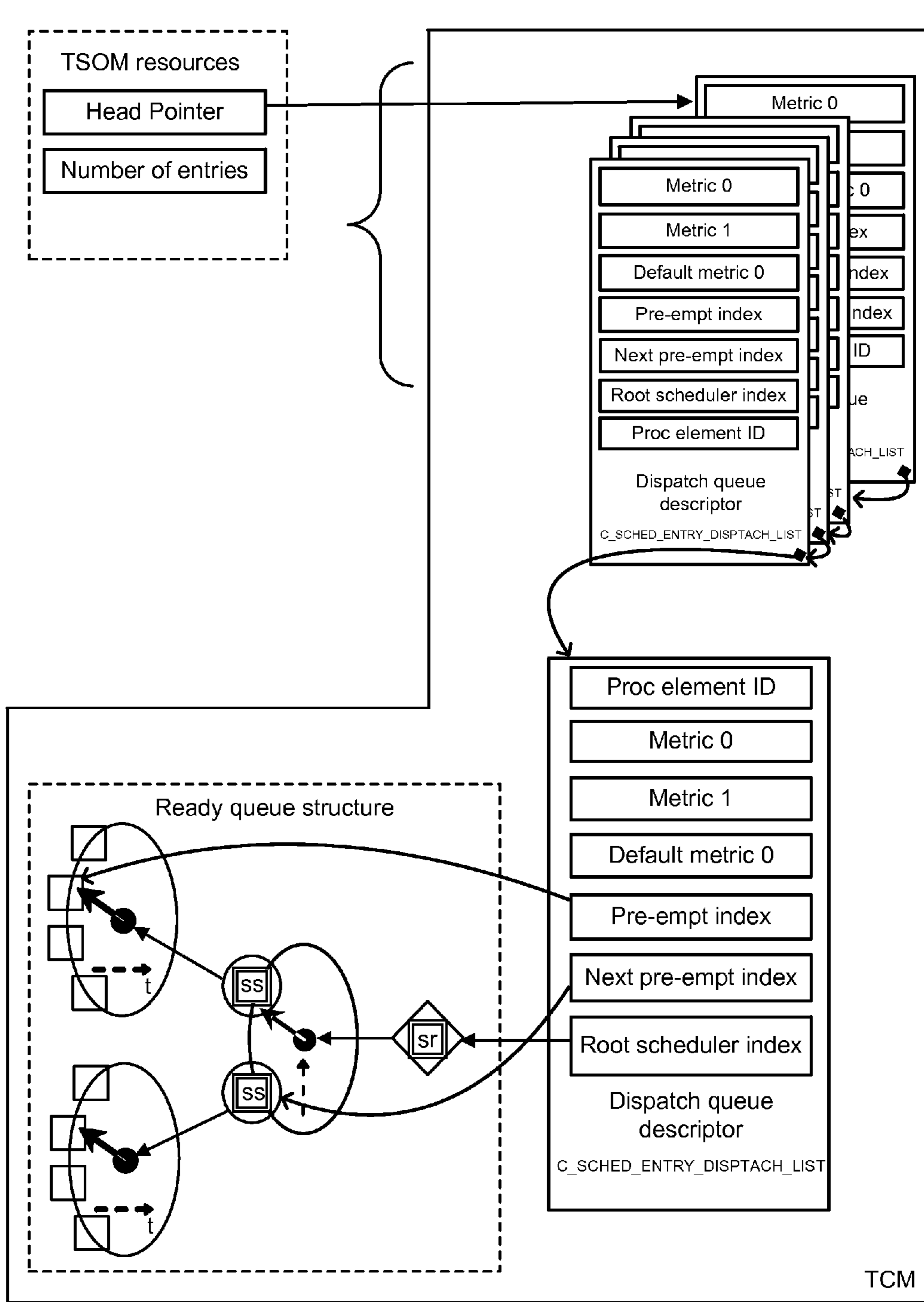
Figure 58: TSOM internal architecture
