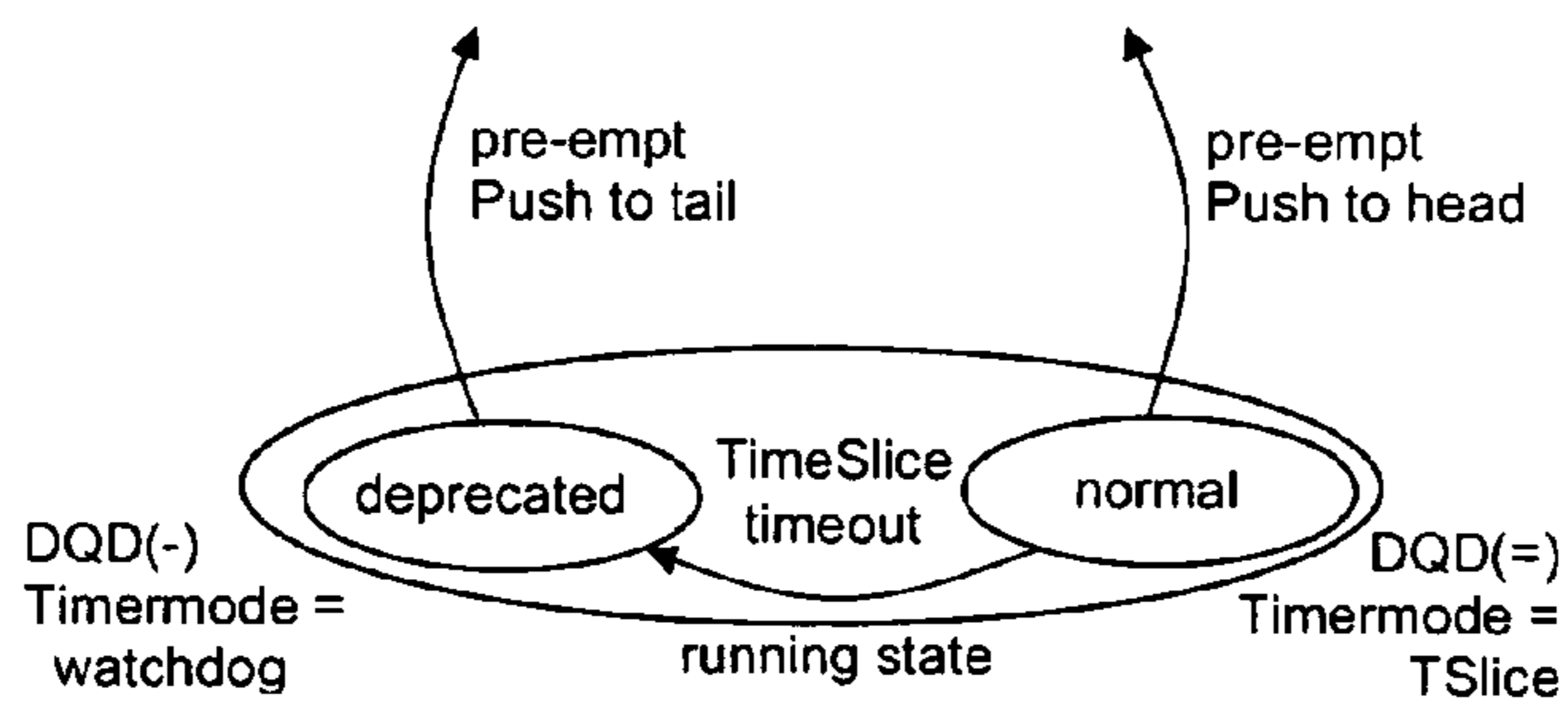
Figure 24: Task priority delta diagram
