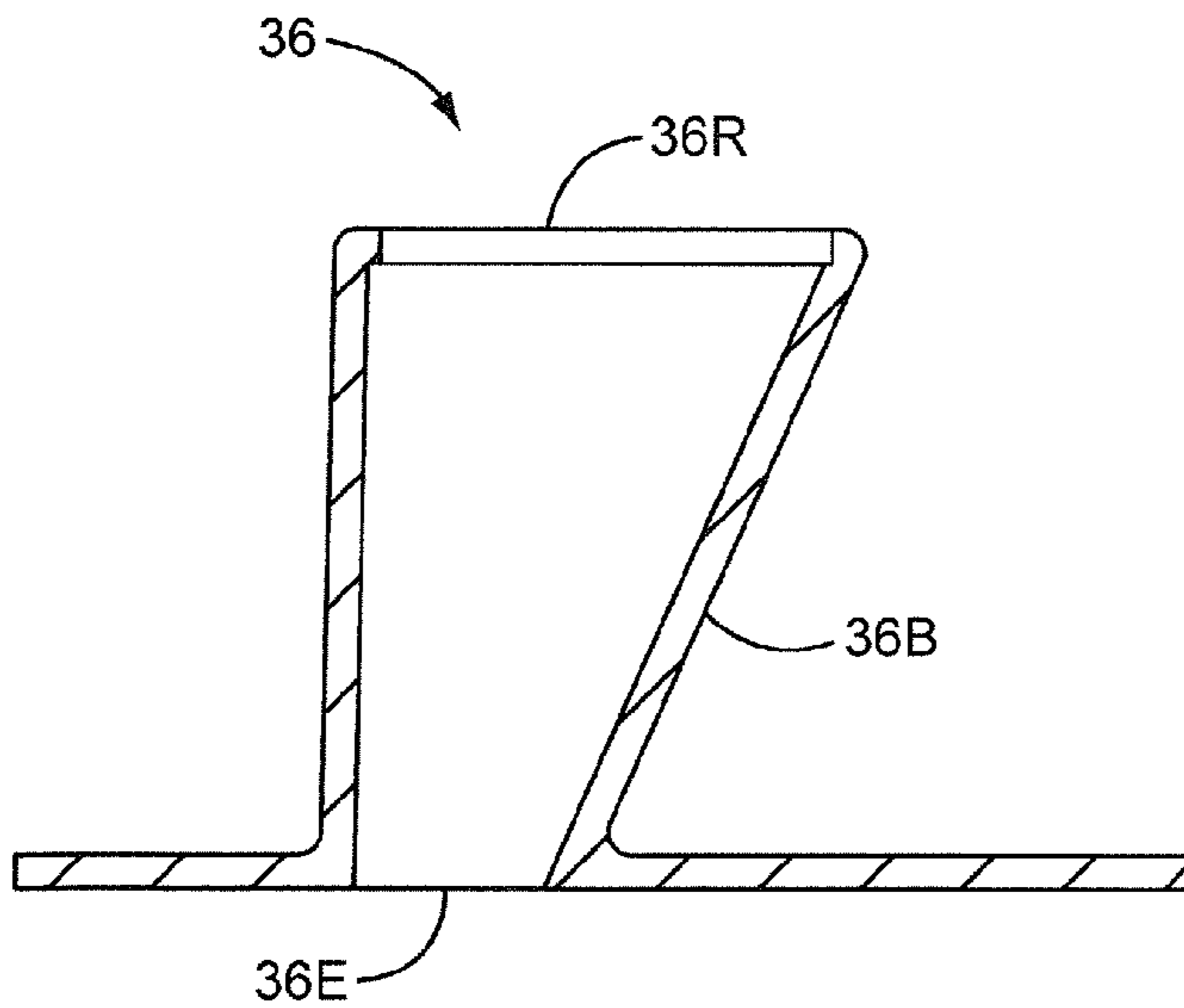
FIG. 12J SECTION F-F
