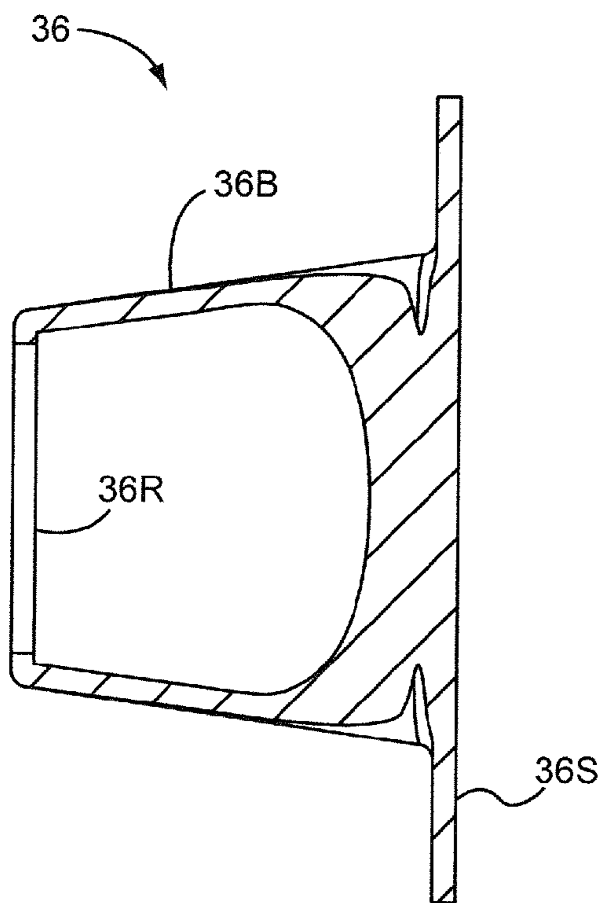
FIG. 12G SECTION C-C
