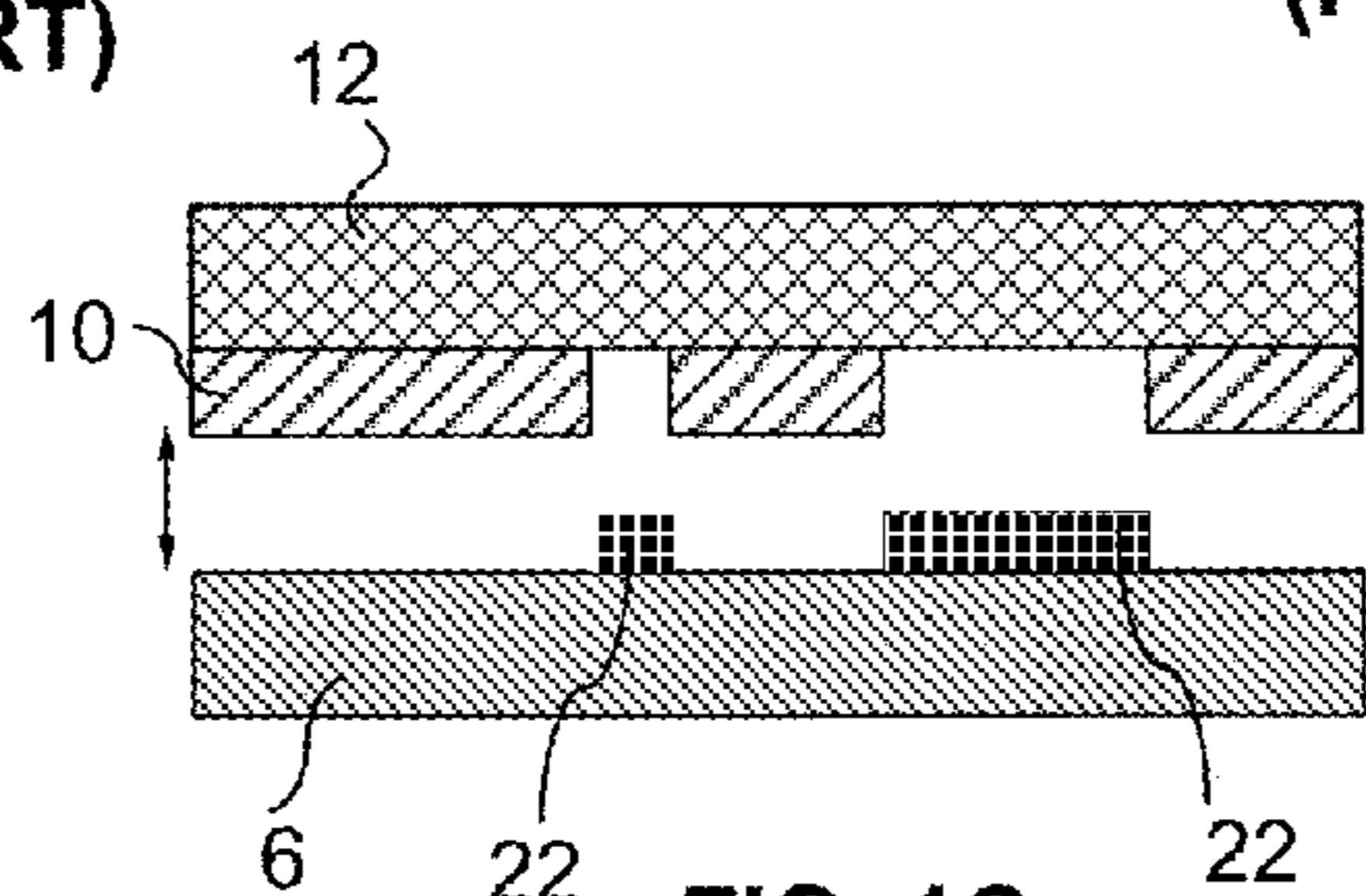
FIG. 1C (PRIOR ART)
