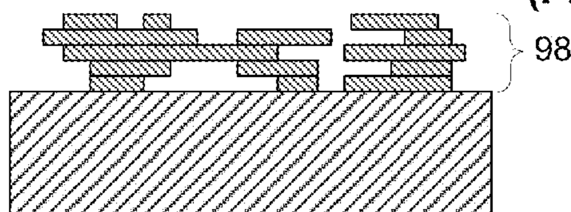
FIG. 4I (PRIOR ART)
