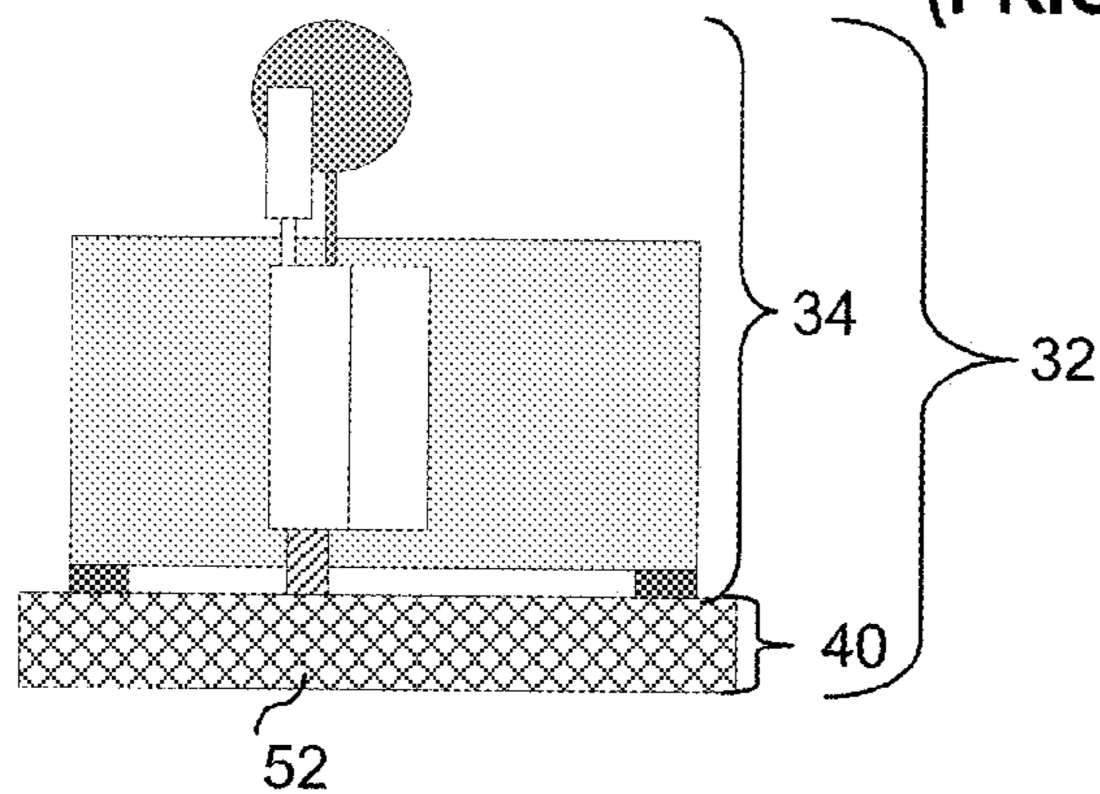
FIG. 3C (PRIOR ART)
