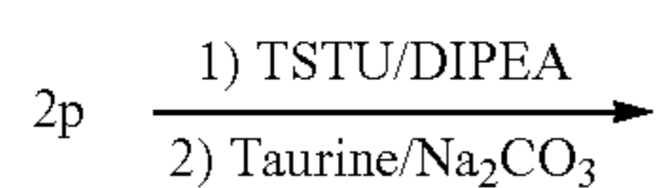
Scheme 4: Synthesis of taurine amide indolenine cyanine dyes
