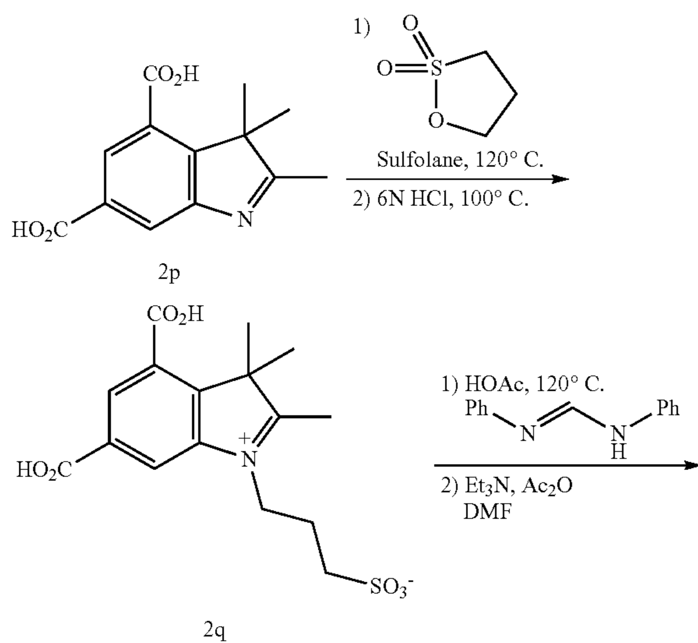
Scheme 3: Synthesis of carboxyl indolenine cyanine dyes
