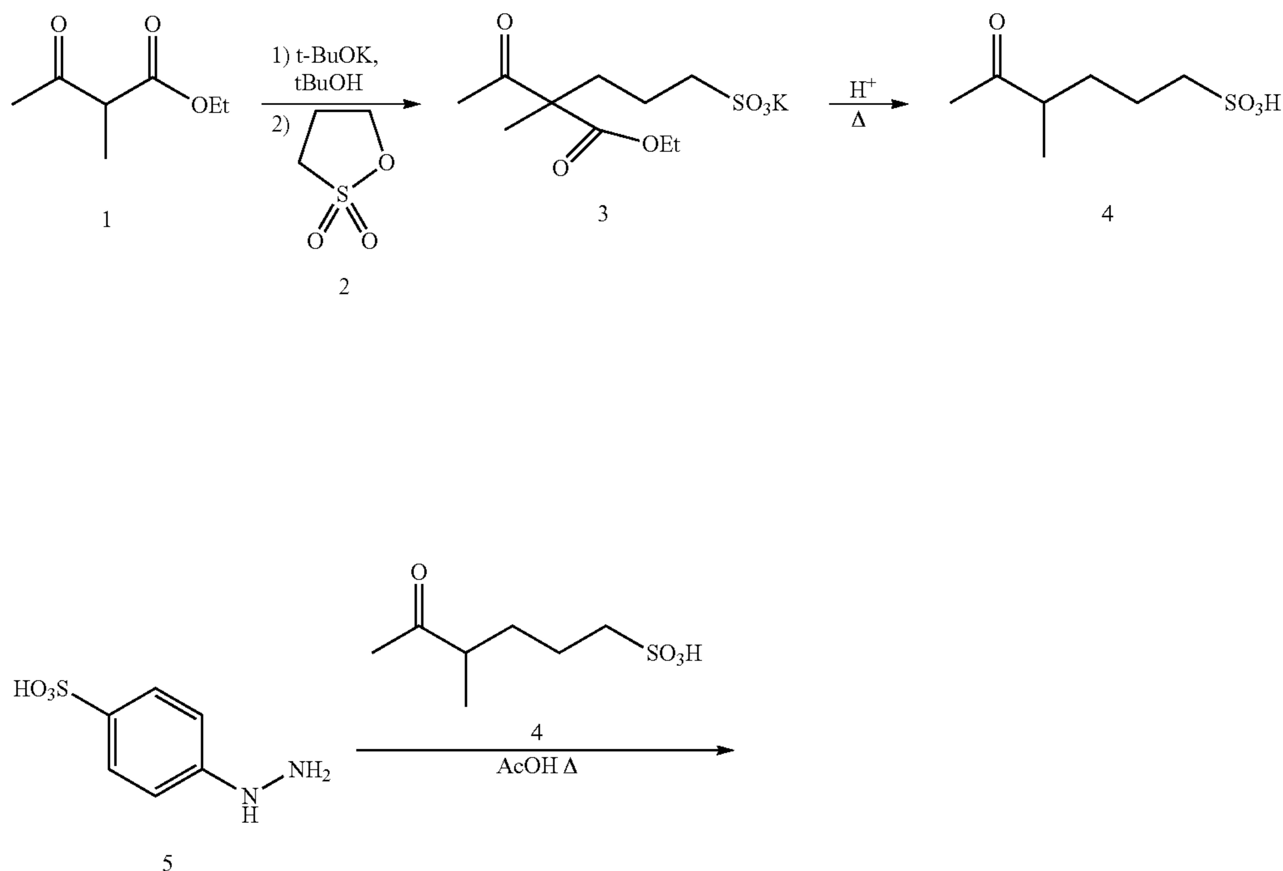
Scheme 1. Synthesis of Pentasulfonated Cyanine Dyes
