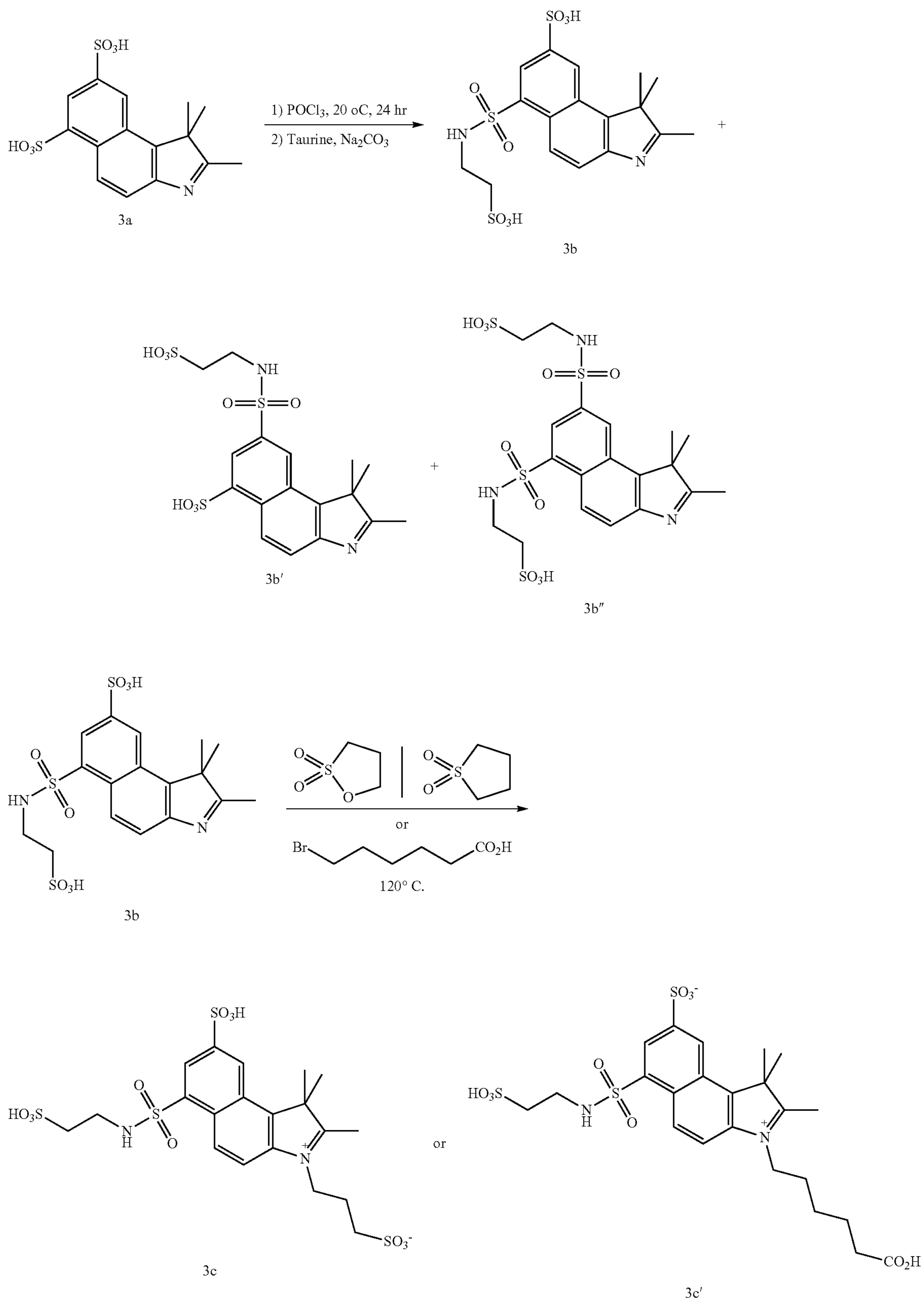
Scheme 5: Synthesis of taurine amide benzindole cyanine dyes
