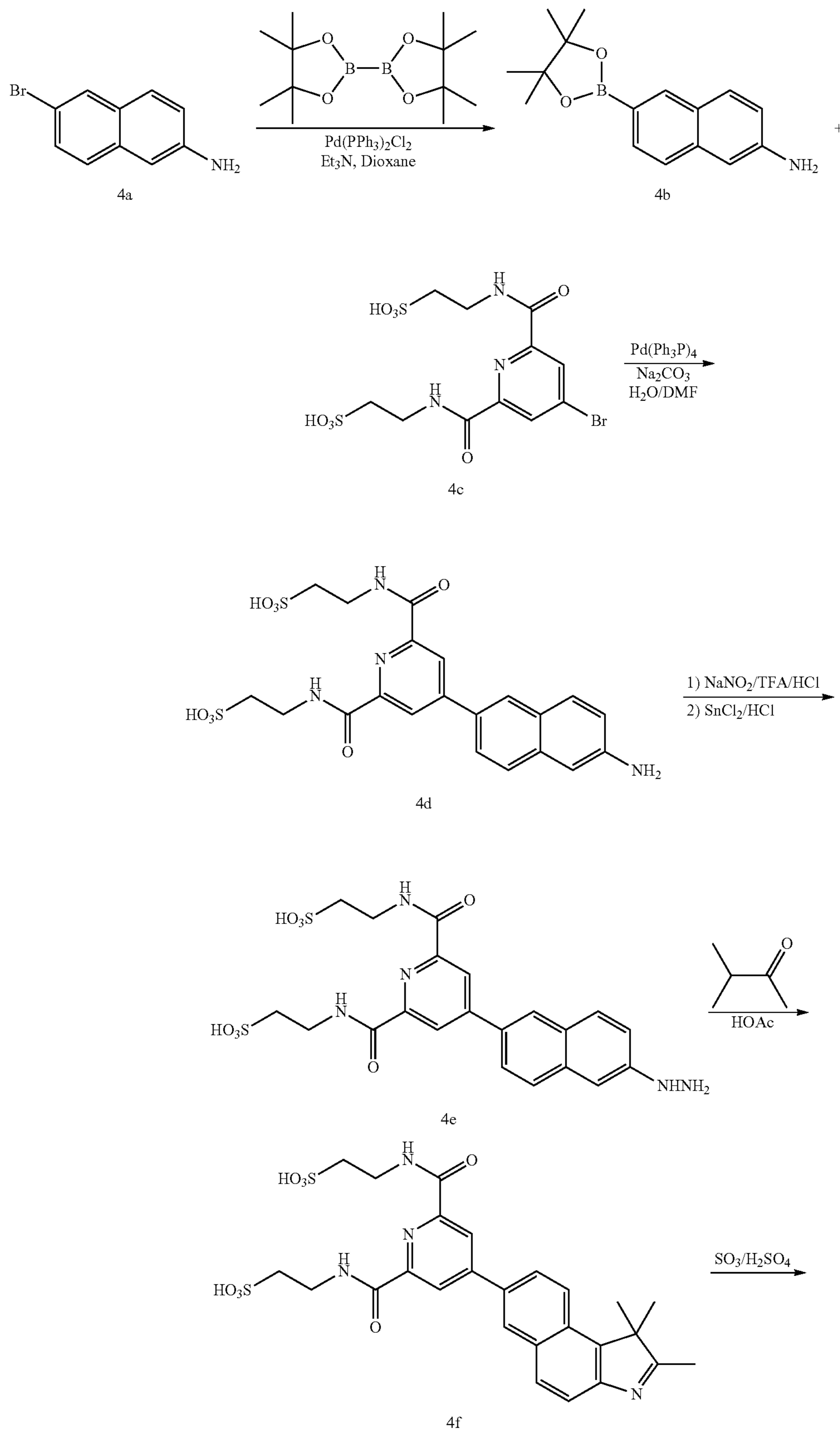
Scheme 6: Synthesis of pyridyl bezindole cyanine dyes
