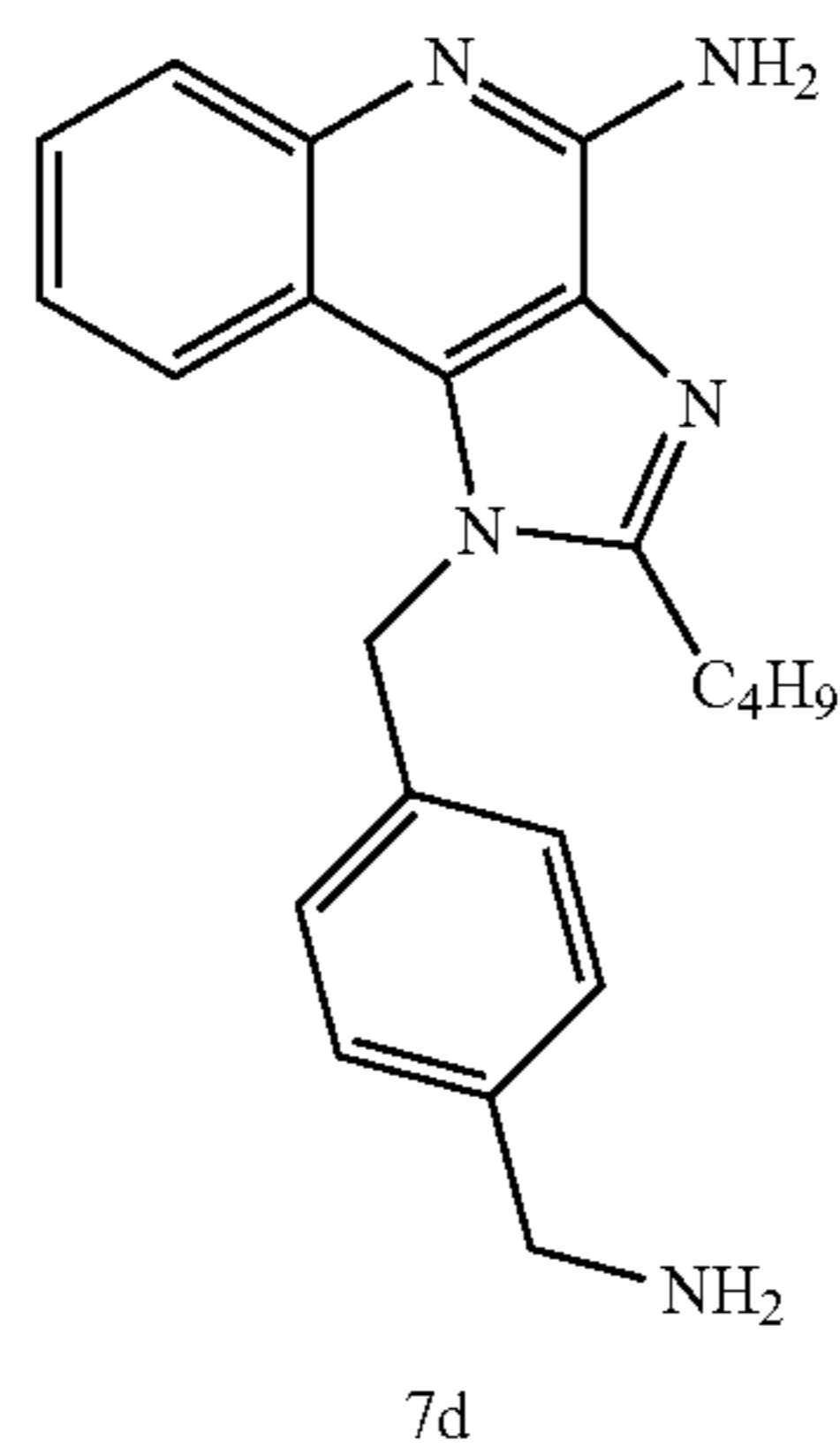
Scheme 4. Syntheses of derivatives of 7d.
