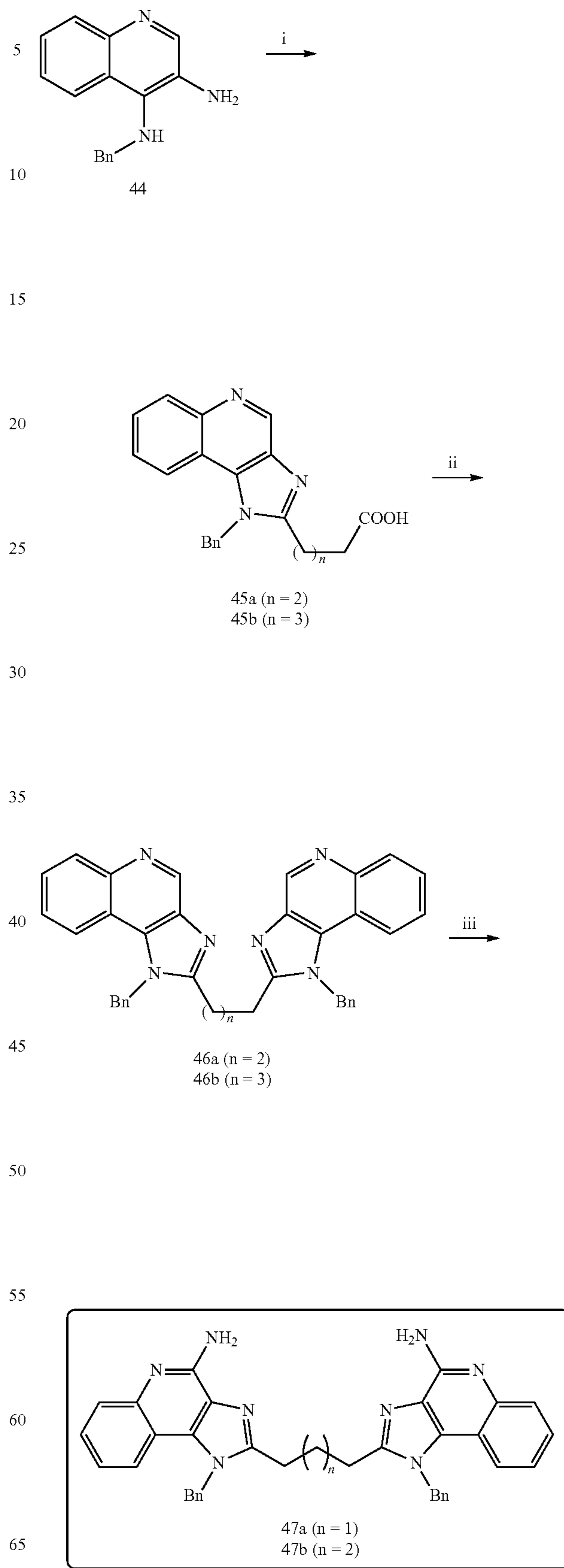
Scheme 15. Syntheses of imidazoquinoline dimers linked at C2.
