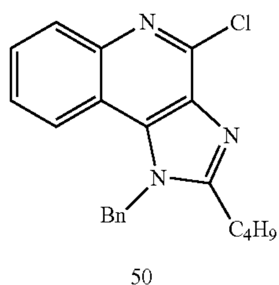
Scheme 16. Syntheses of imidazoquinoline dimers linked at C4—NH 2 .
