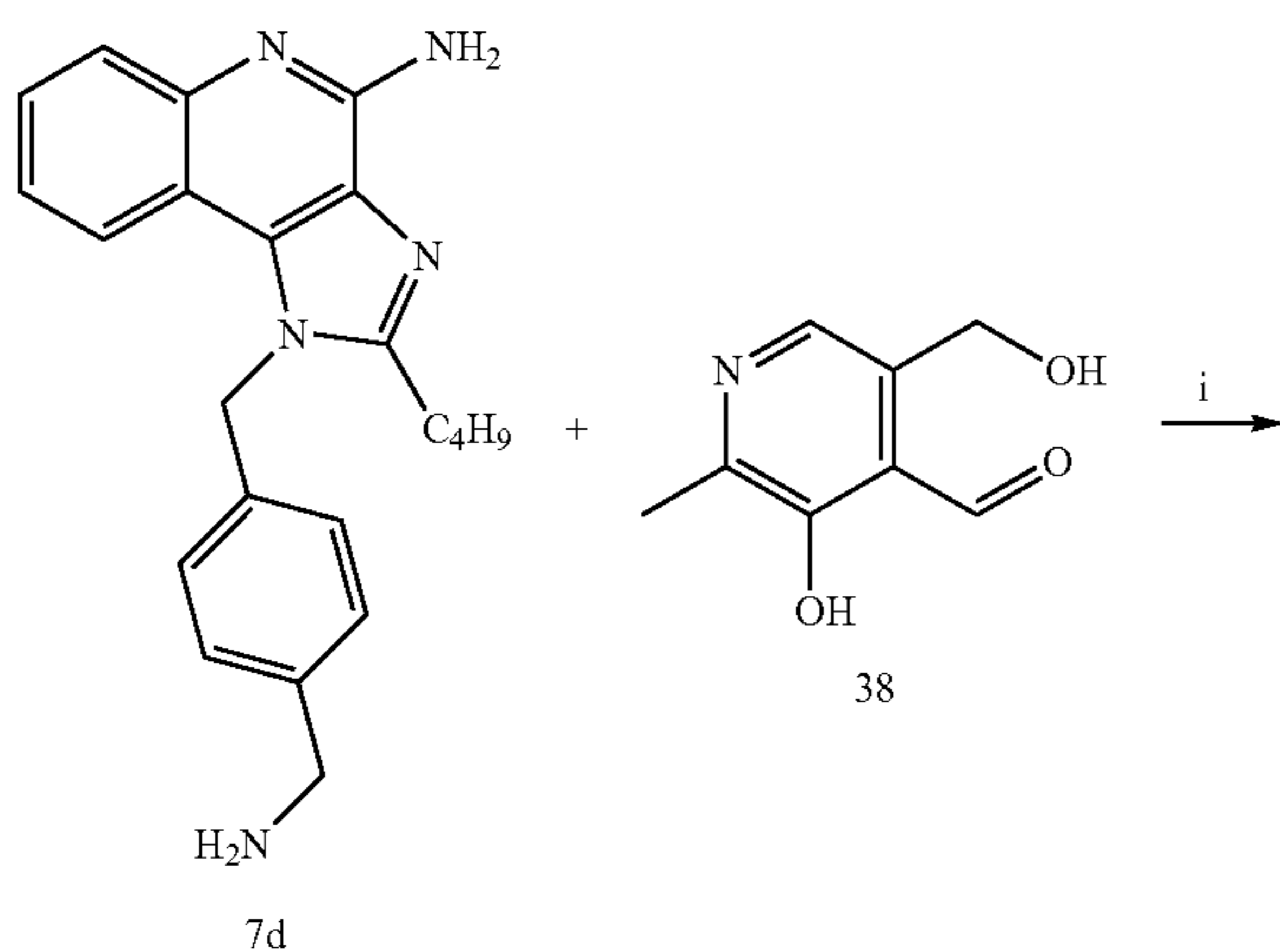
Scheme 12. Synthesis of a pyridoxal derivative 39.
