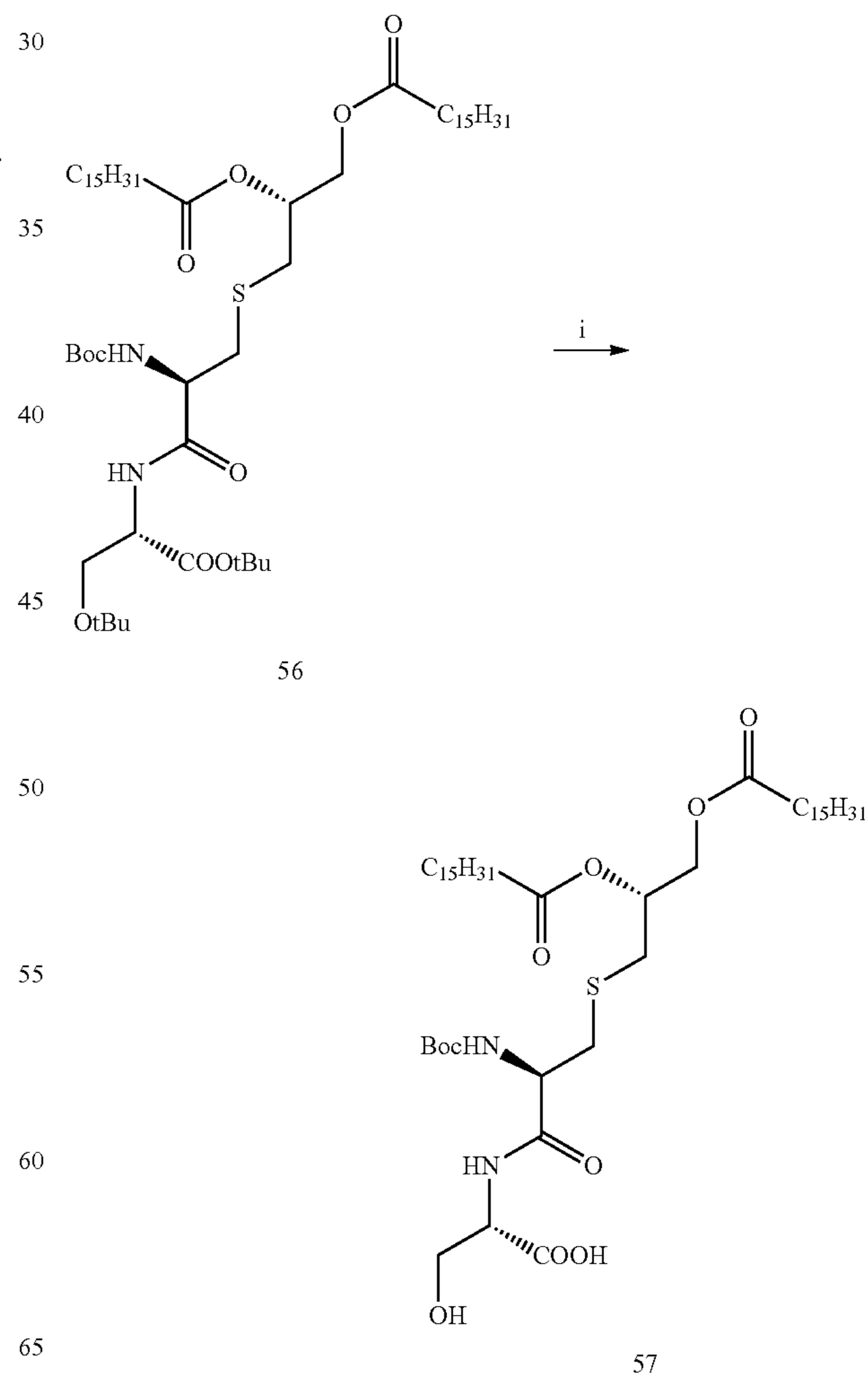
Scheme 19. Syntheses of derivatives of PAM 2 CS.
