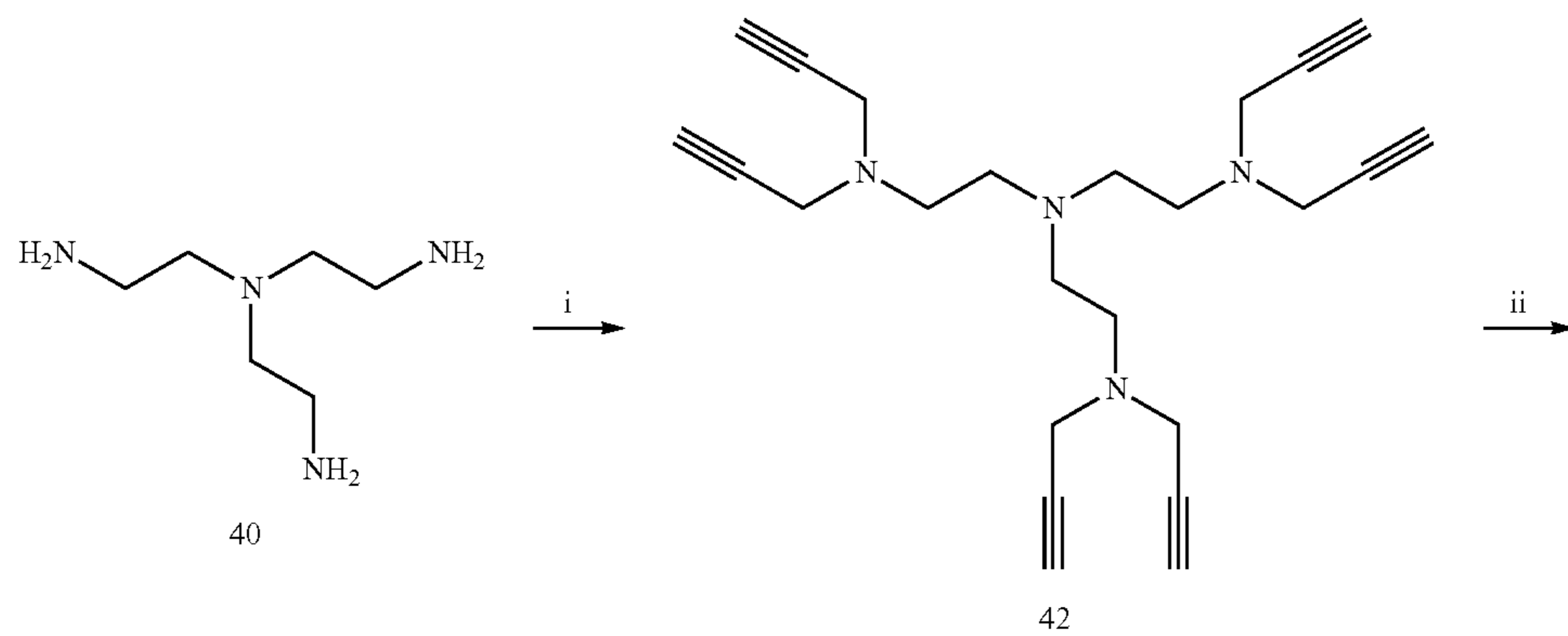
Scheme 14. Synthesis of a 'Click Reaction'-derived hexameric dendrimer.
