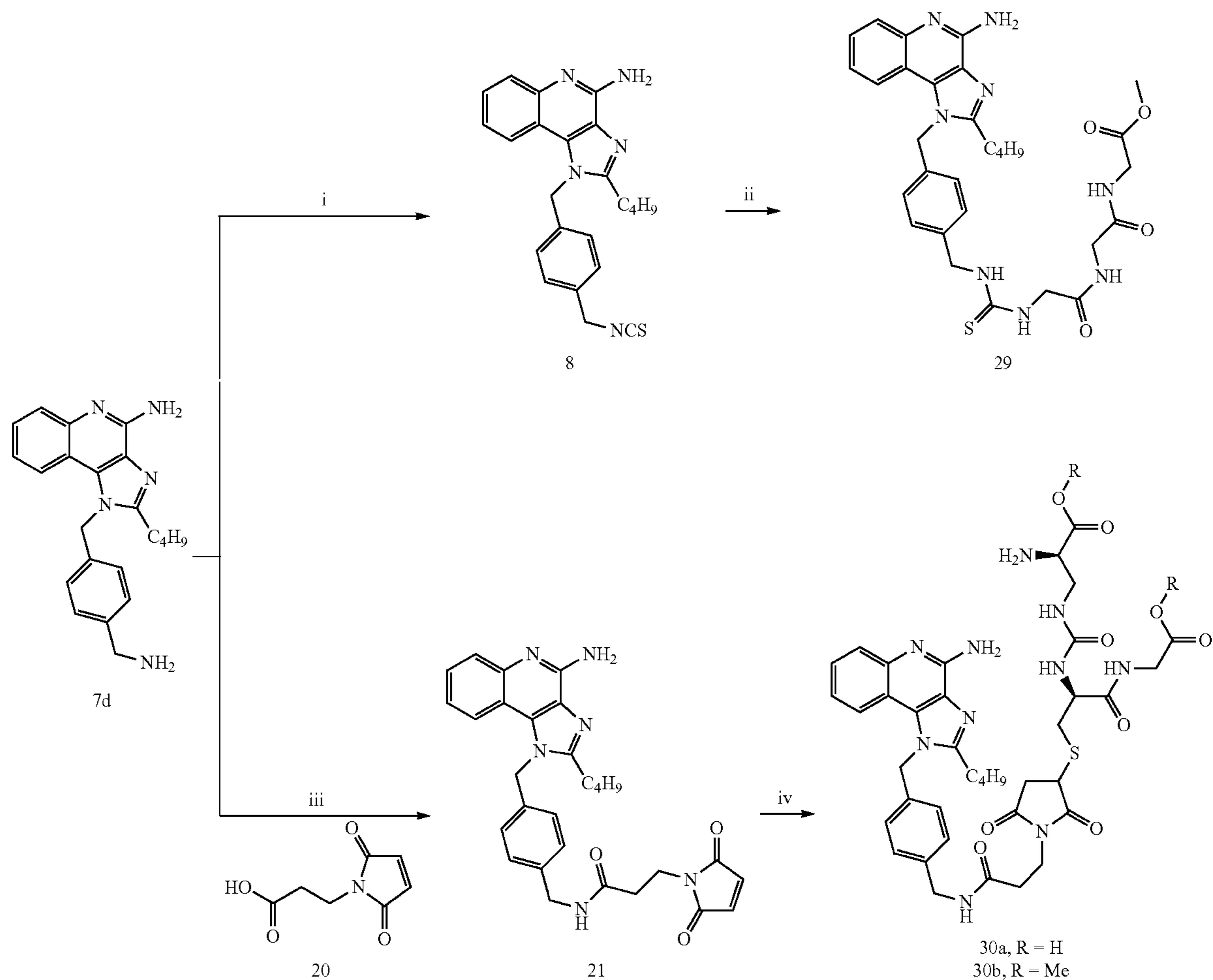
Scheme 7. Syntheses of isothiocyanate and maleimide imidazoquinoline derived compounds of 7d, and their corresponding model peptide conjugates.
