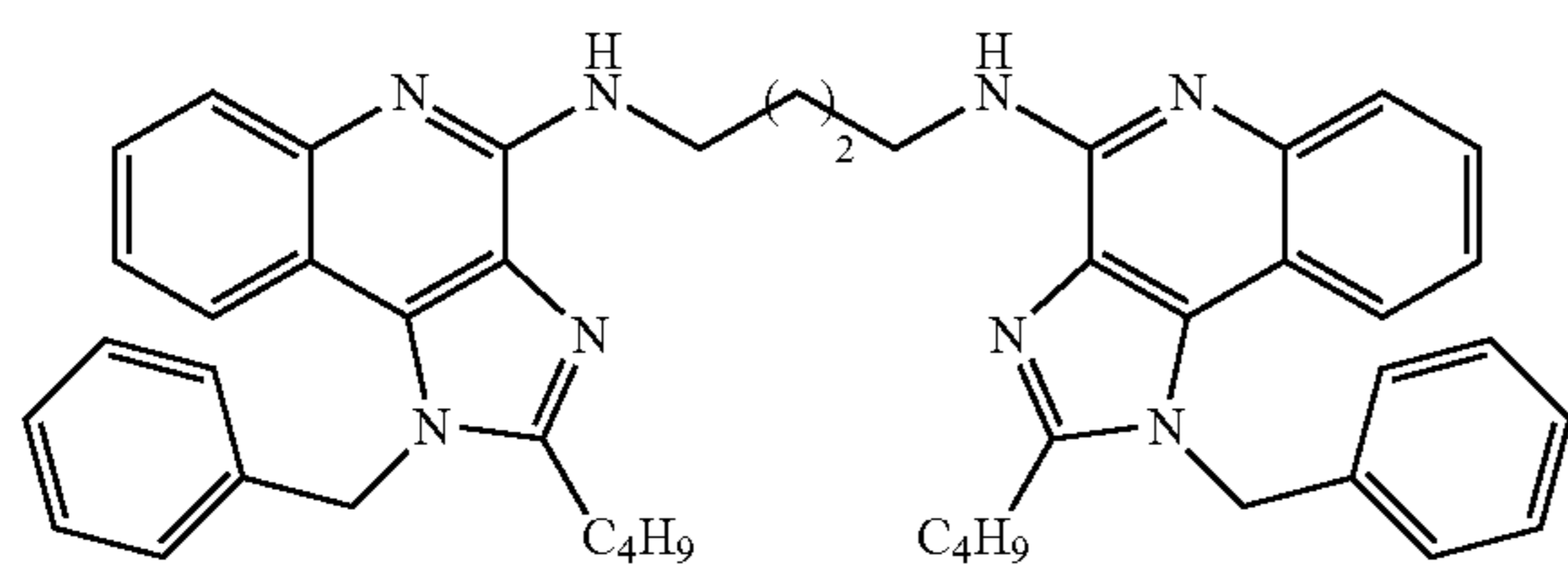
51a: N 1 ,N 4 -bis(1-benzyl-2-butyl-1H-imidazo[4,5-c]quinolin-4-yl)butane-1,4-diamine
