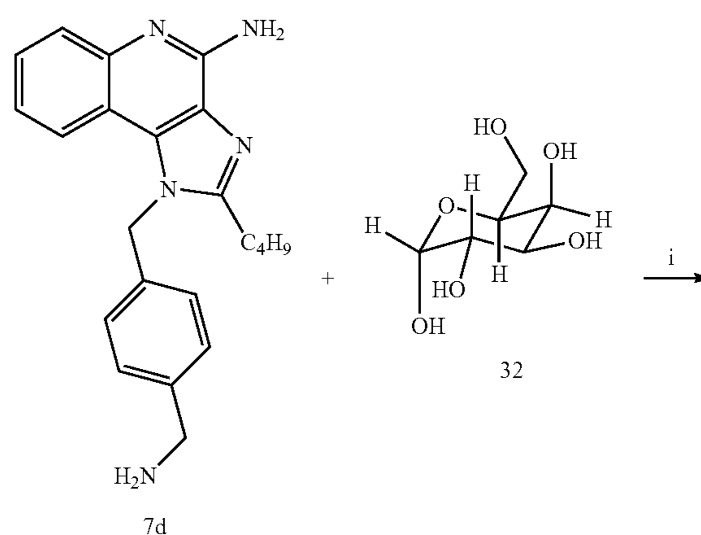
Scheme 9. Synthesis of a galactose derivative 33.
