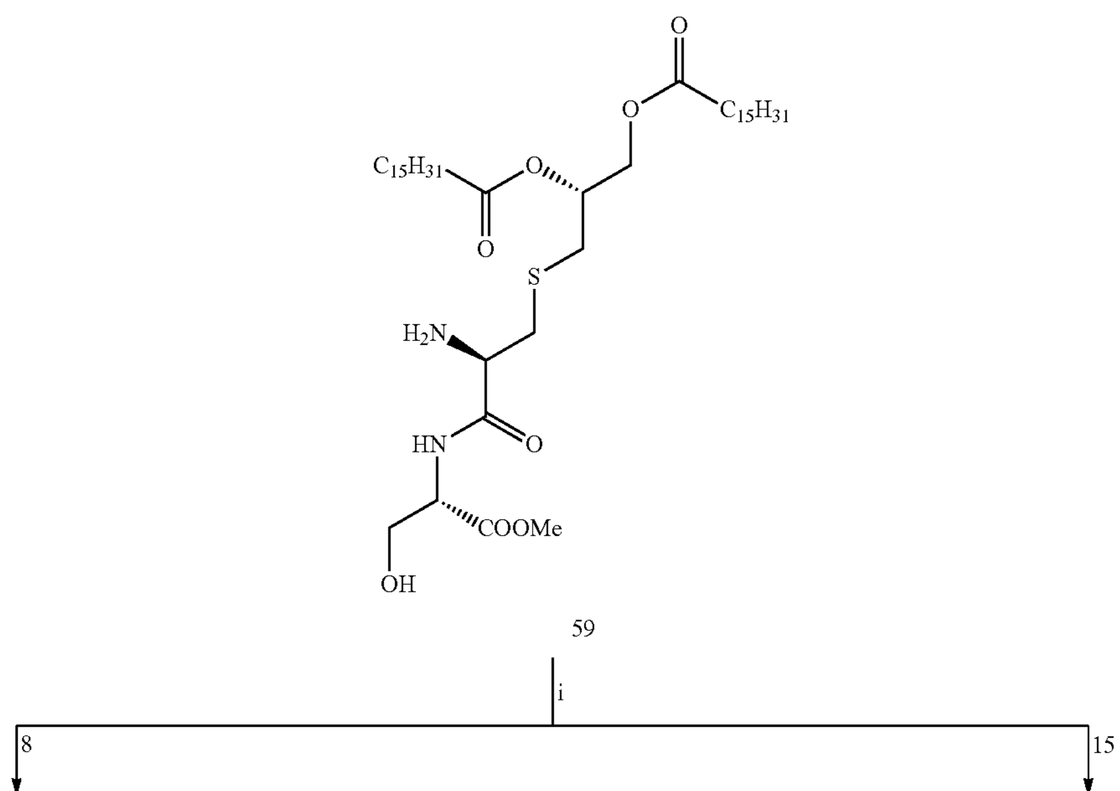
Scheme 20. Synthesis of thioureau-linked TLR-2/7 hybrid compounds 60 and 61.
