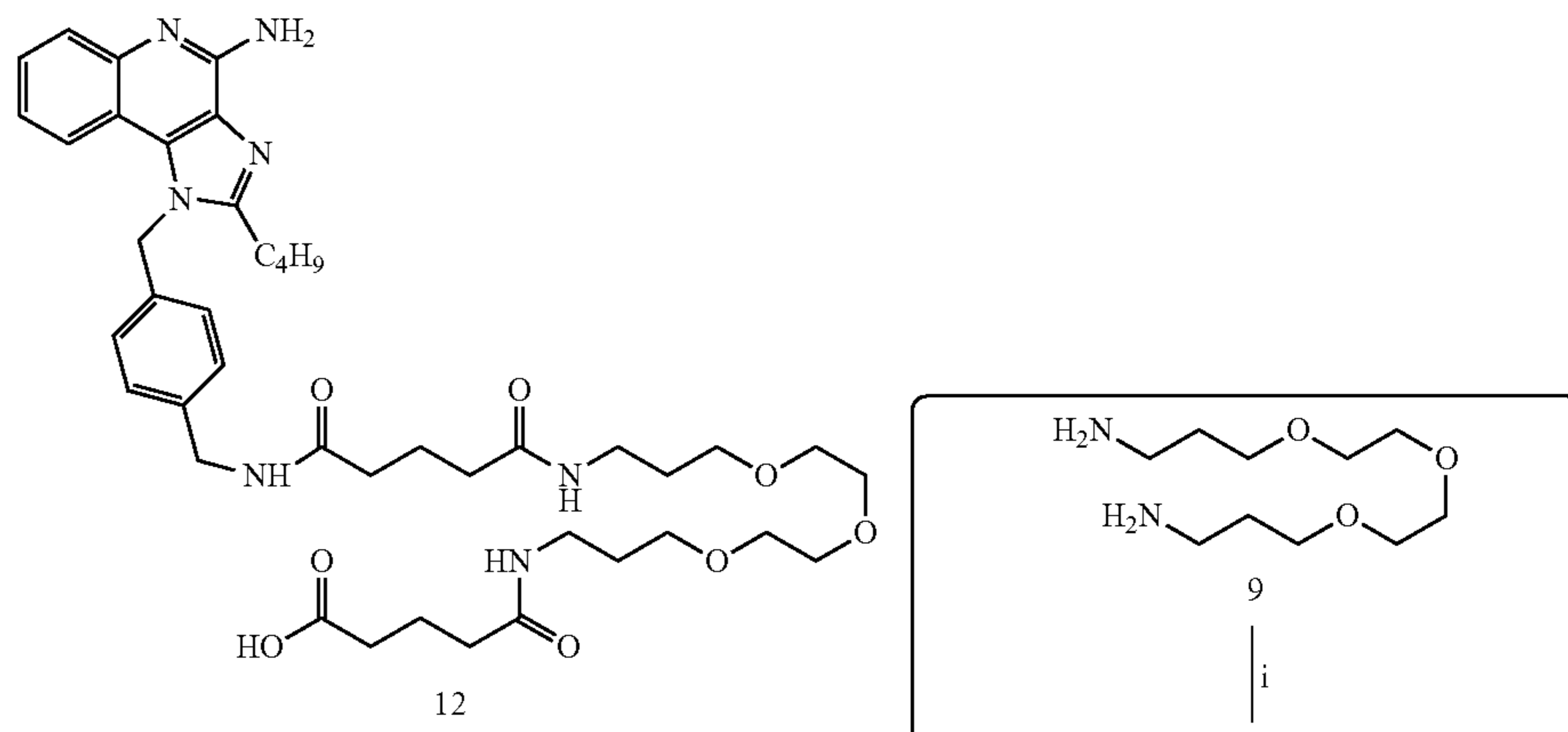
Scheme 2. Syntheses of derivatives of 7d.
