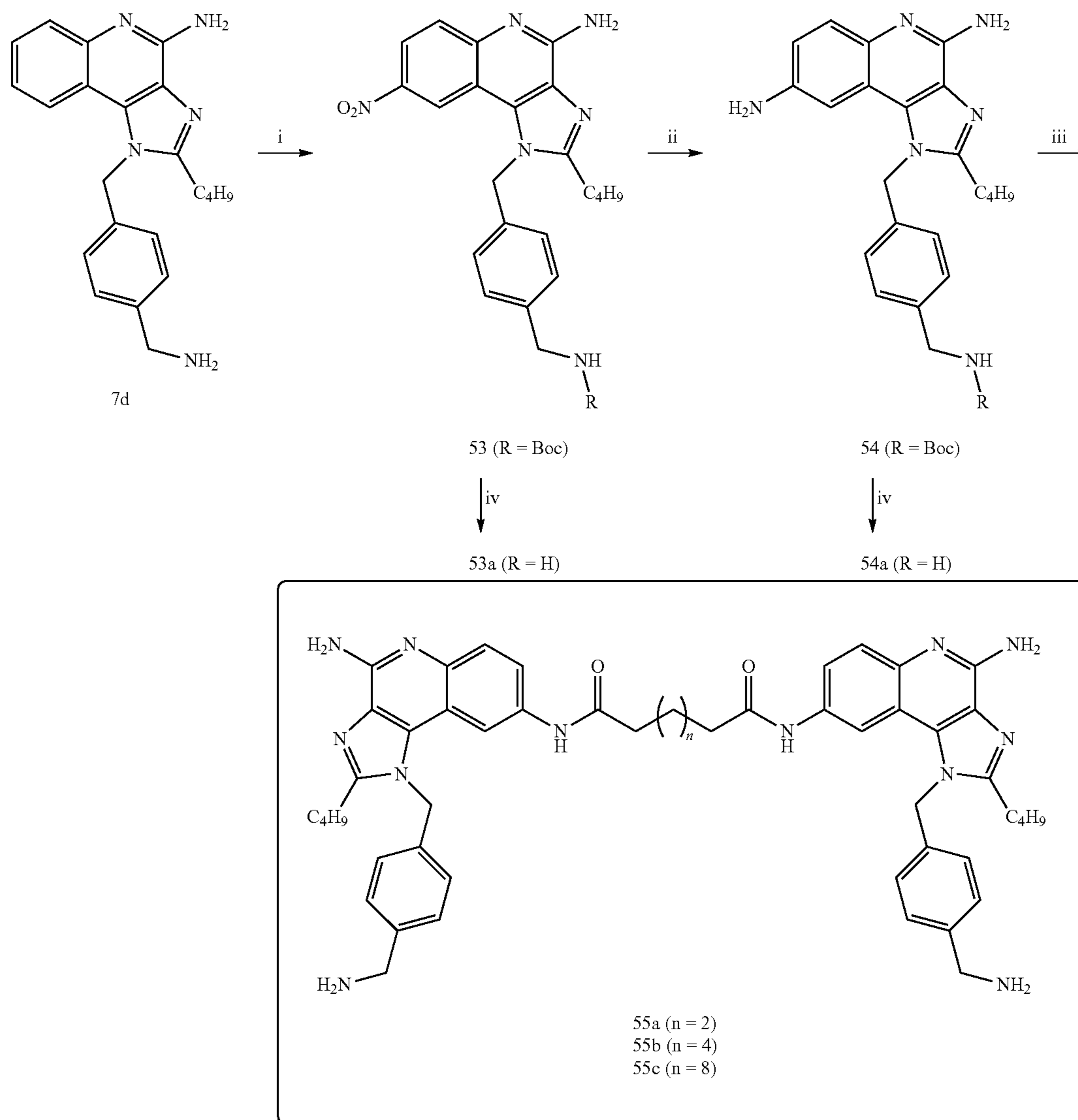
Scheme 18. Syntheses of imidazoquinoline dimers linked at C8—NH 2
