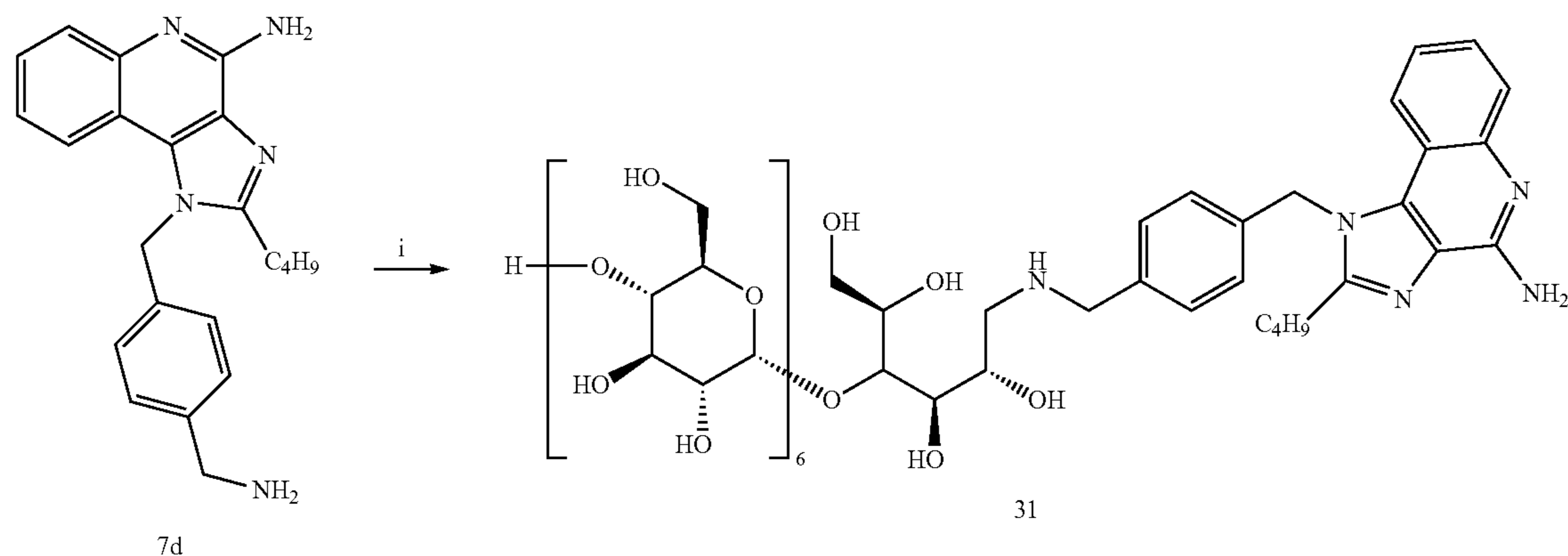
Scheme 8. Syntheses of the maltoheptaose conjugate.
