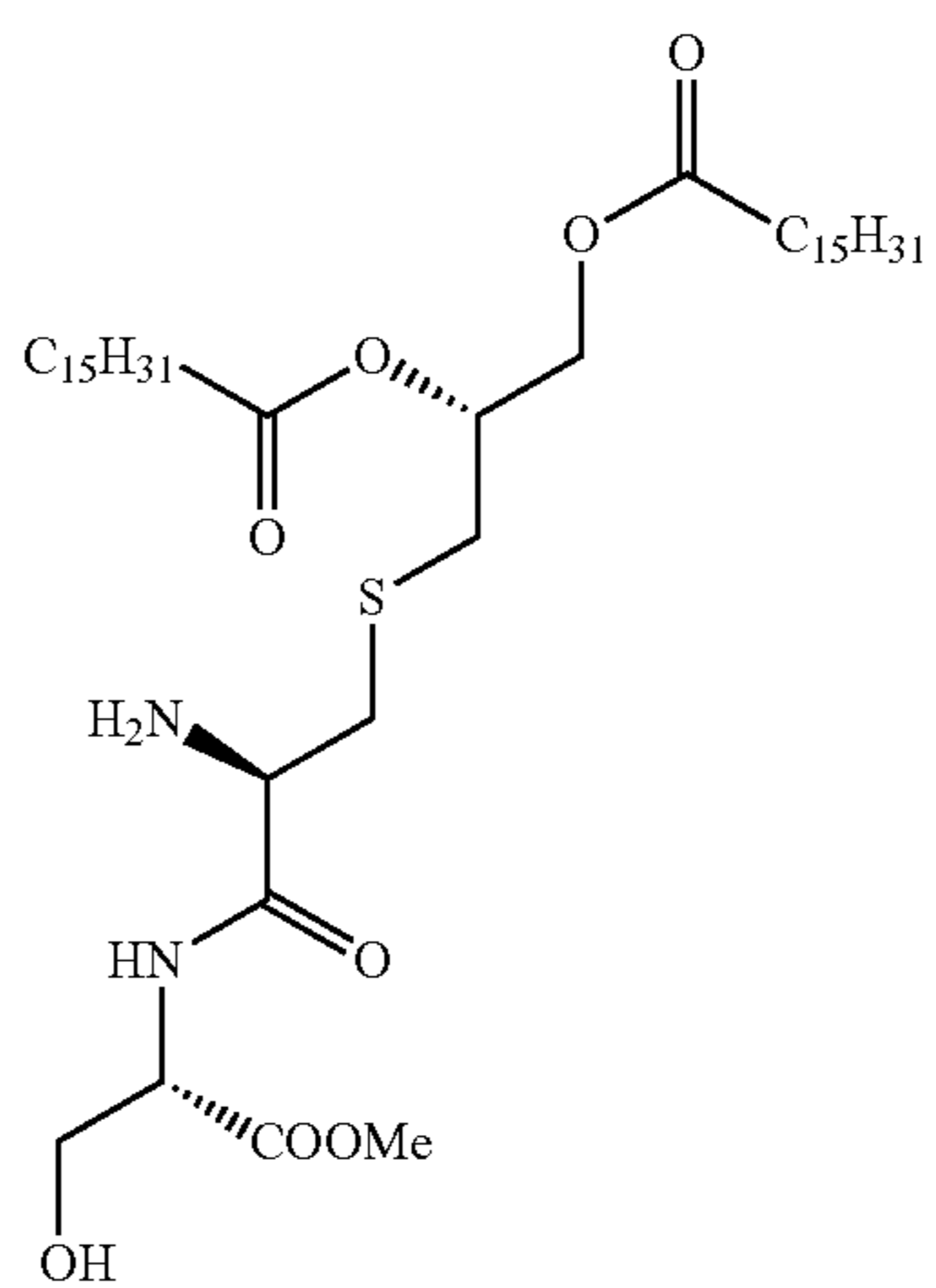
Scheme 22. Synthesis of thiourea-linked TLR-2/7 hybrid compounds 64 and 65.
