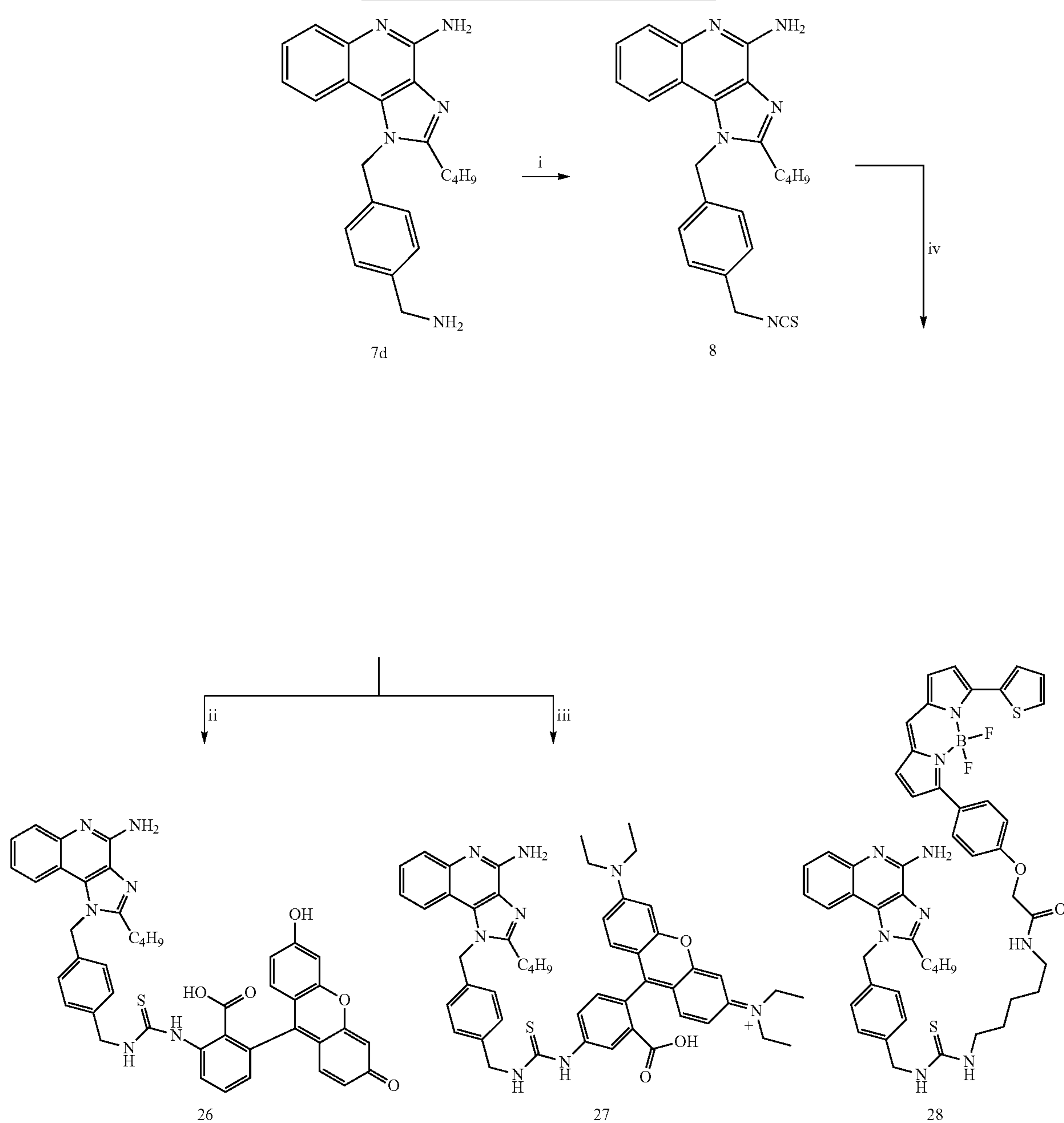
Scheme 6. Syntheses of fluorescent analogues of 7d.
