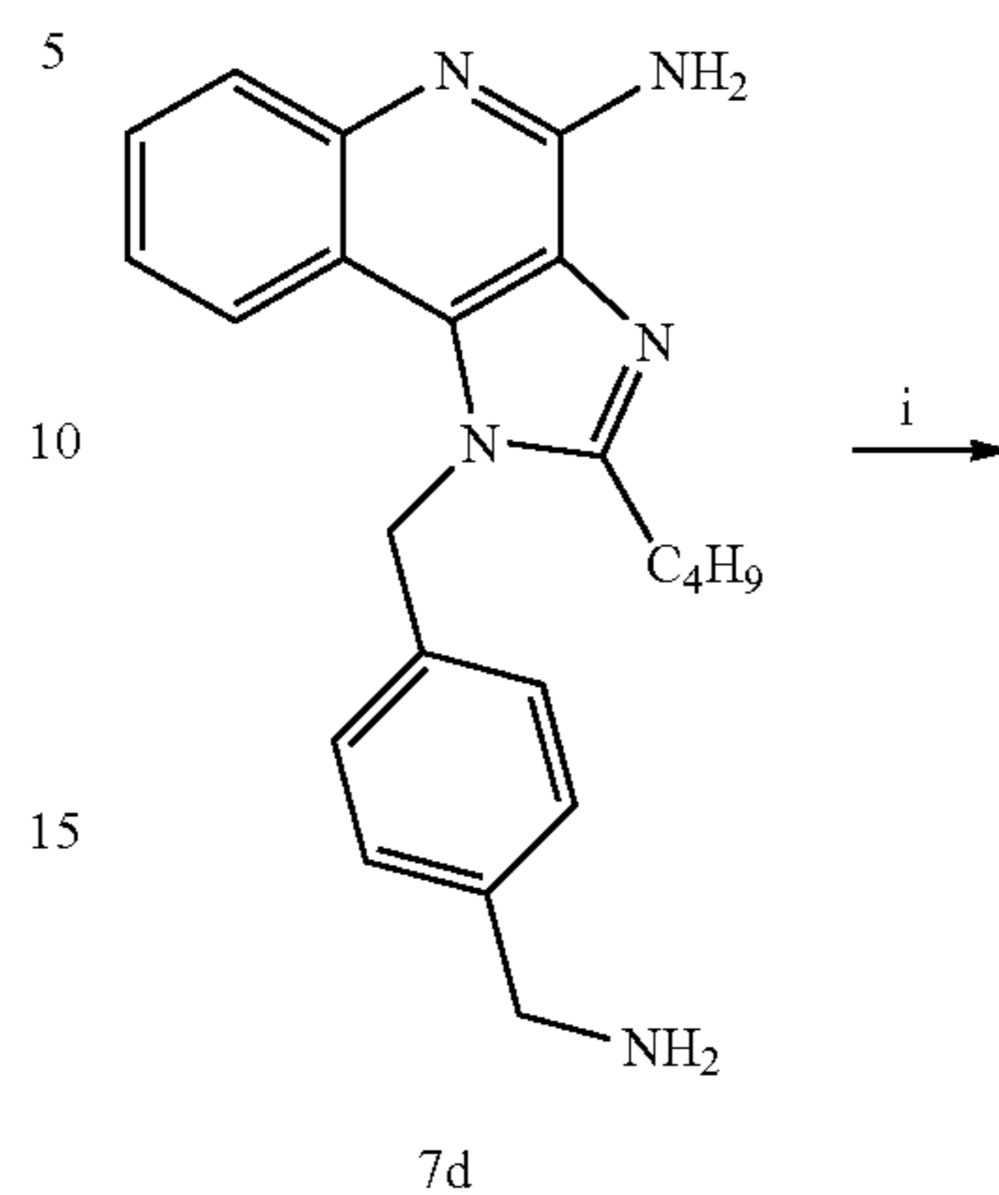
Scheme 17. Syntheses of imidazoquinoline dimers linked at N 1 -(4-aminomethylene)benzyl.
