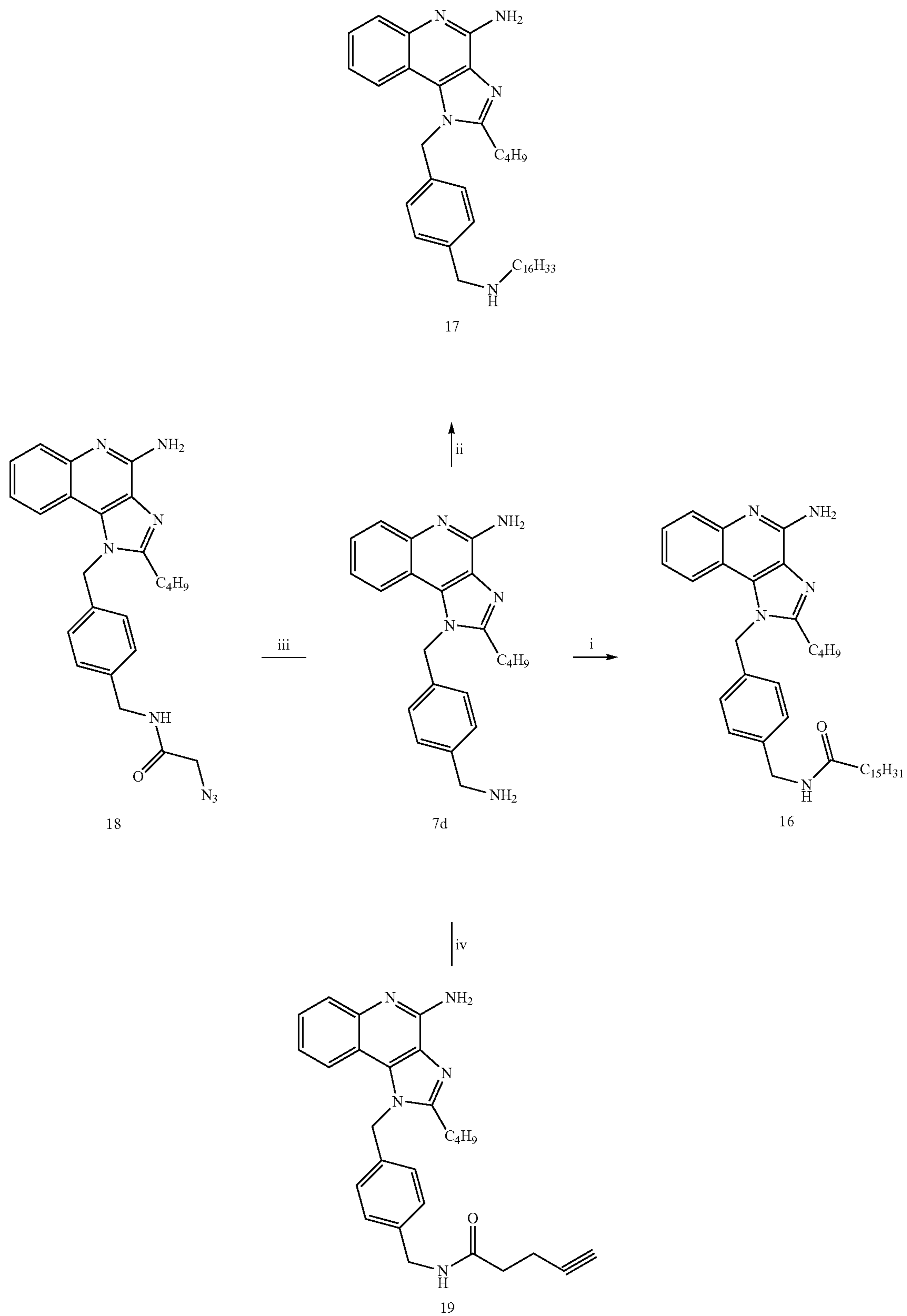
Scheme 3. Syntheses of derivatives of 7d.
