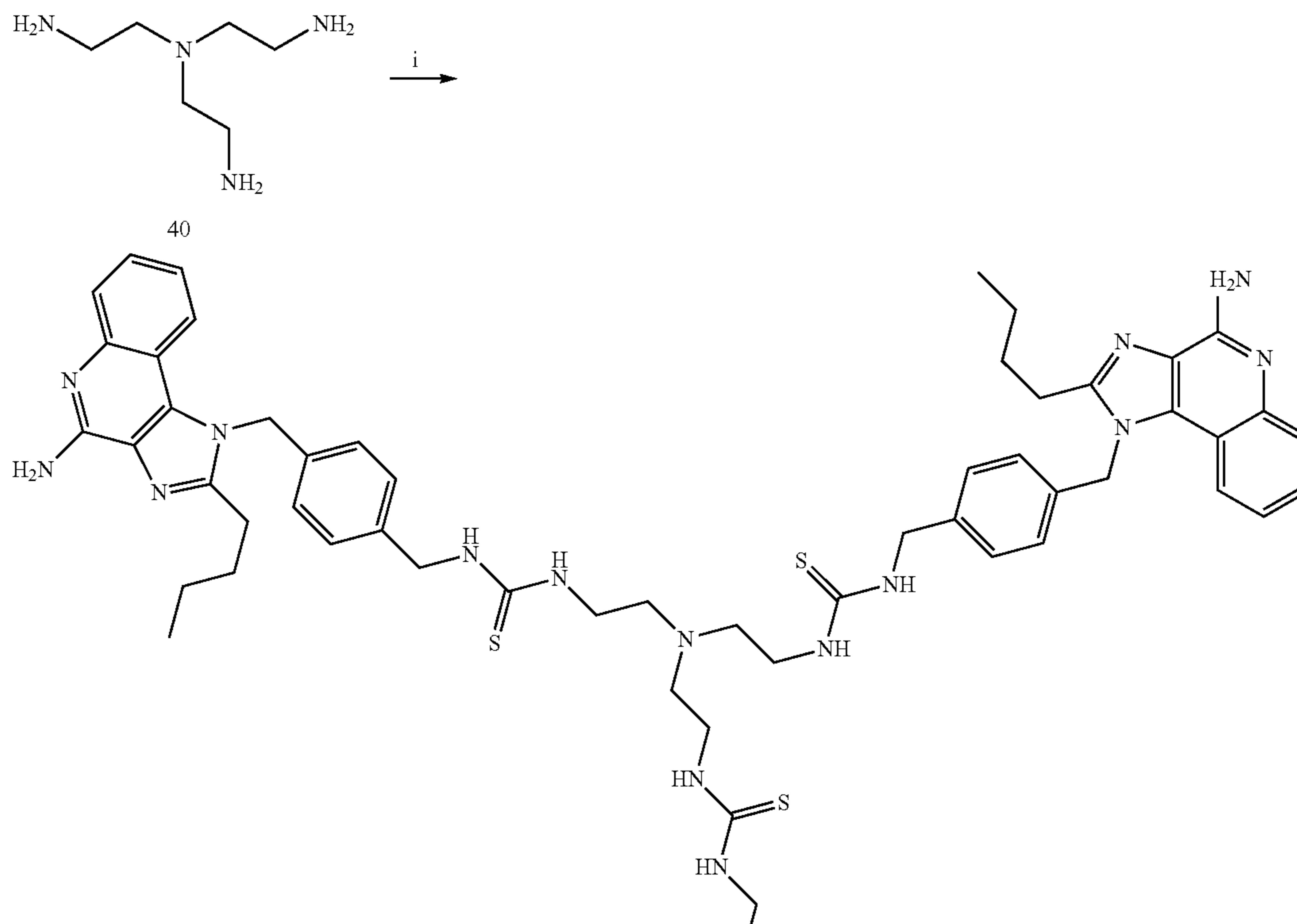
Scheme 13. Syntheses of the trimeric imidazoquinoline dendrimer.
