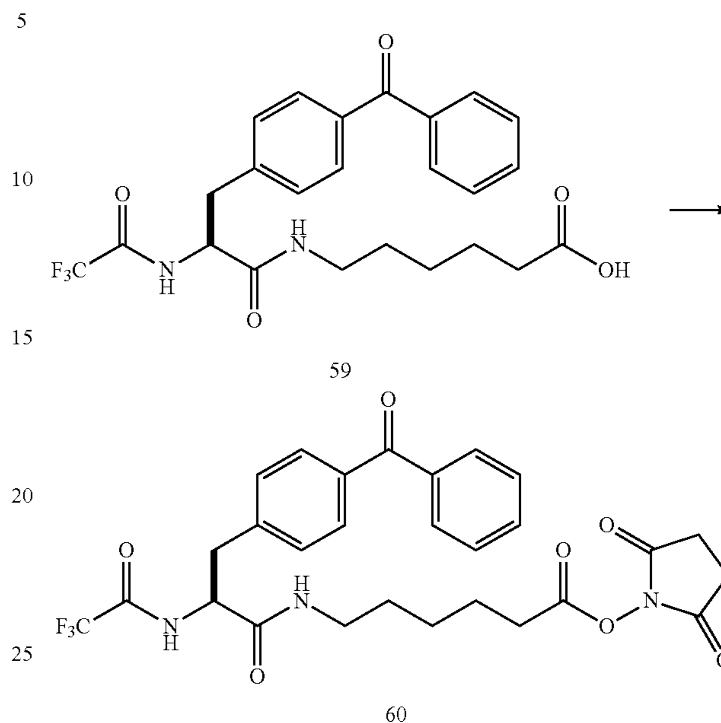
N—(N'-Trifluoroacetyl(4-benzoylphenylalanine)) aminocaproic acid N-hydroxysuccinimide ester (60)
