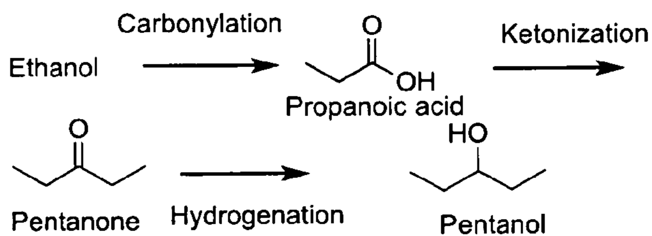
Fig. 11: Synthesis of pentanol from ethanol.
