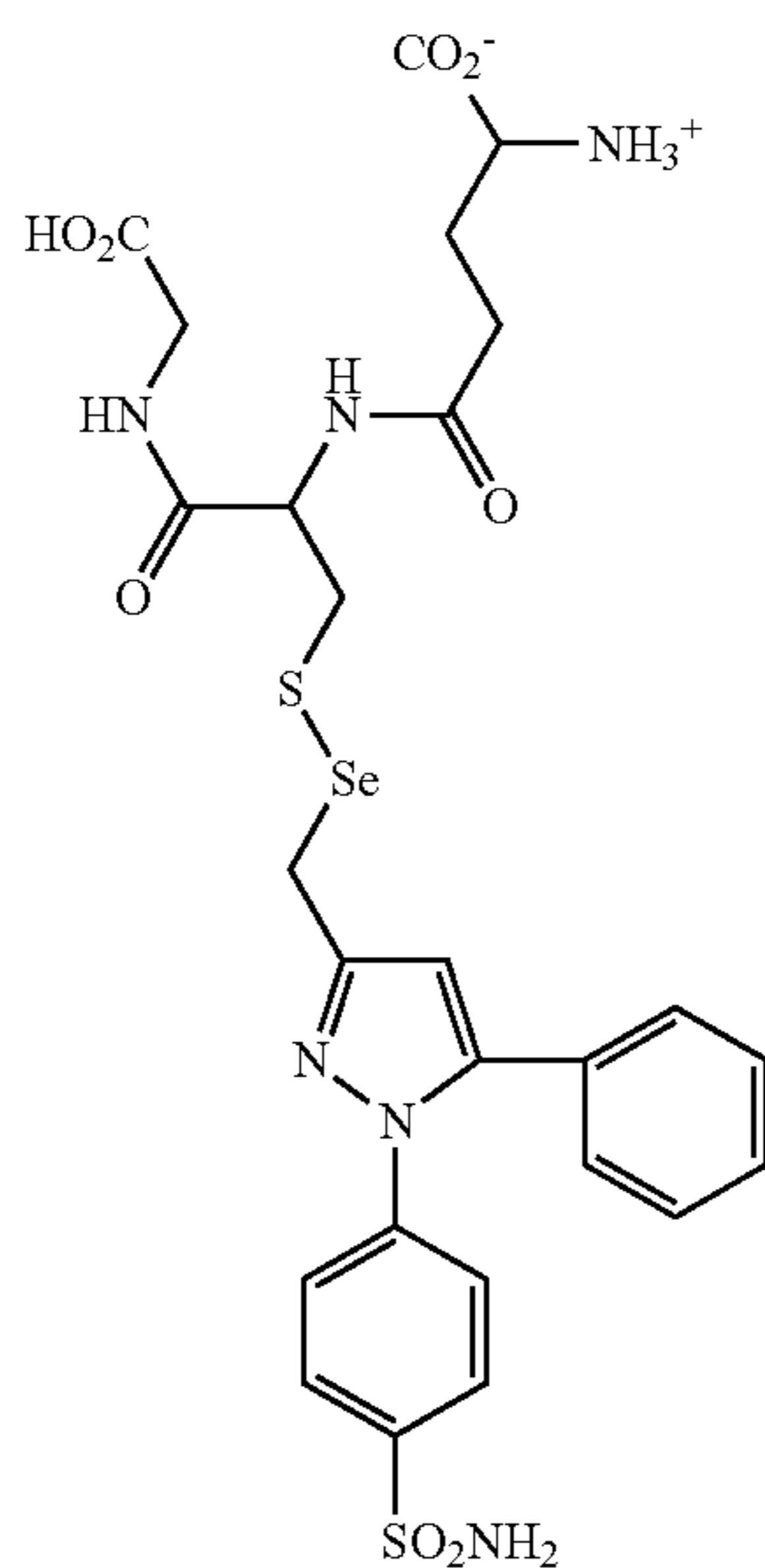
2-amino-4-(1-(carboxymethyl-carbamoyl)-2-[5-phenyl-1-(4-sulfamoylphenyl)-1H-pyrazol-3yl)methylselenanylthiol-ethylcarbamoyl]-butyric acid.
