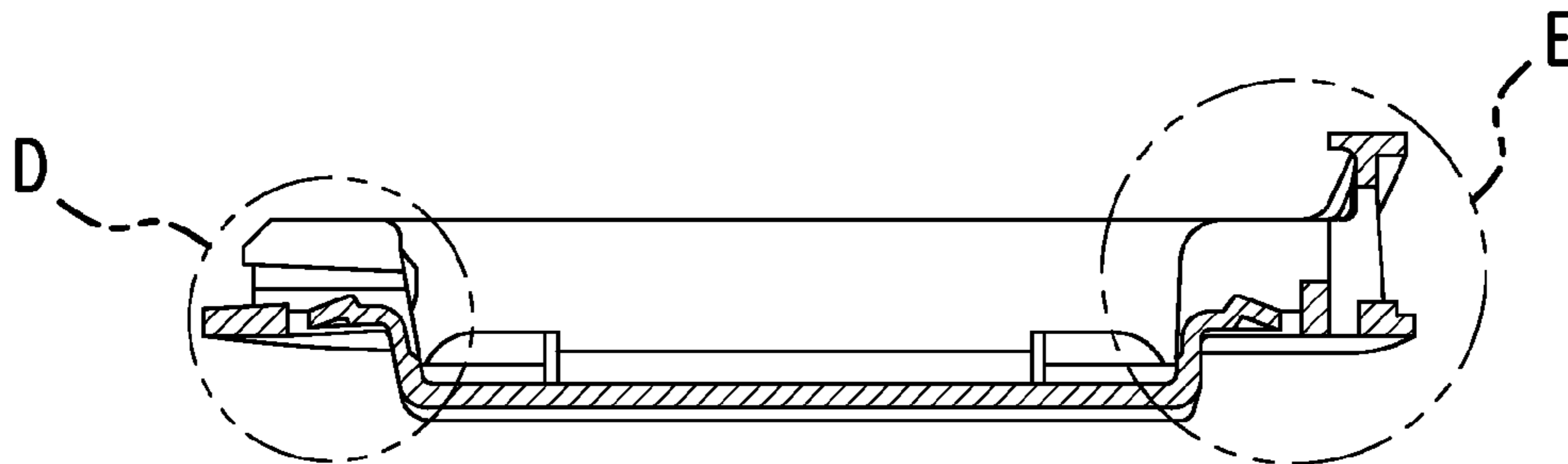
Section C-C
