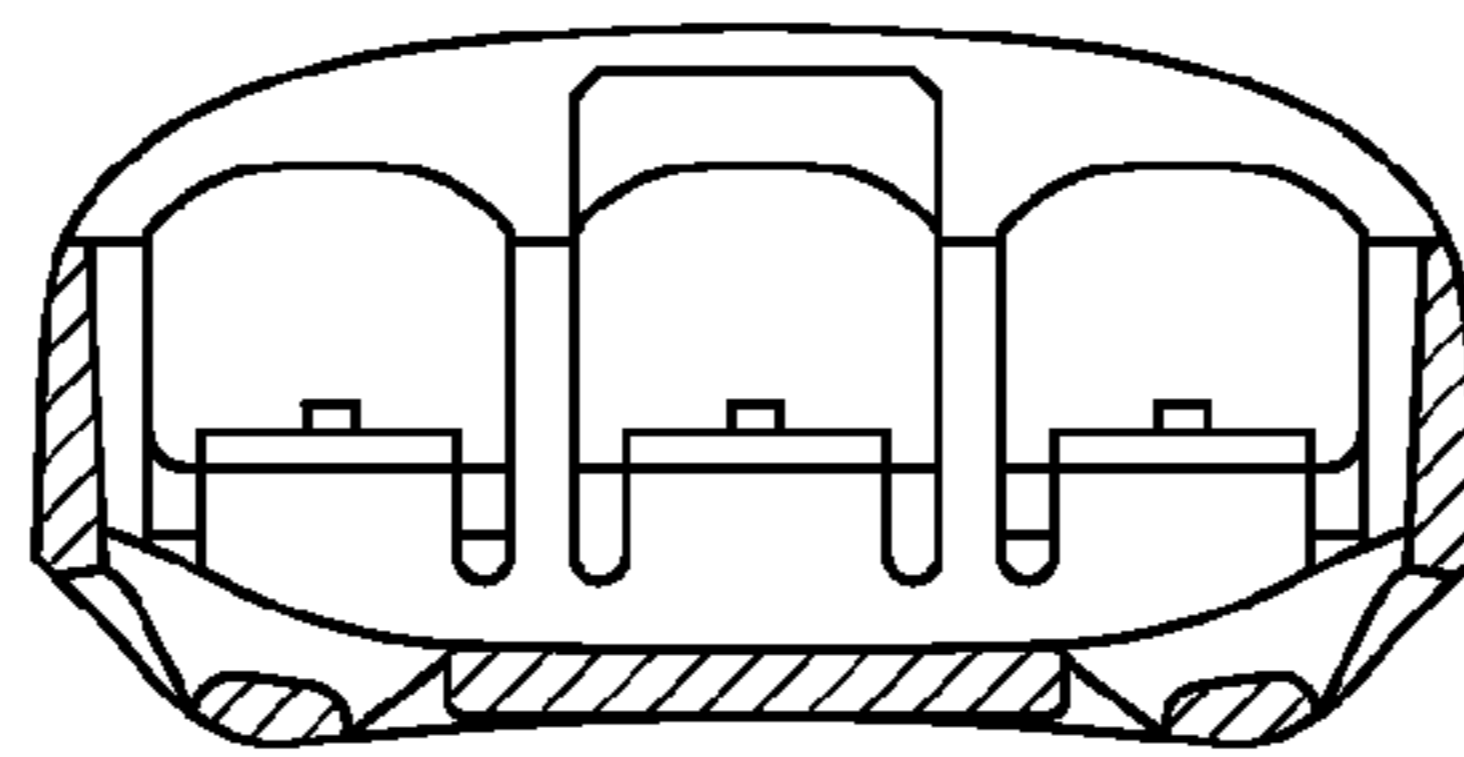
Section B-B
