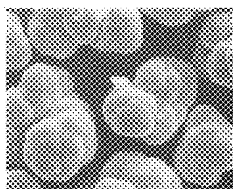
Scanning electron microscope image of an iron(III) orthophosphate with a nanostrange Fe crystal structure produced according to the prior art from Fe(ISO)_4 with phosphoric acid.
