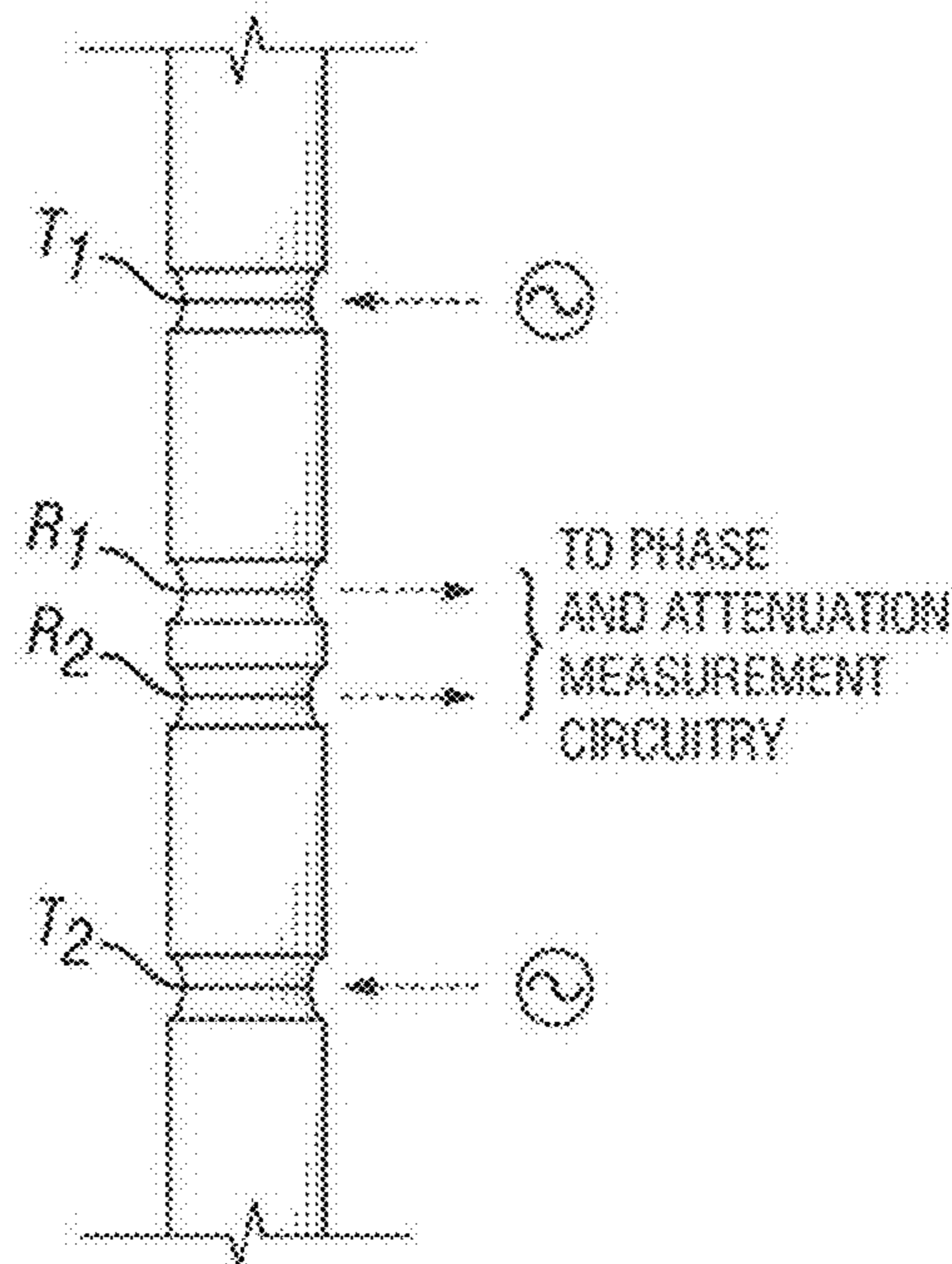
FIG. 2 (Prior Art)
