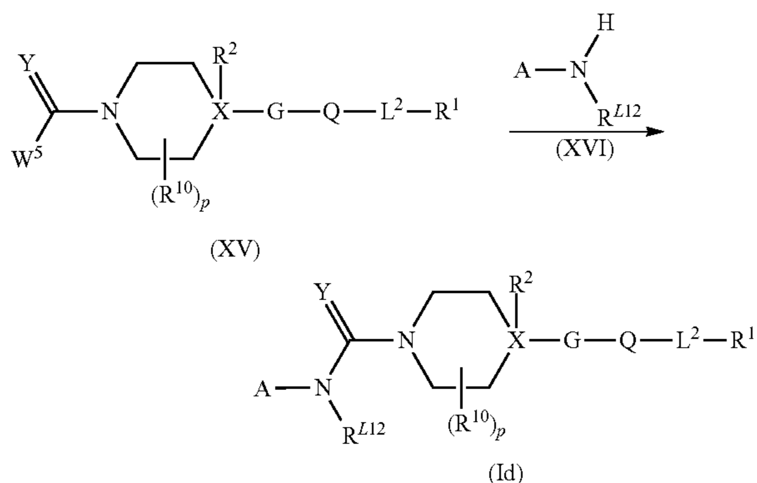
Scheme 11: Process J
