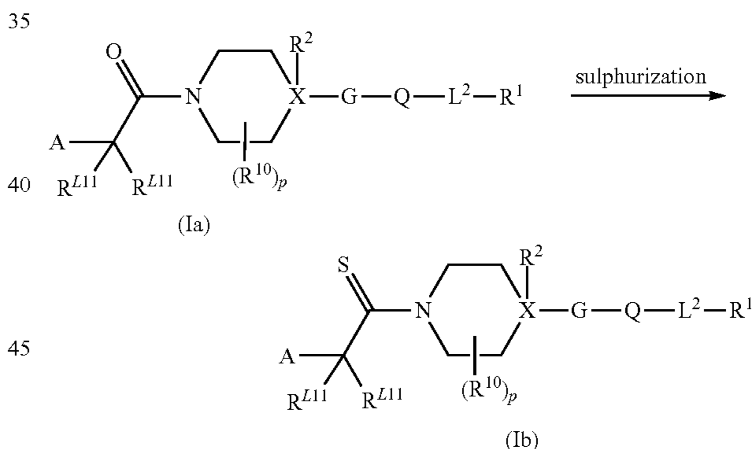
Scheme 7: Process F
