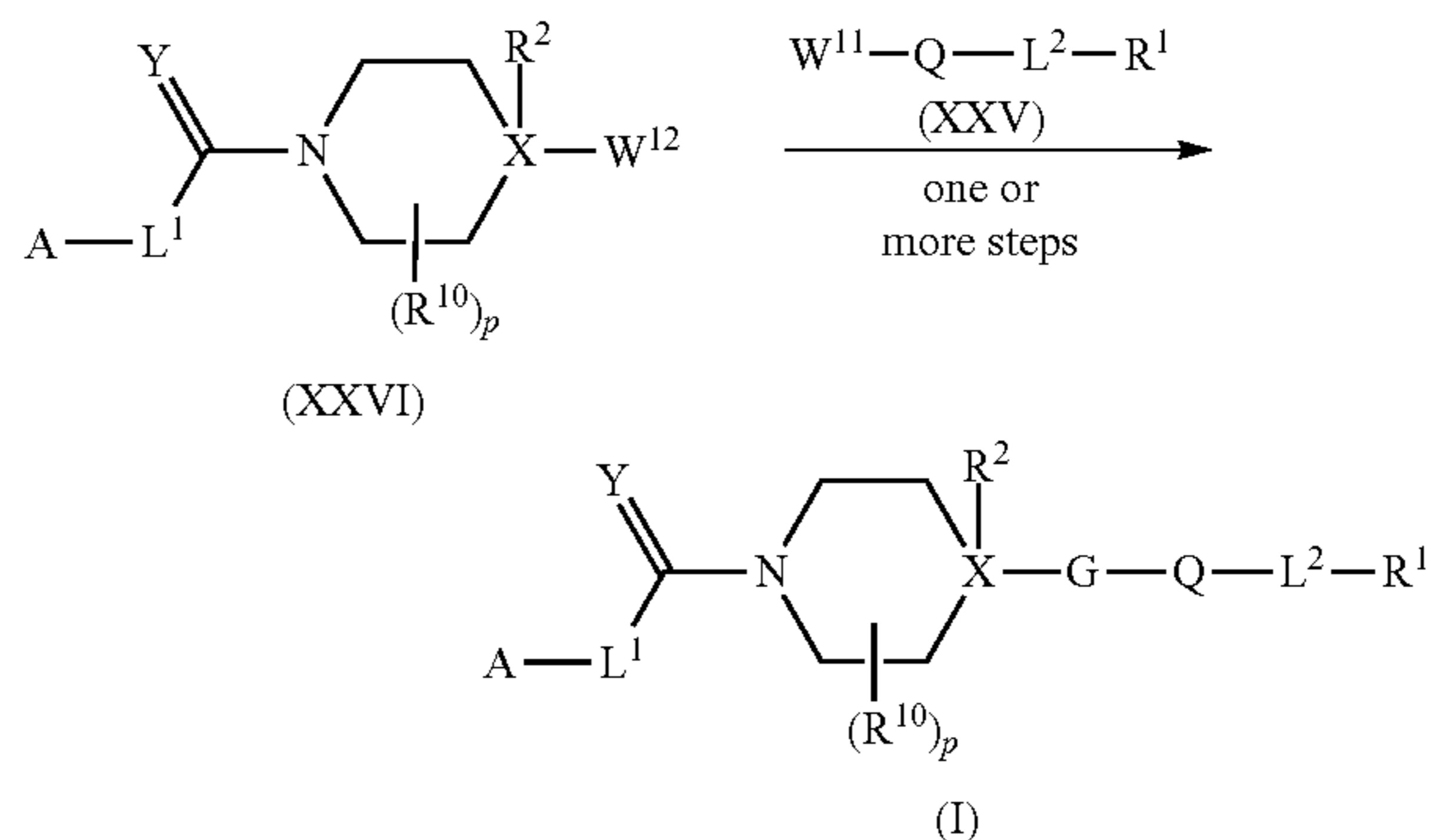
Scheme 4: Process D
