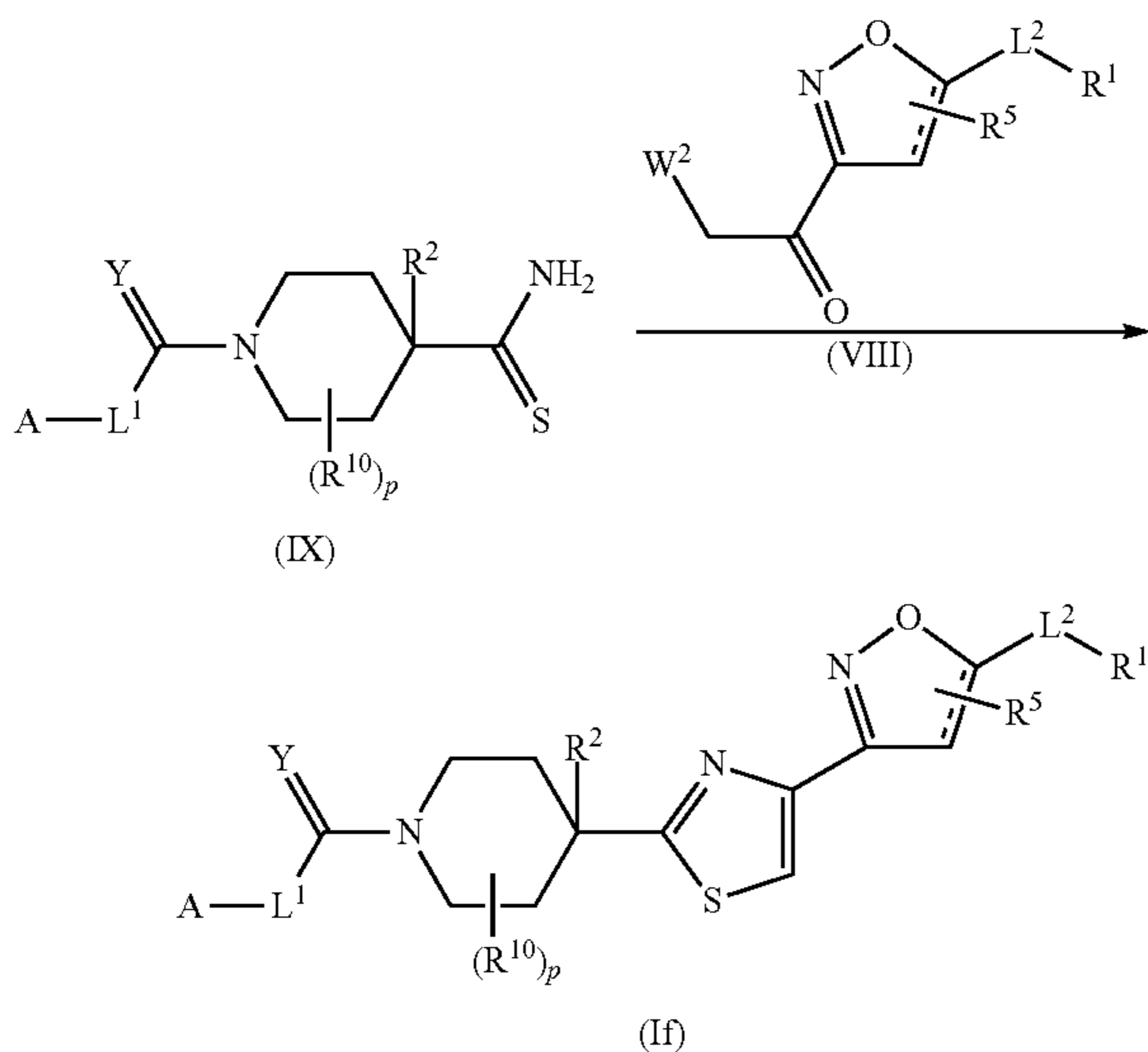
Scheme 5: Process E
