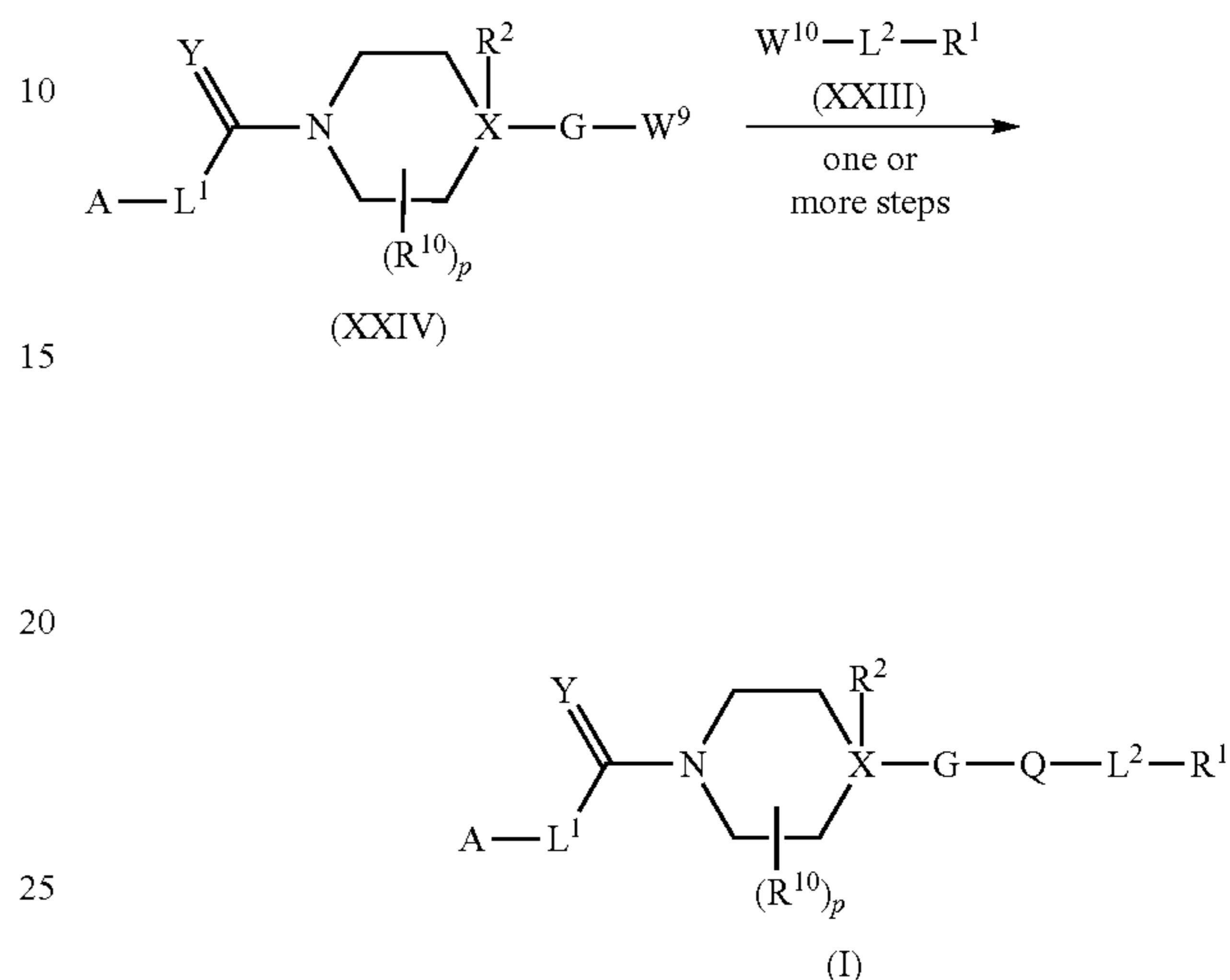
Scheme 1: Process A
