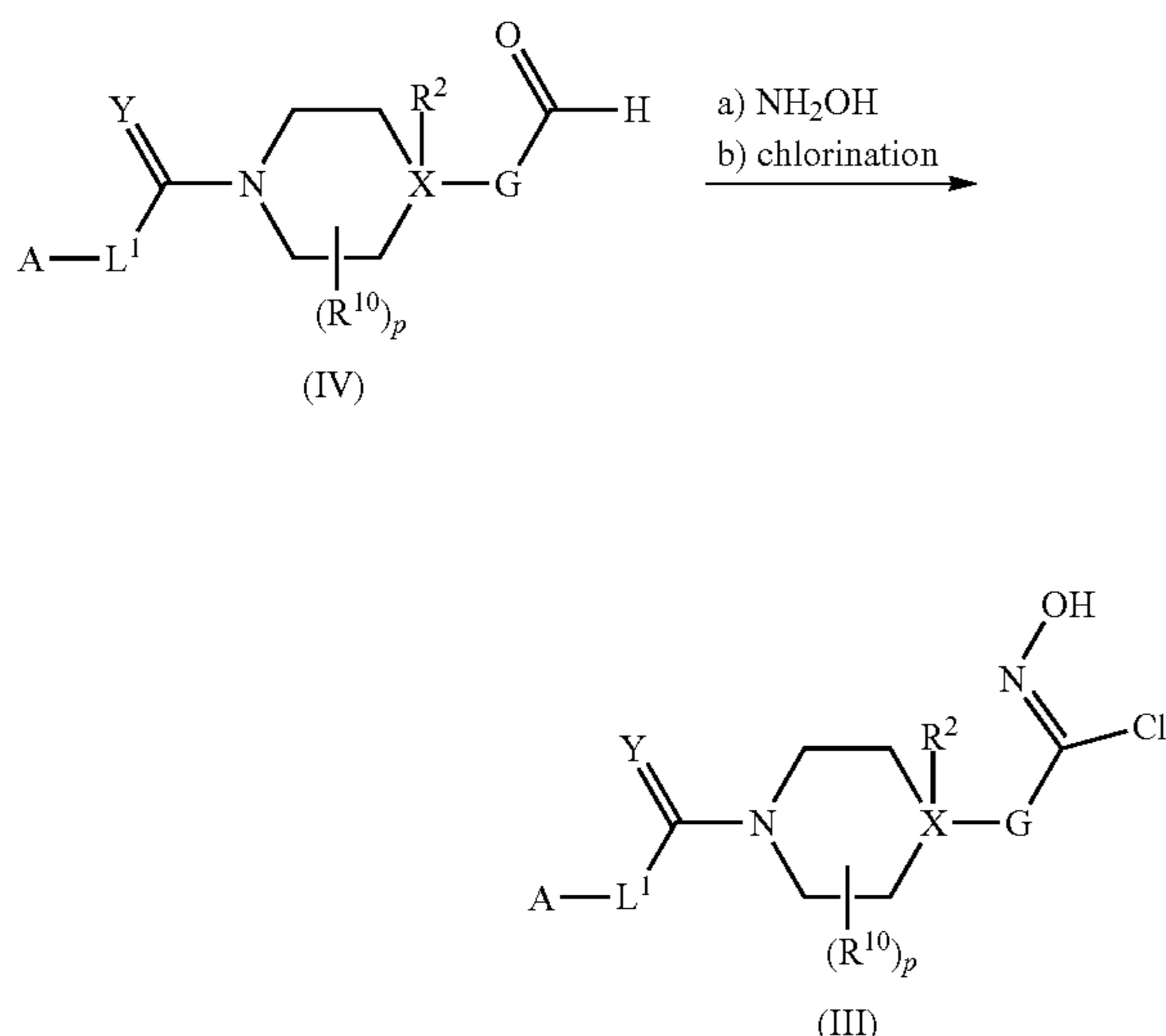
Scheme 3: Process C
