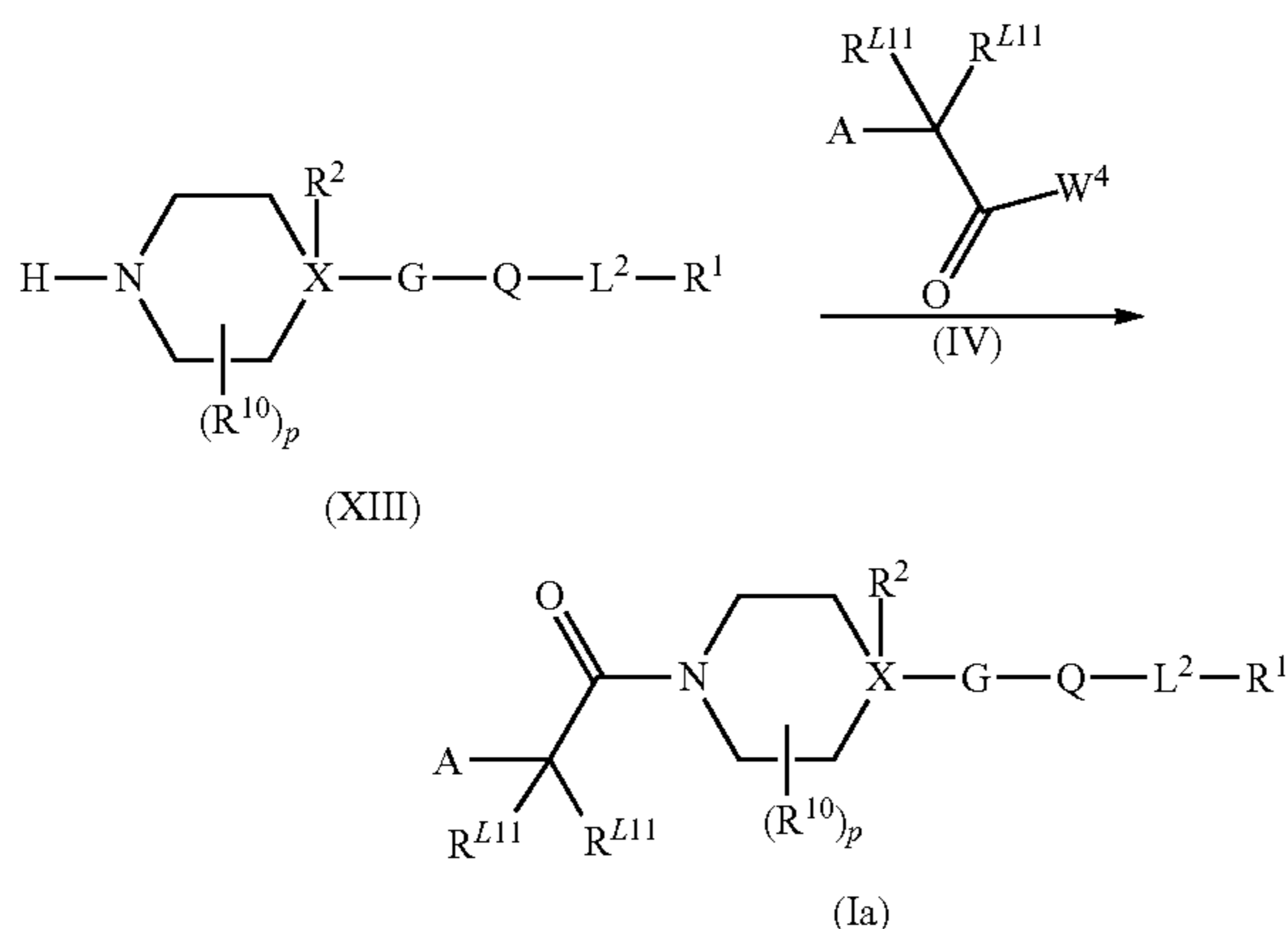
Scheme 8: Process G
