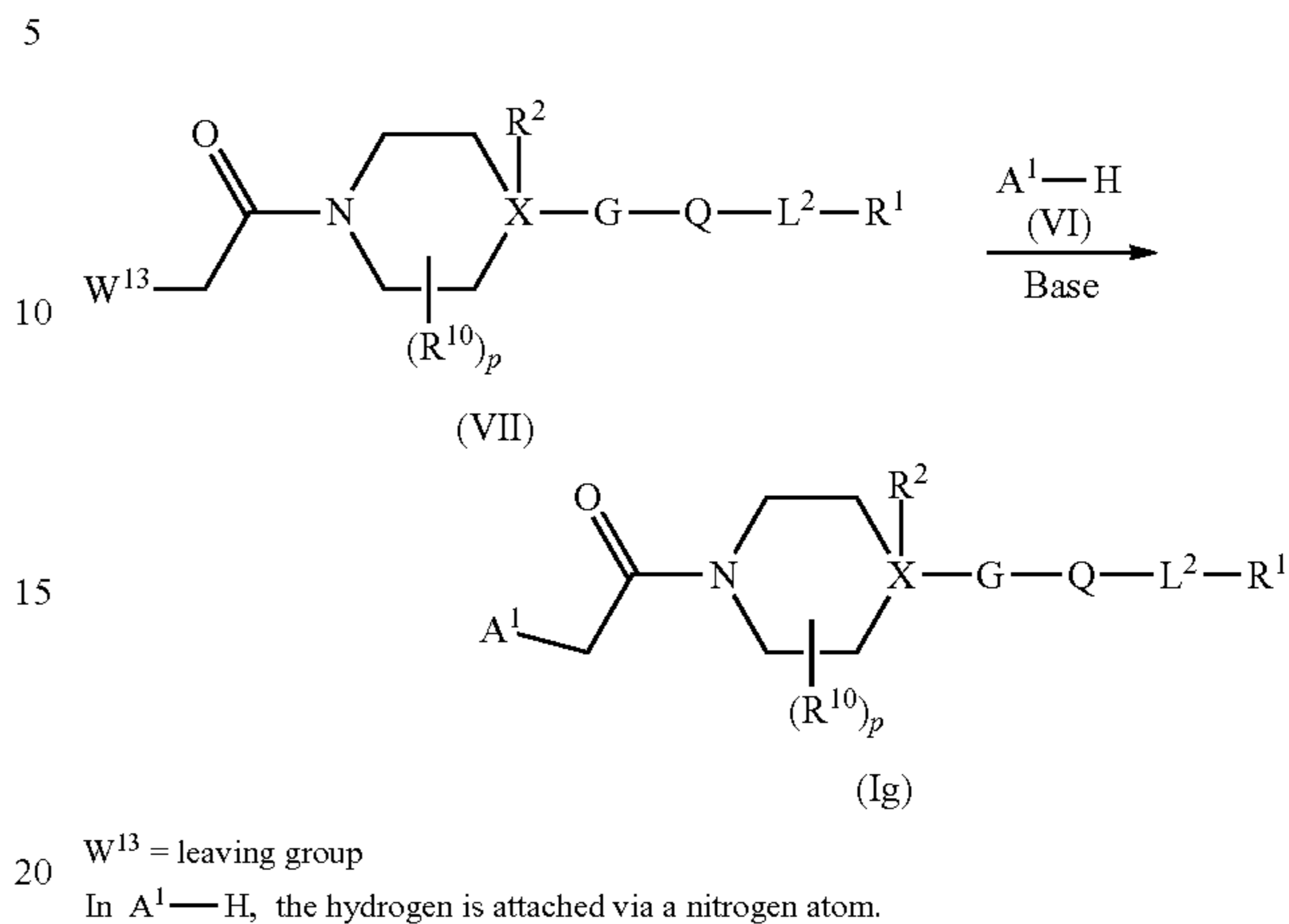
Scheme 9: Process H
