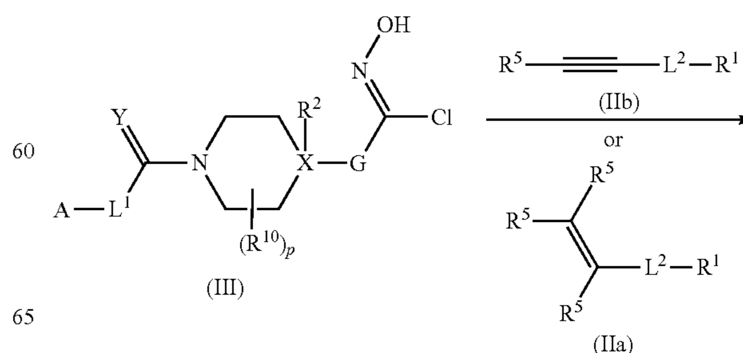
Scheme 2: Process B
