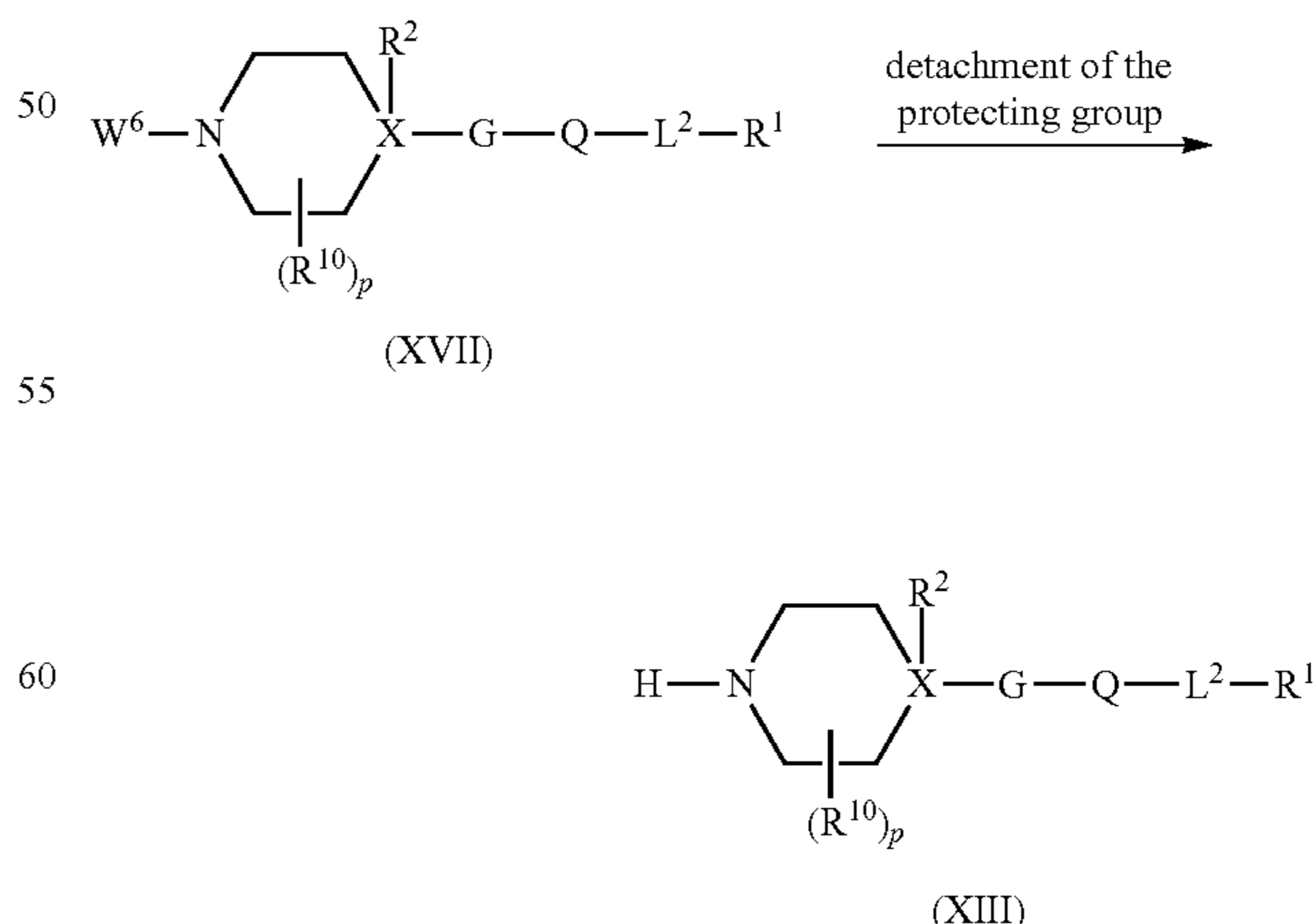
Scheme 12: Process K
