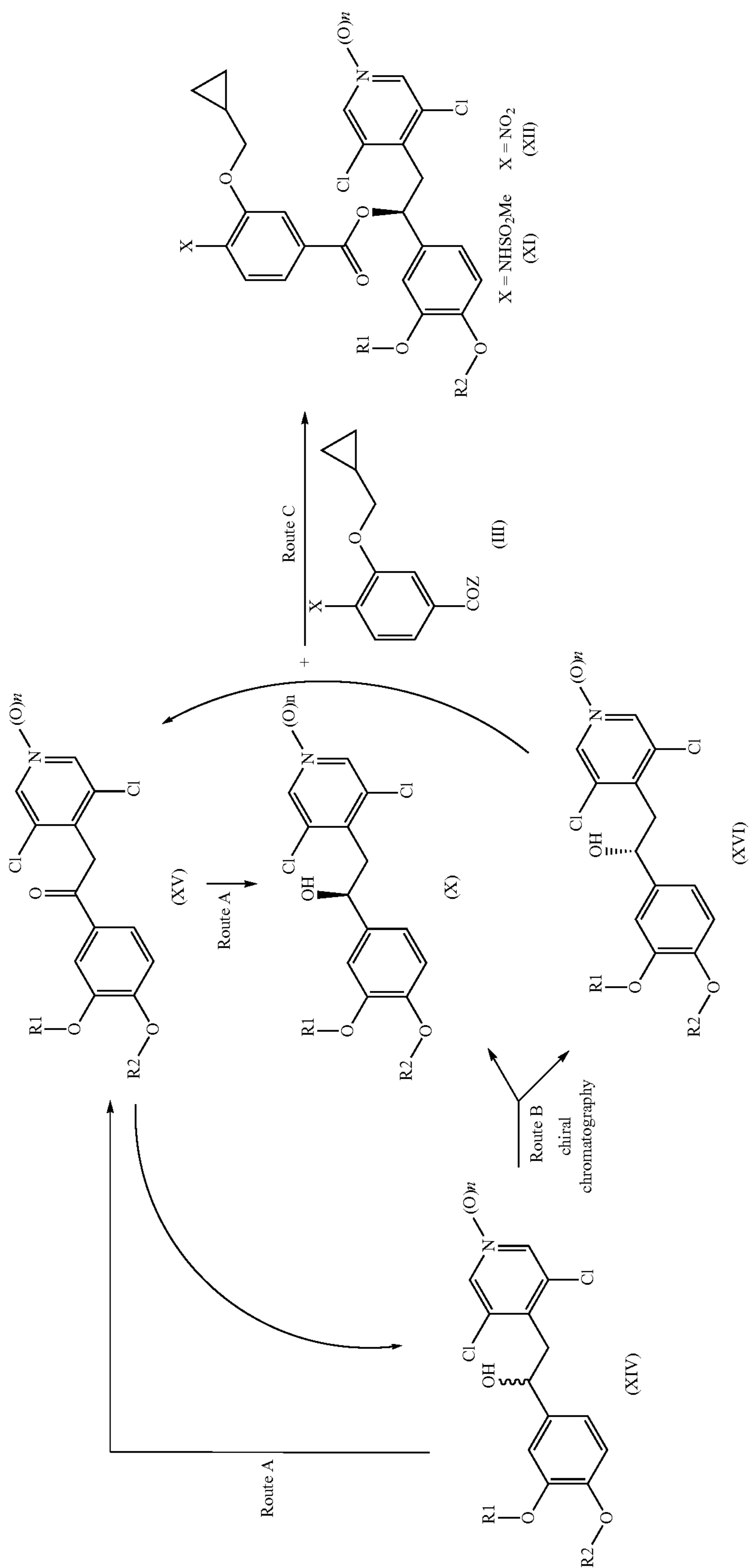
Scheme 4
