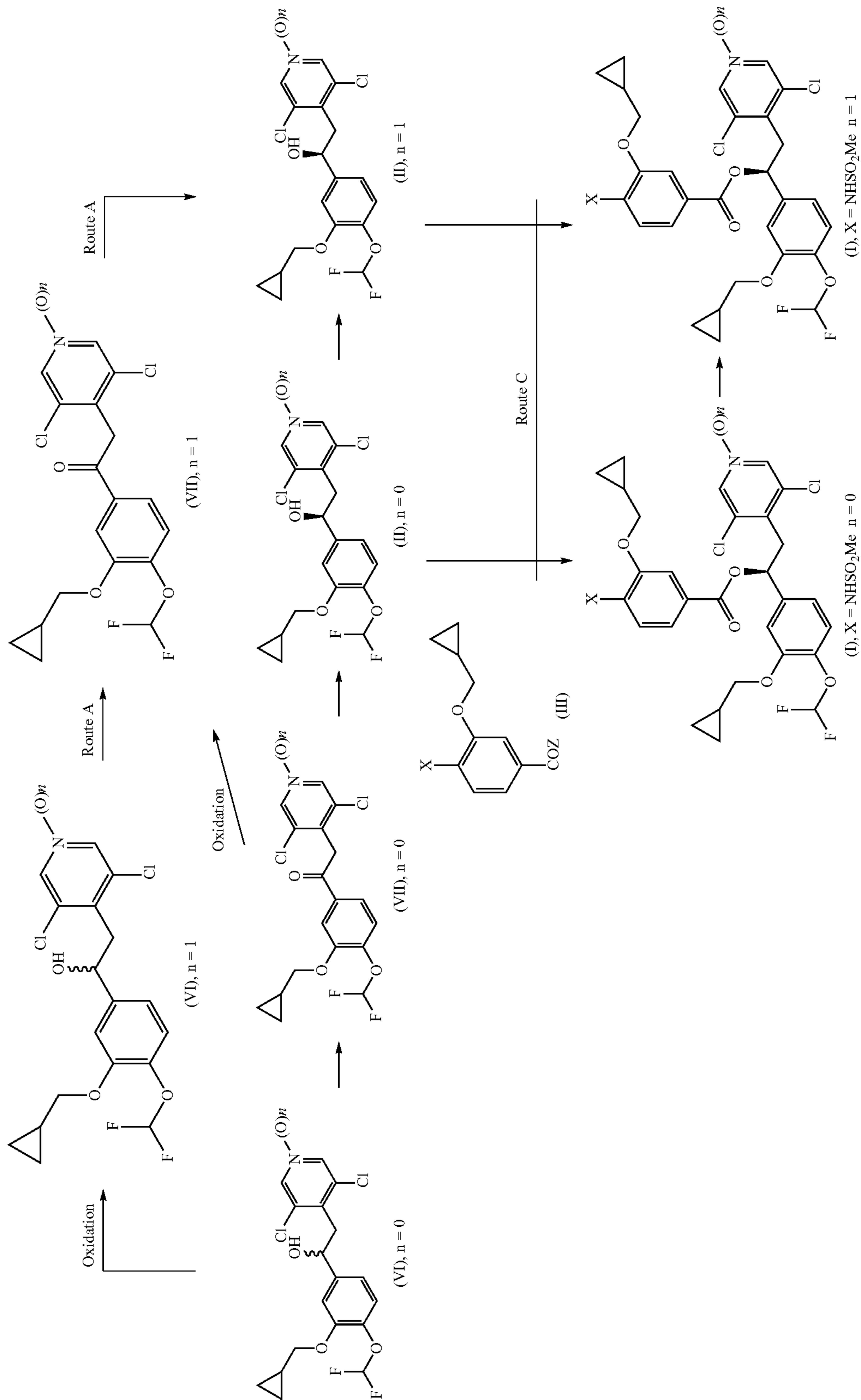
Scheme 2
