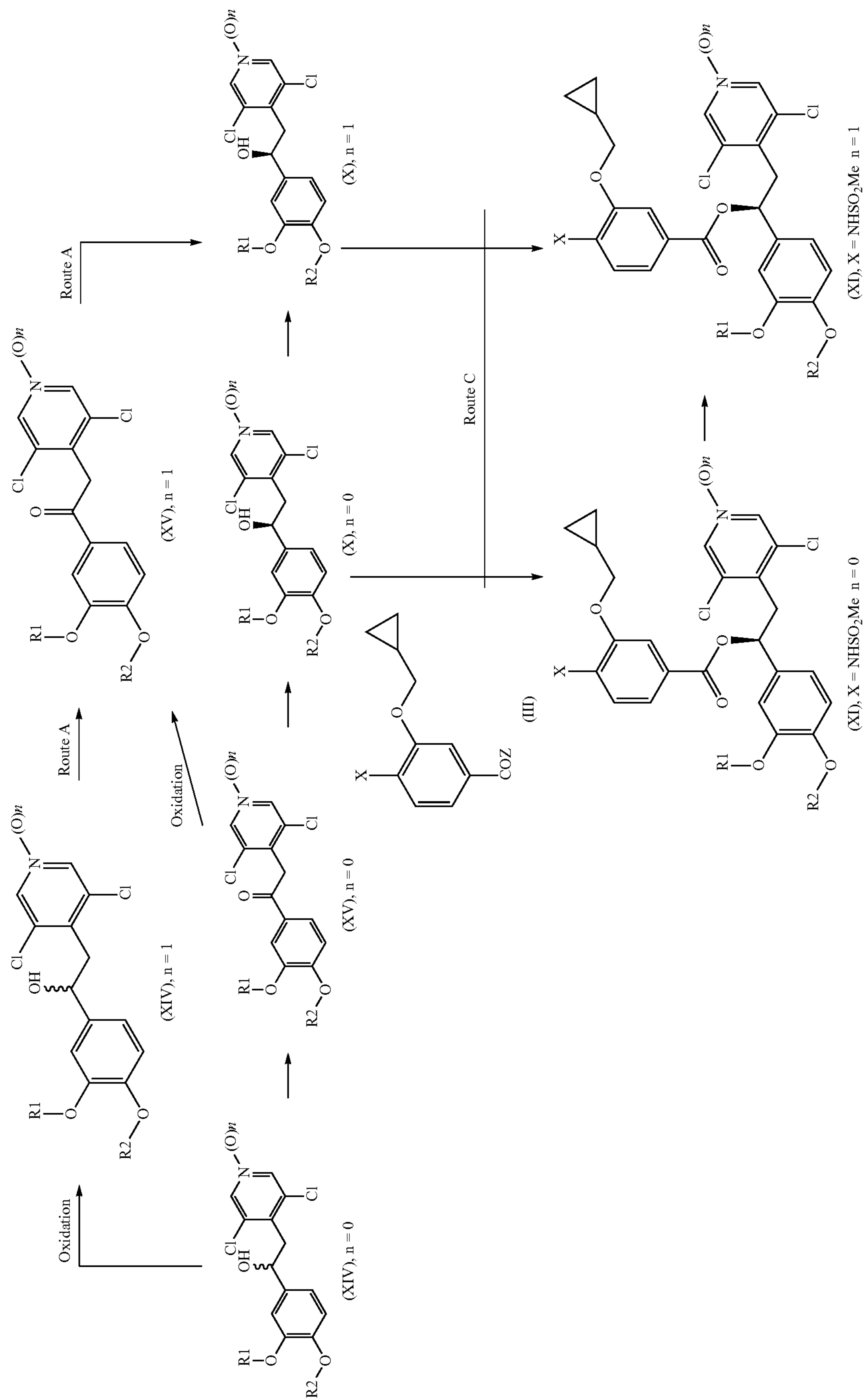
Scheme 5
