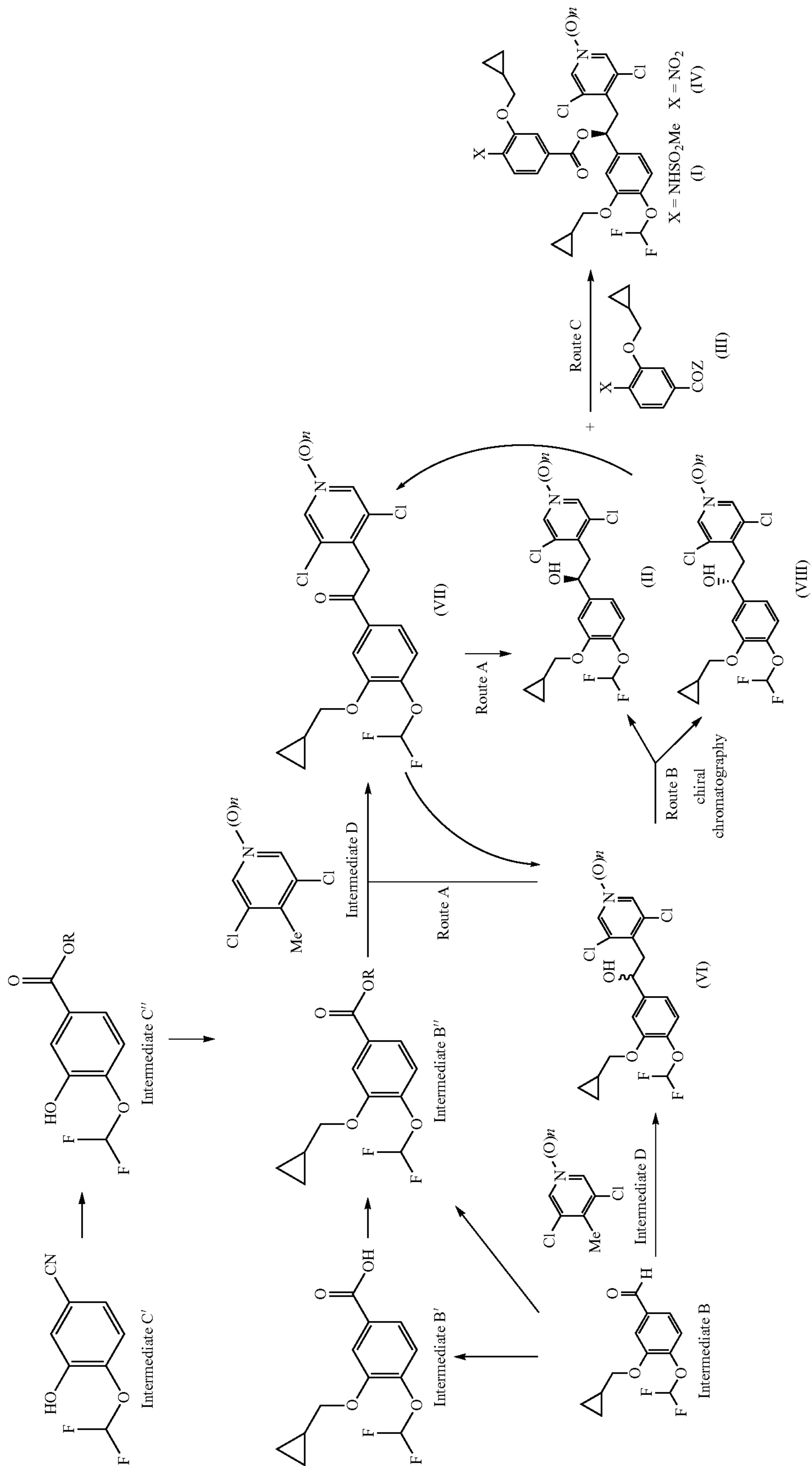
Scheme 1
