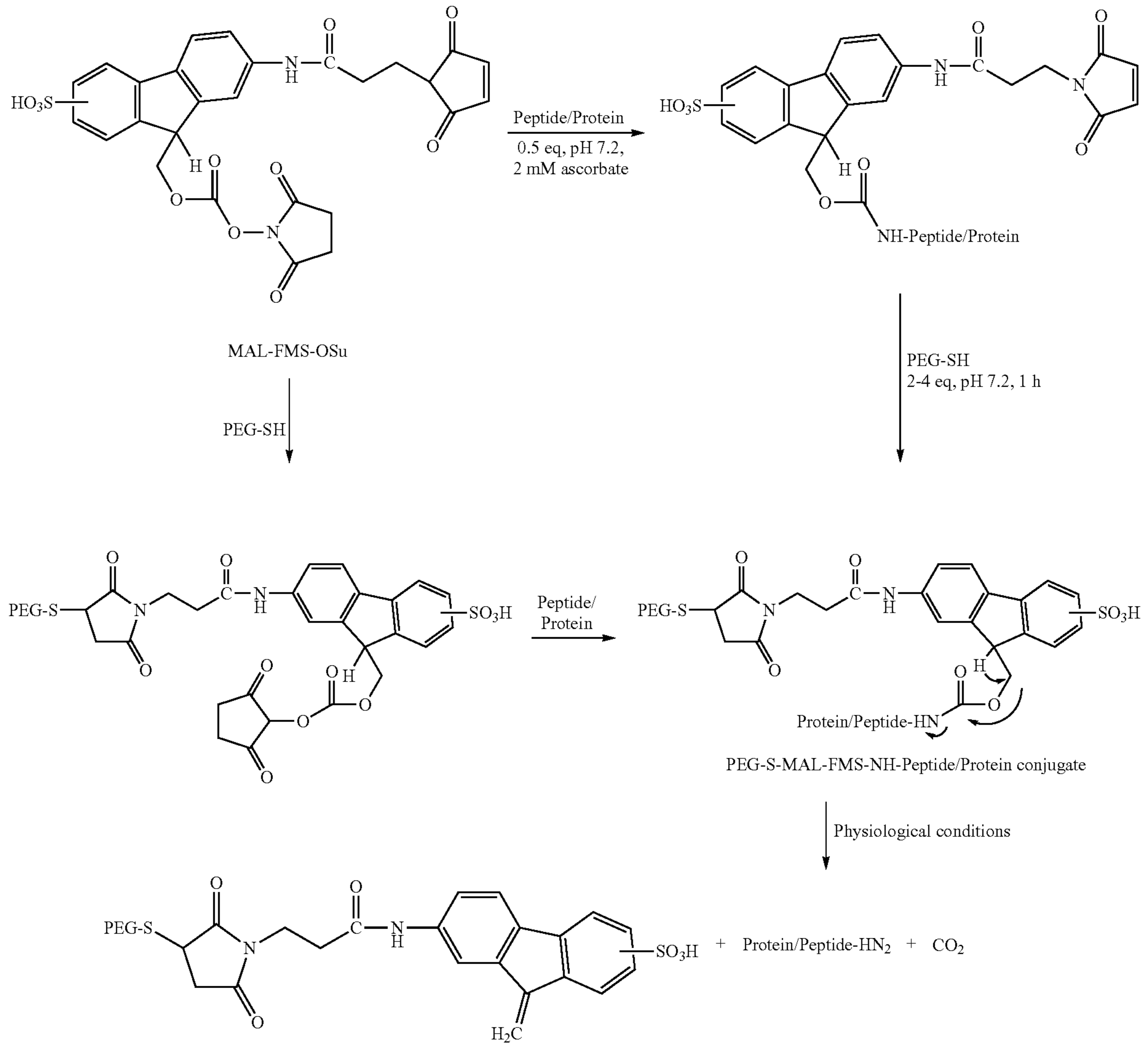
Scheme 6: Procedures for preparation of PEG-FMS-drugs
