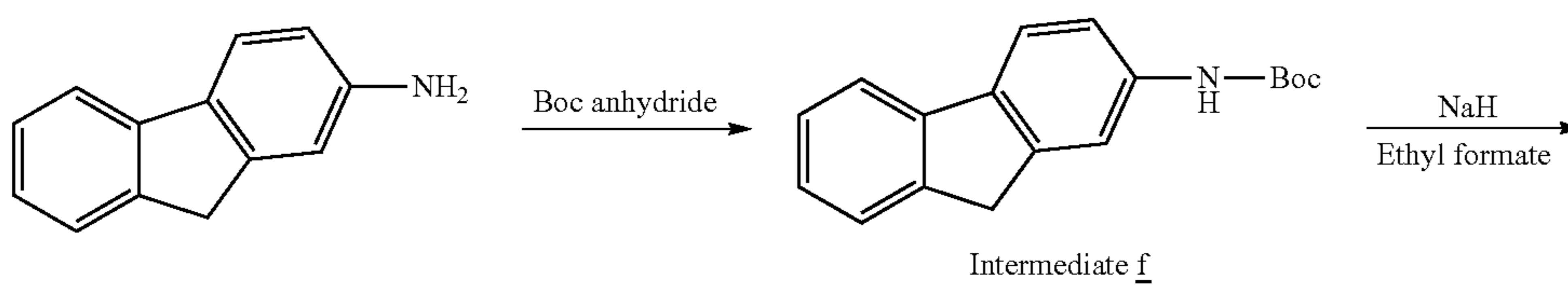
Scheme 2: Synthesis of Precursors 5
