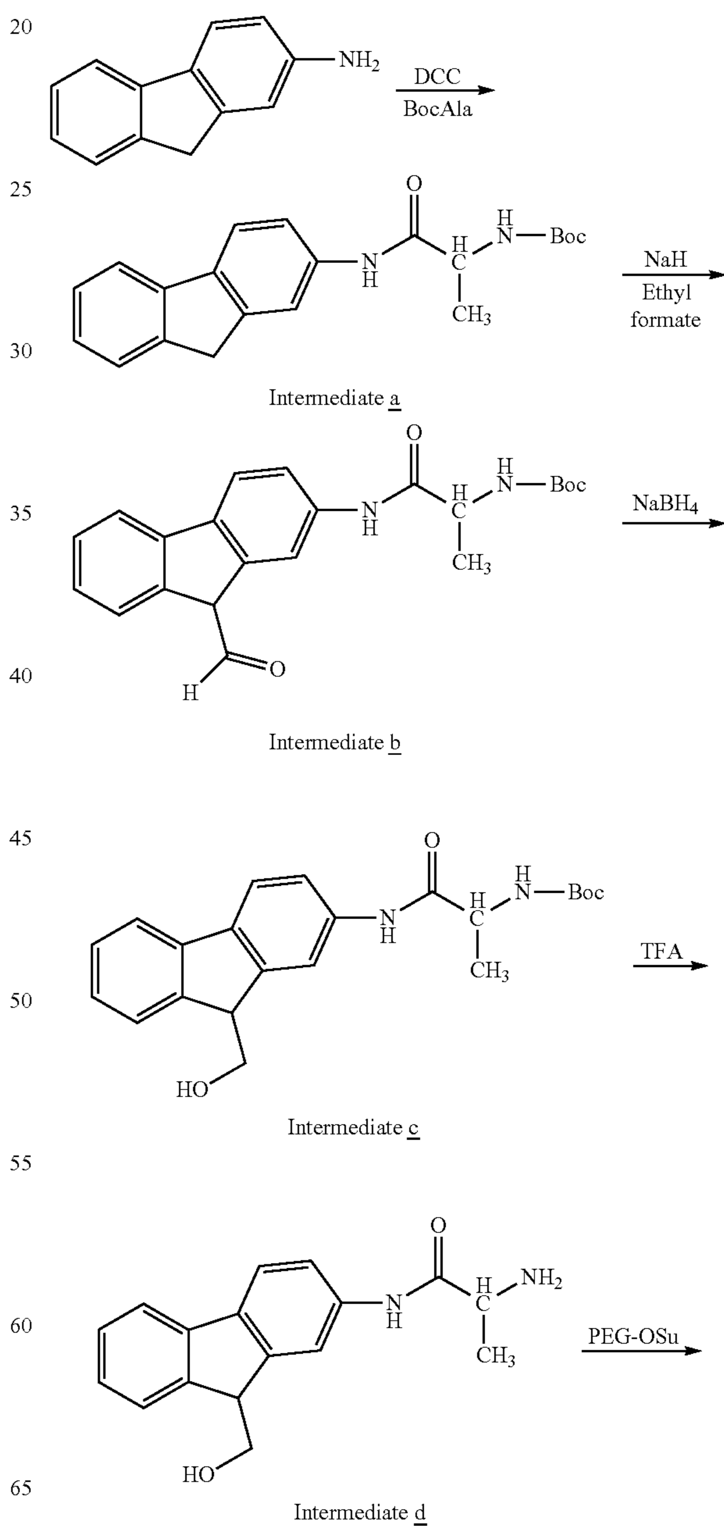
Scheme 2: Synthesis of Precursors 1-4
