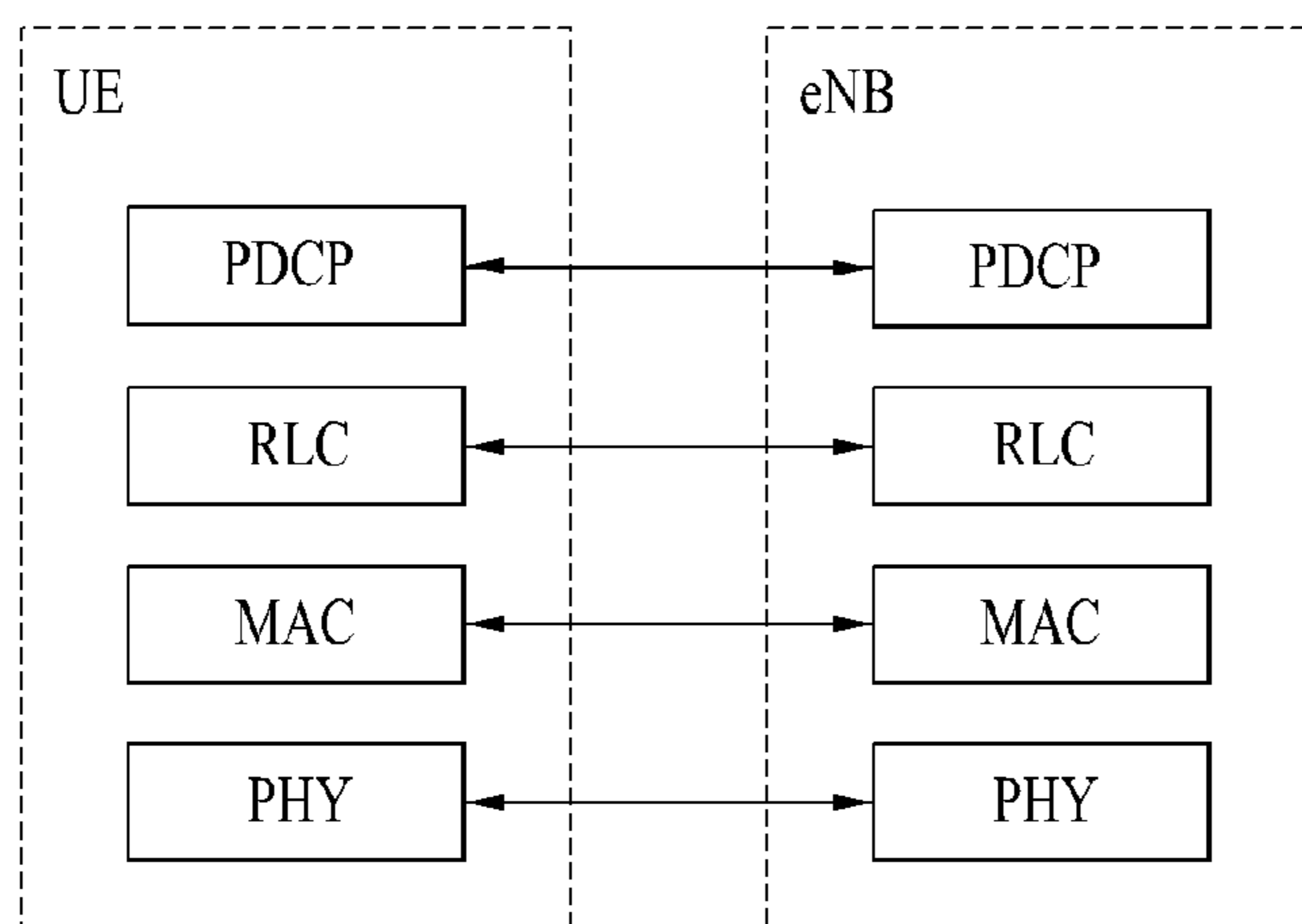
(b) User-Plane Protocol Stack
