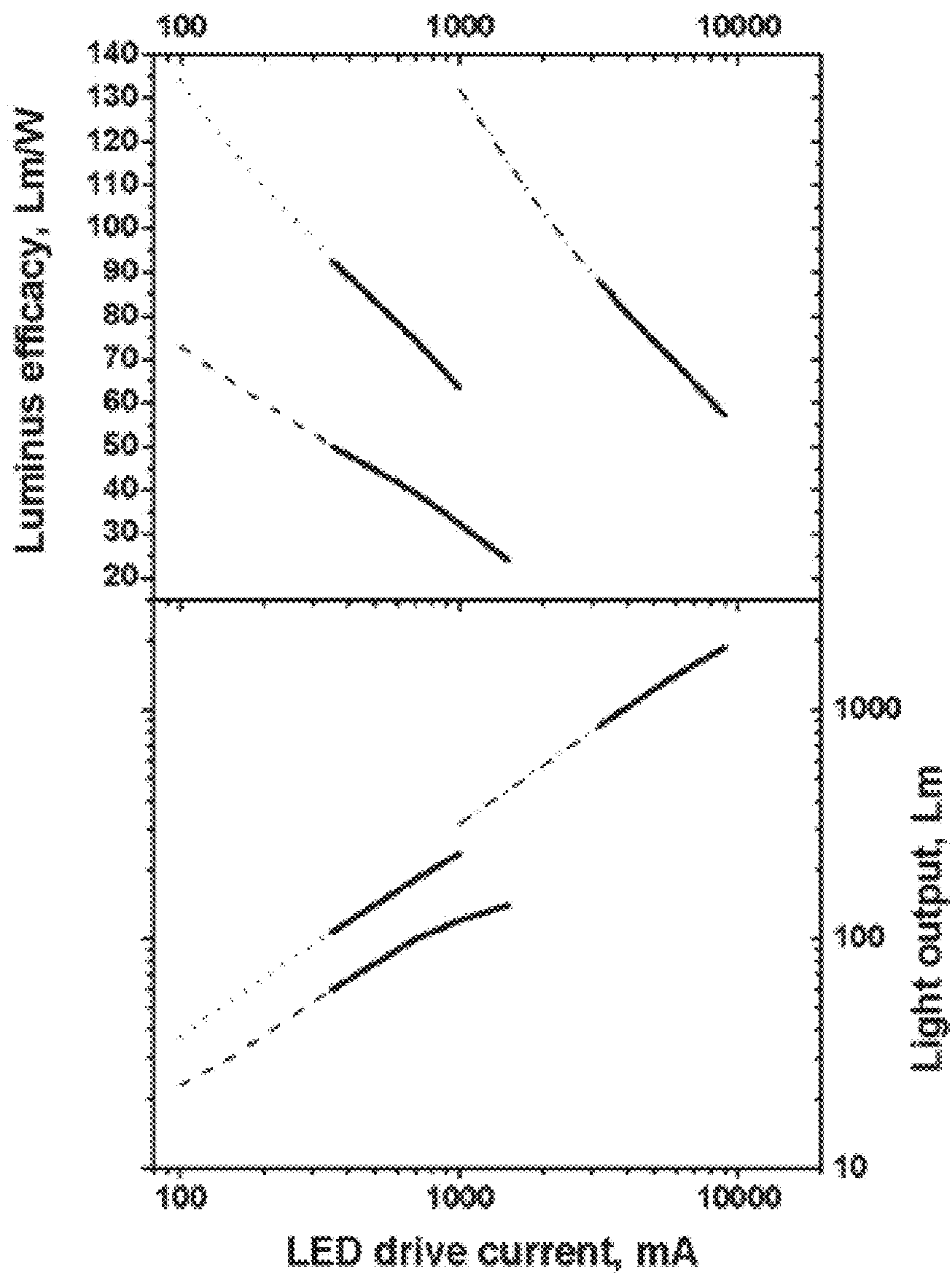
FIG. 1 (Prior Art)
