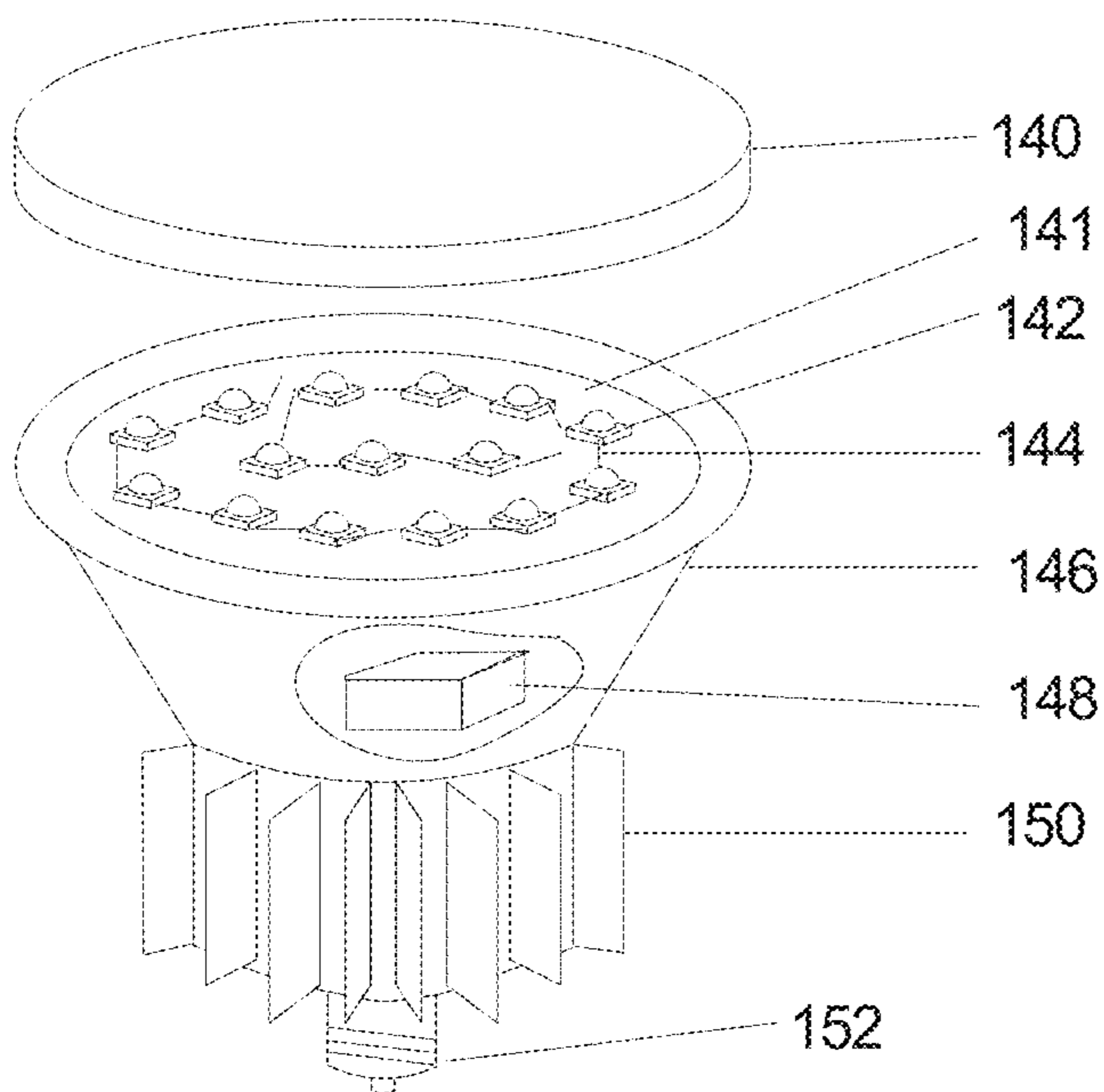
FIG. 4 (Prior Art)
