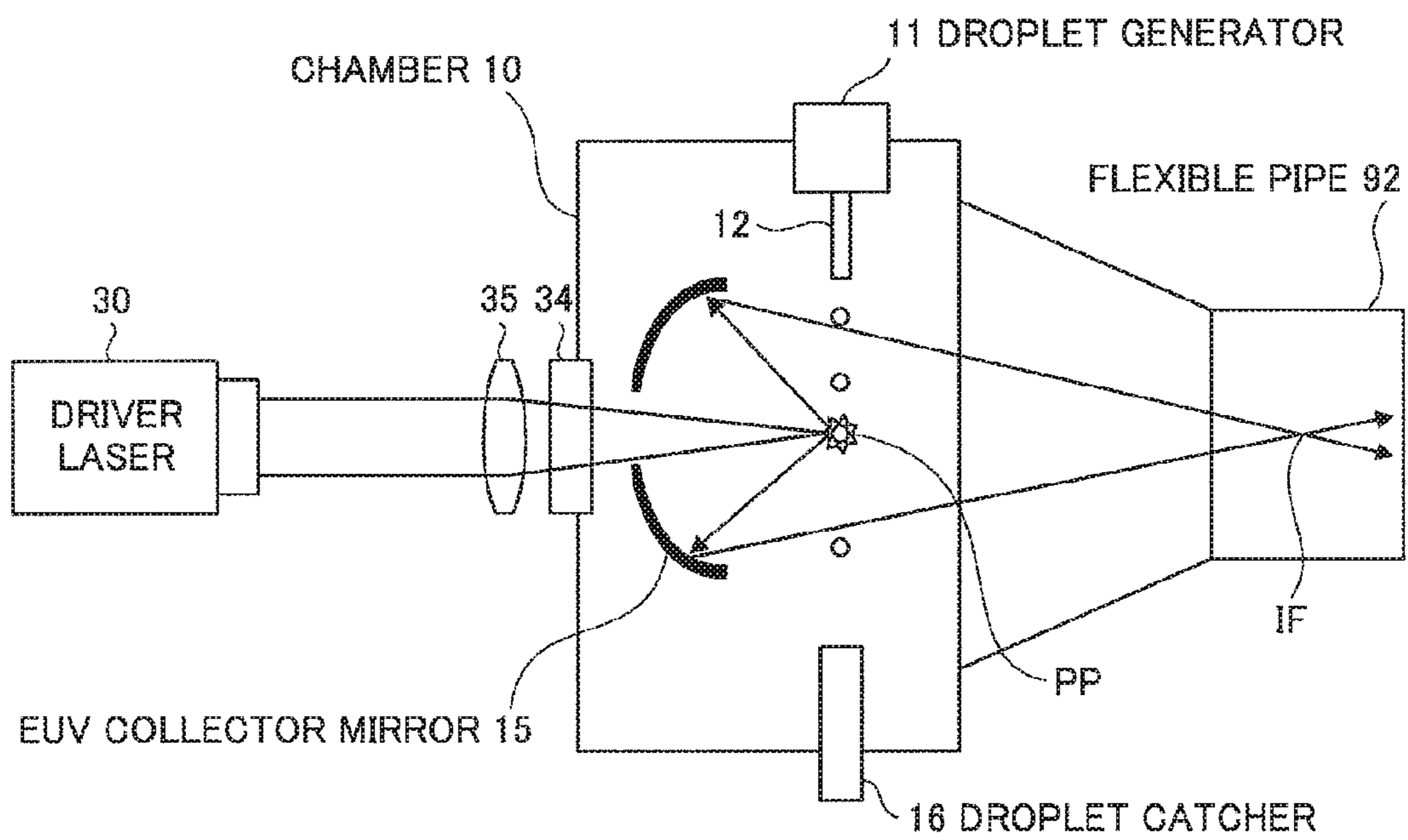
1 EUV LIGHT SOURCE APPARATUS
