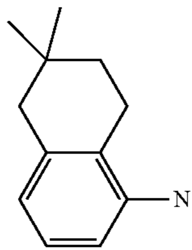
6,6-dimethyl-5,6,7,8-tetrahydronaphthalen-1-amine
