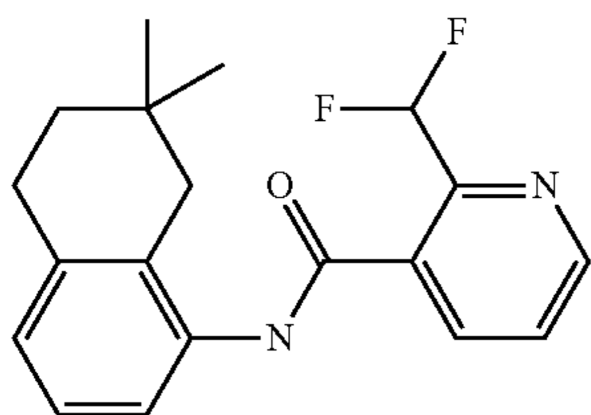
2-(difluoromethyl)-N-(7,7-dimethyl-5,6,7,8-tetrahydronaphthalen-1-yl)nicotinamide (example 1)
