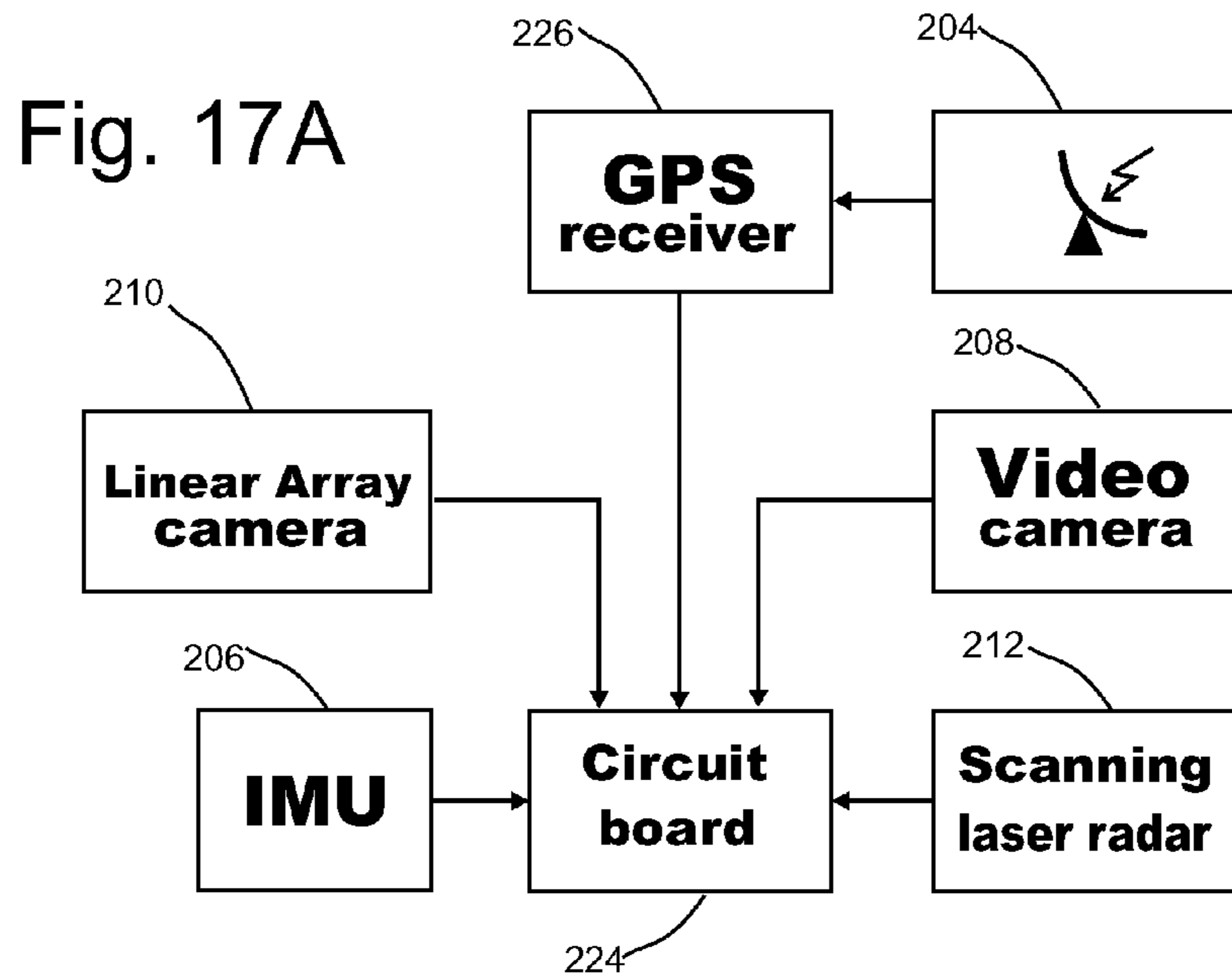
Data acquisition module
