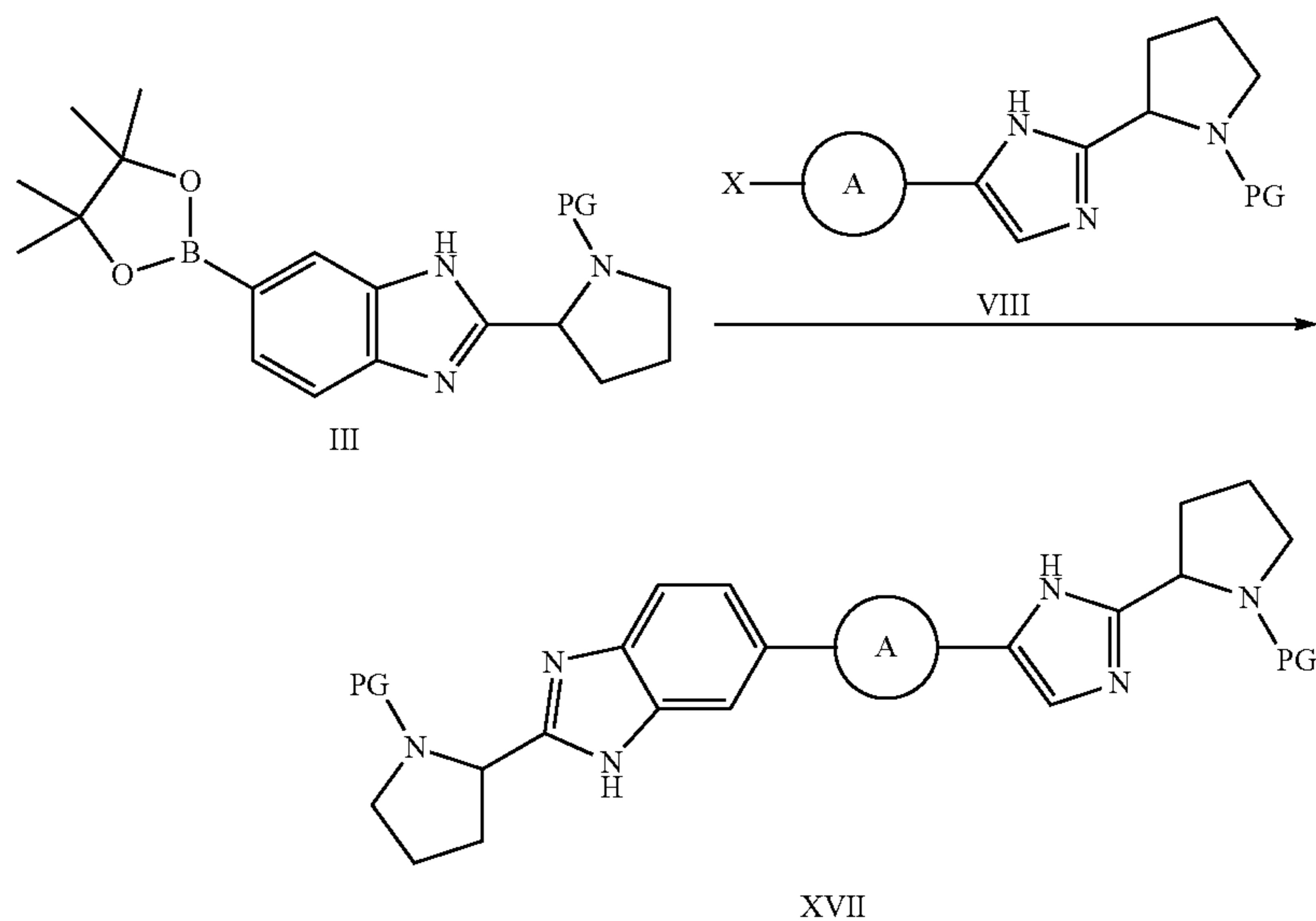
Scheme 4
