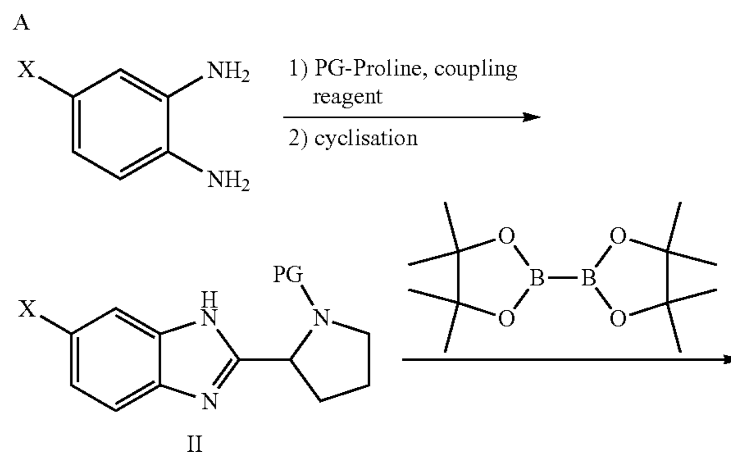
Scheme 1
