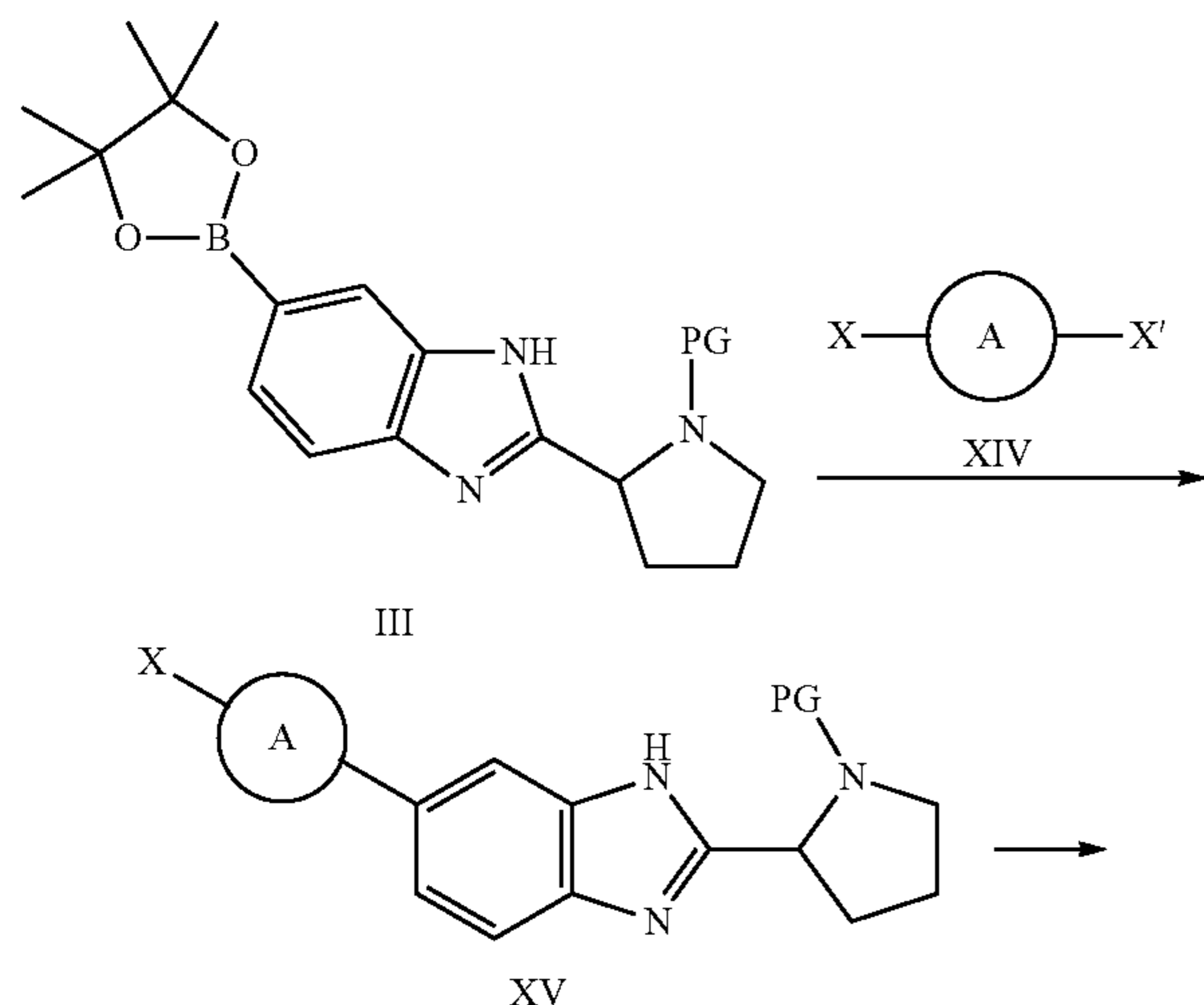
Scheme 3
