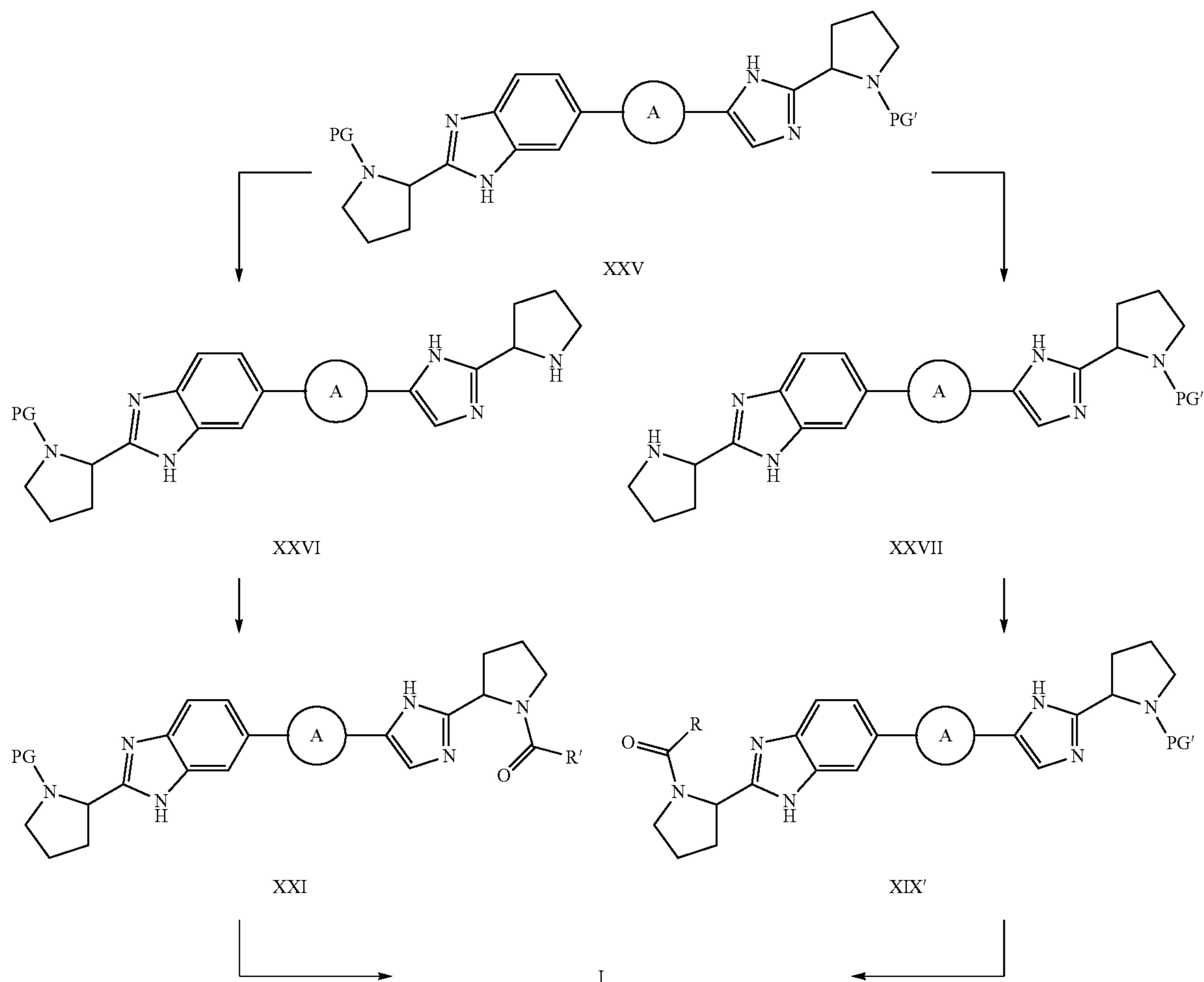
Scheme 7
