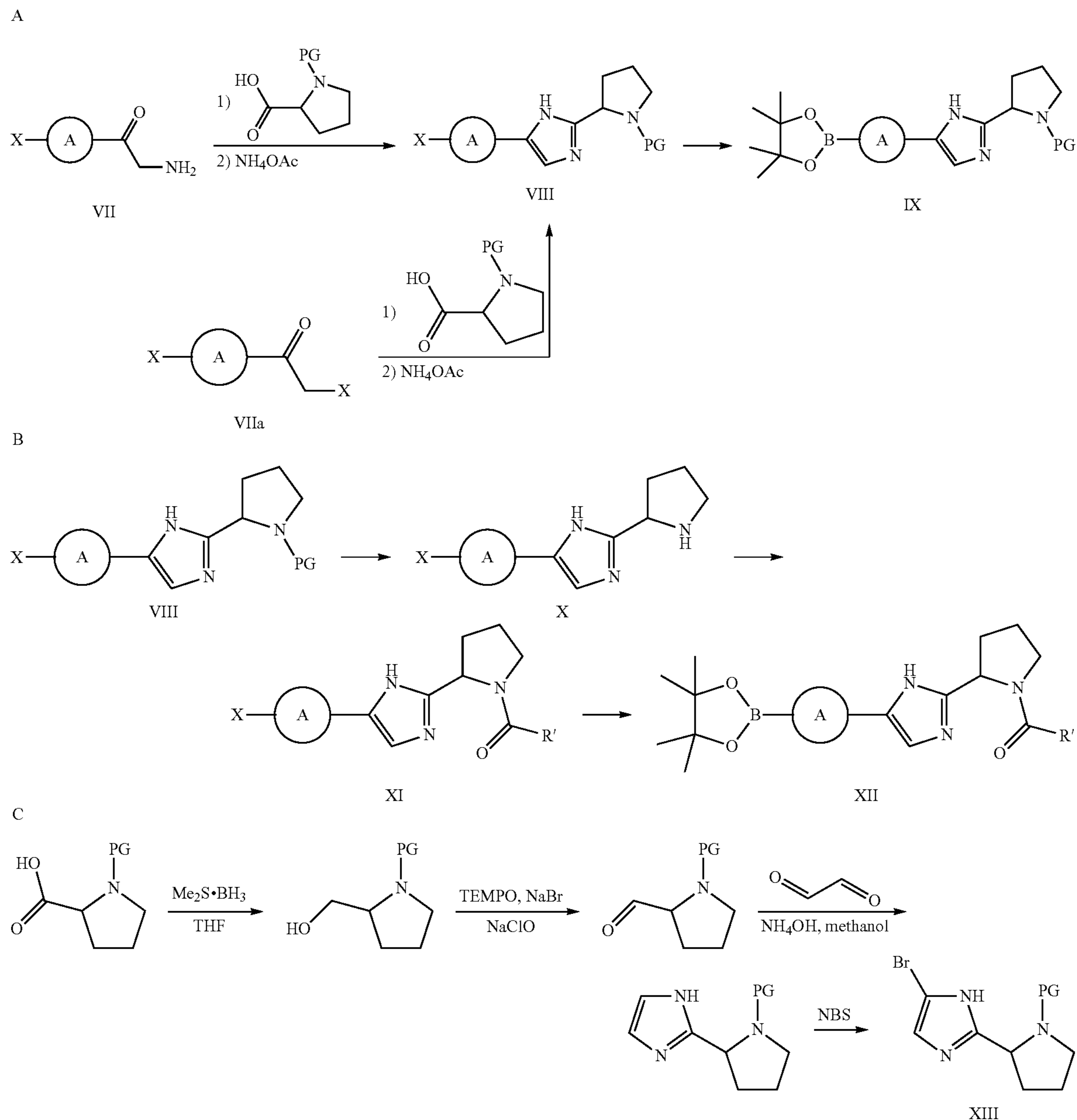
Scheme 2
