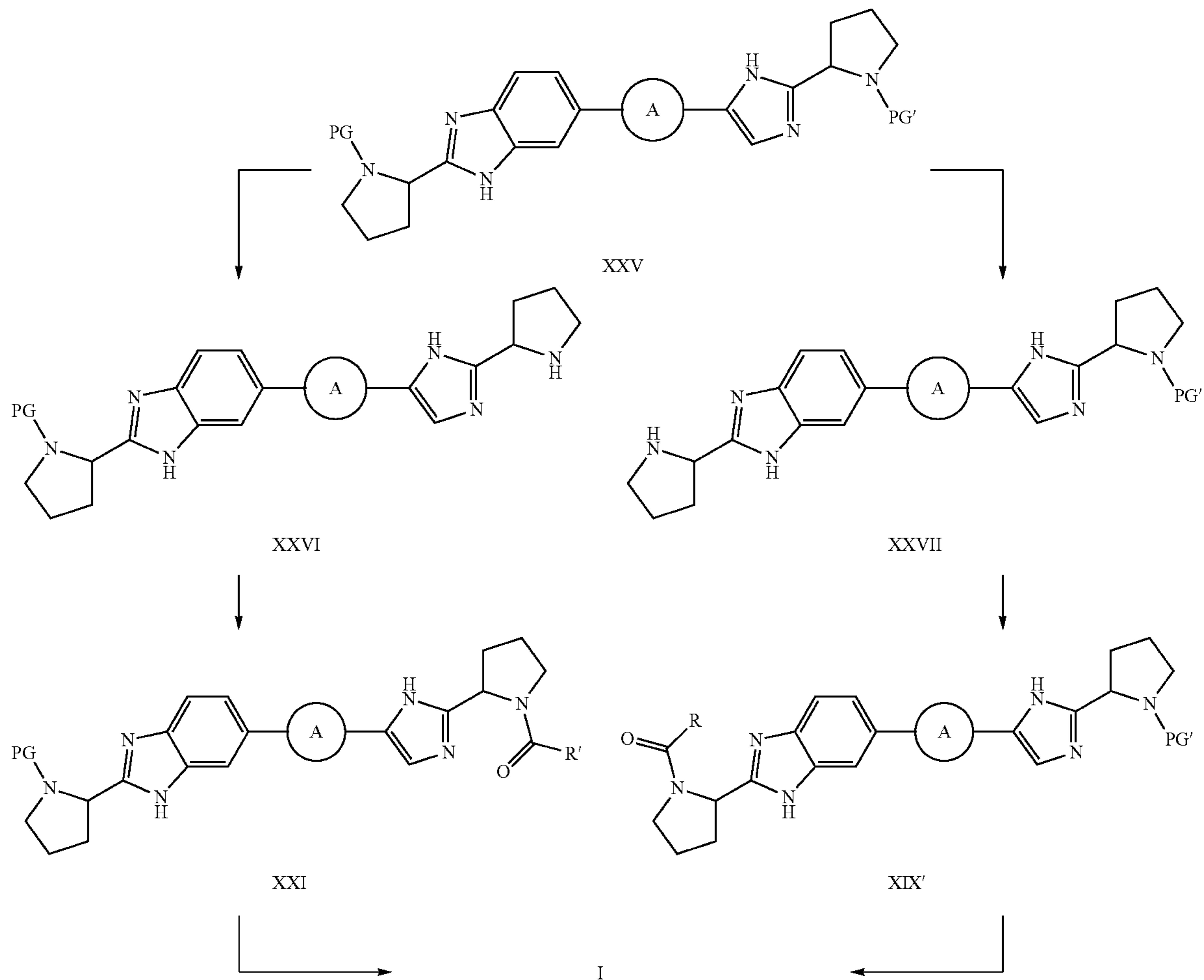
Scheme 7
