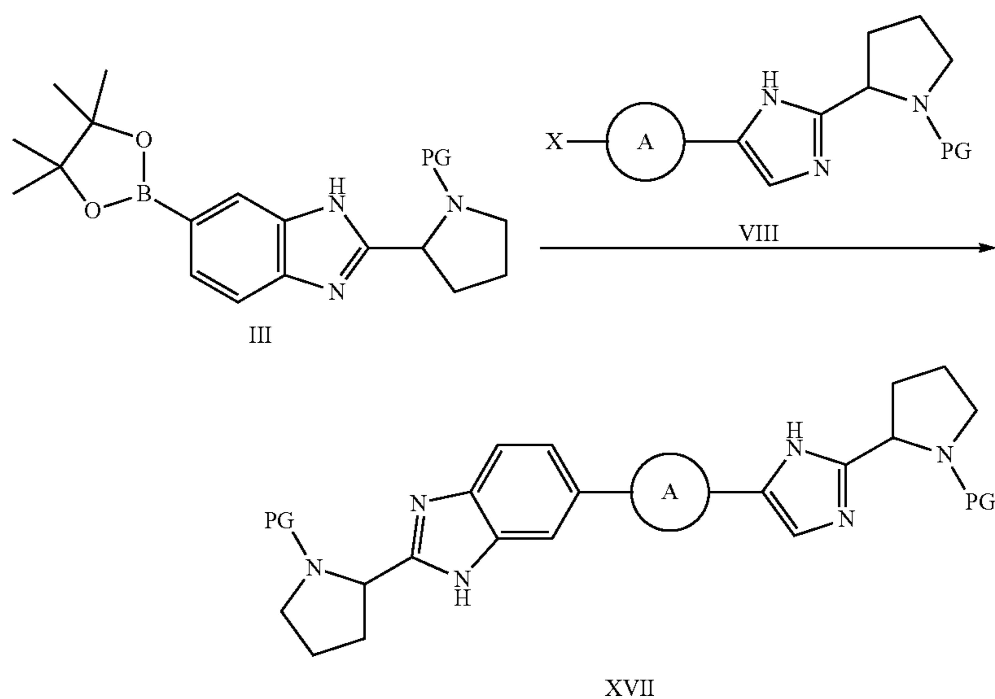
Scheme 4
