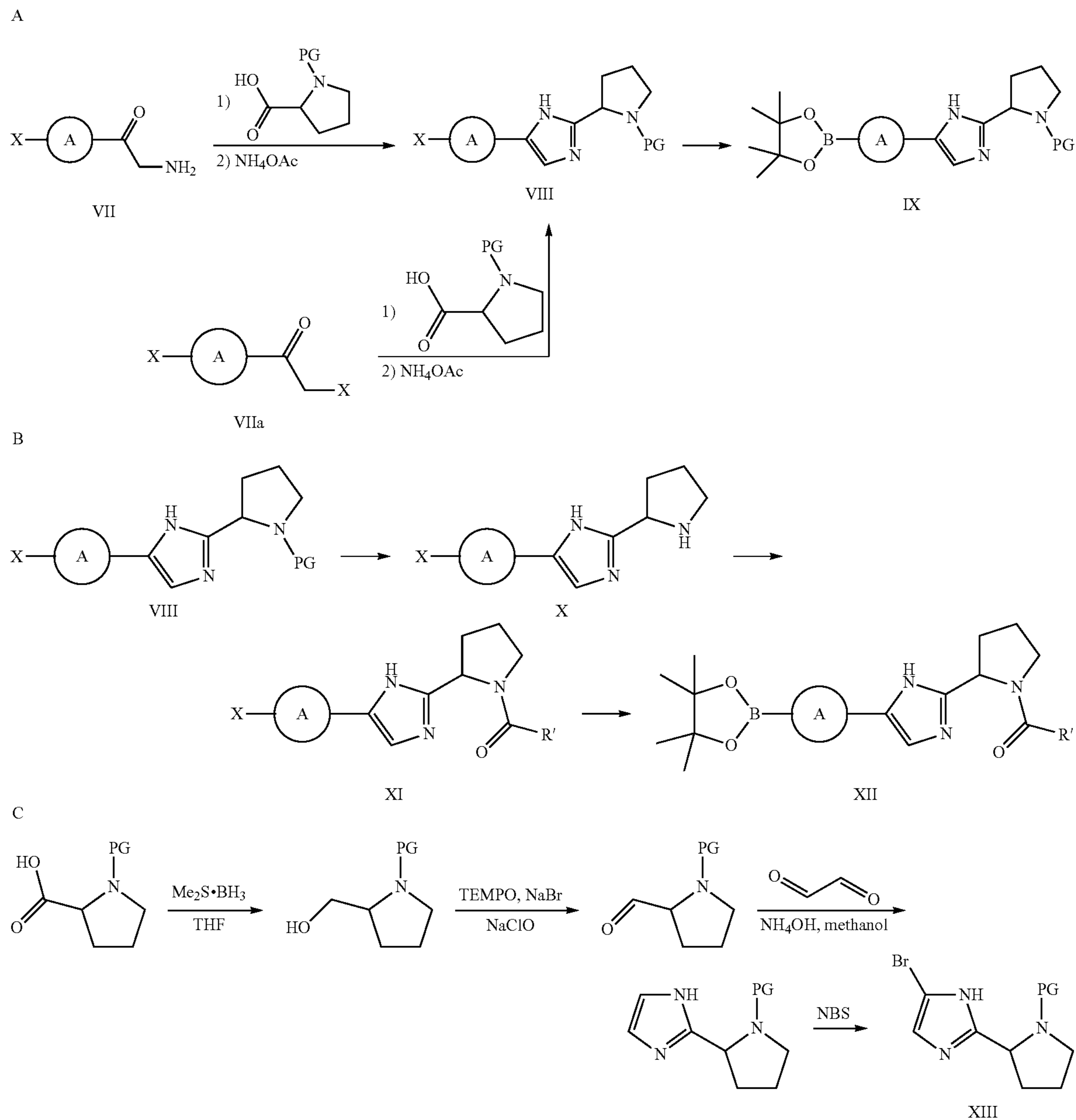
Scheme 2
