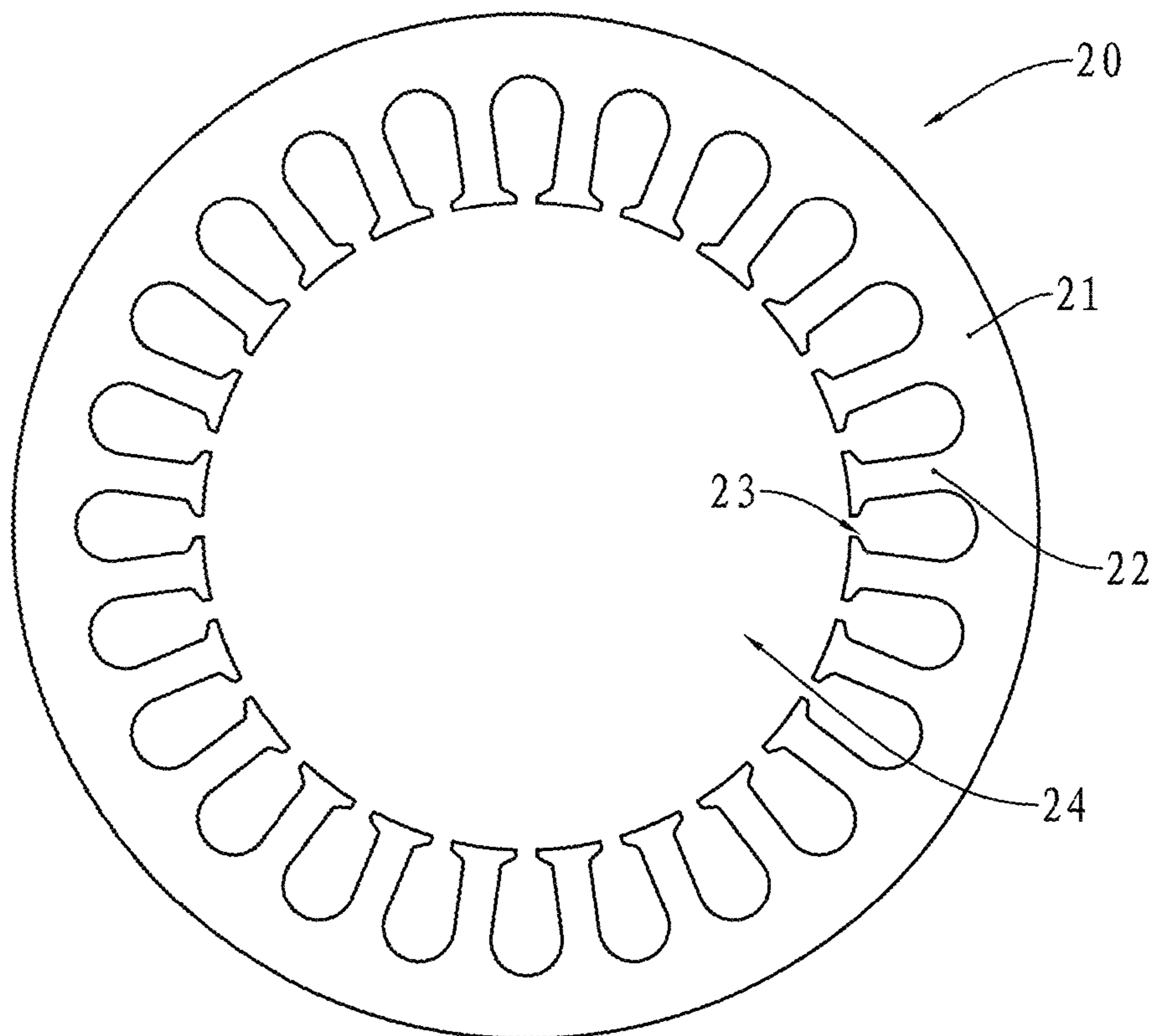
Fig. 2 Prior Art
