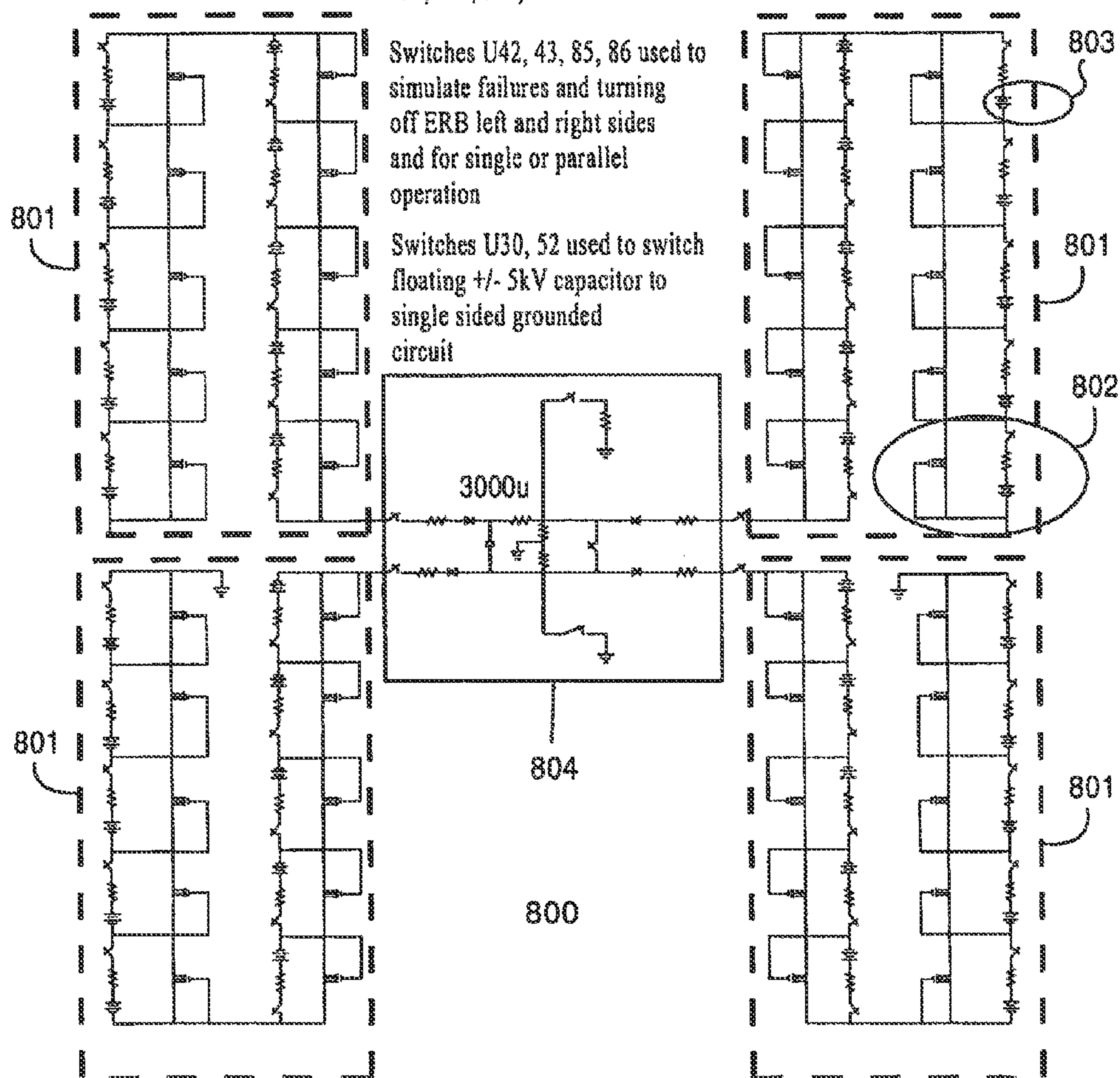
FIG. 8 H Configure ERB
