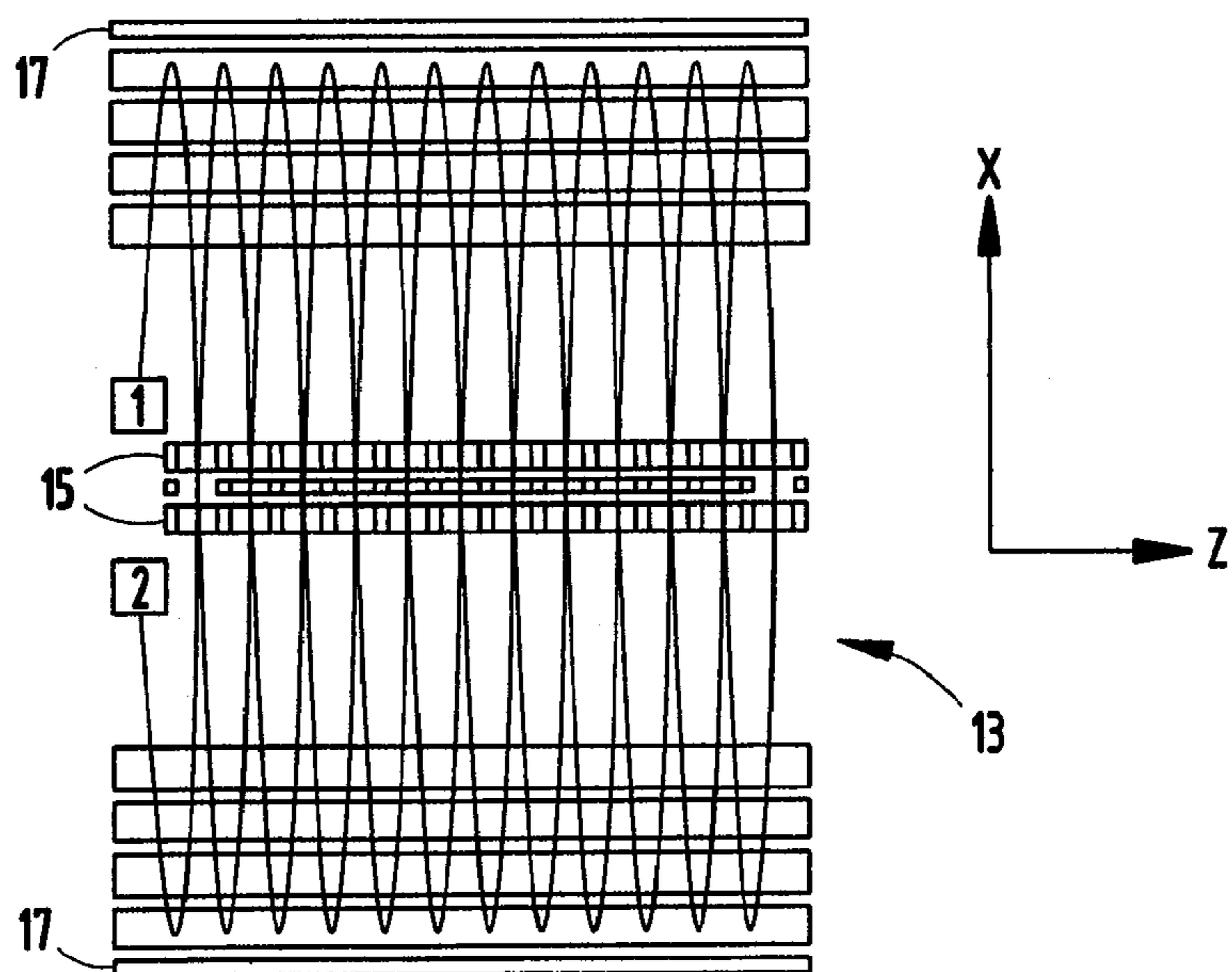
FIG. 3 (PRIOR ART)
