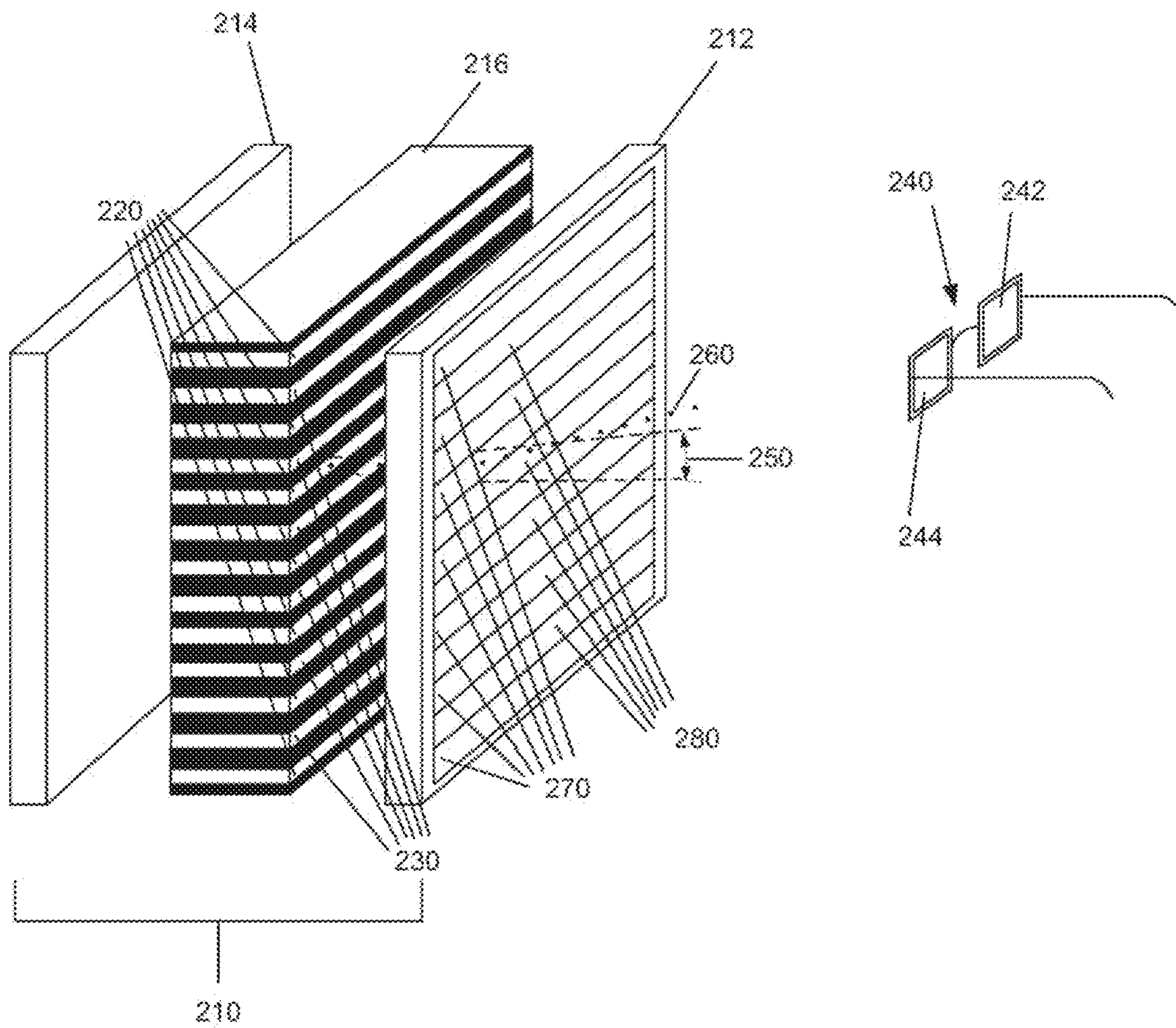
FIG. 2 (prior art)
