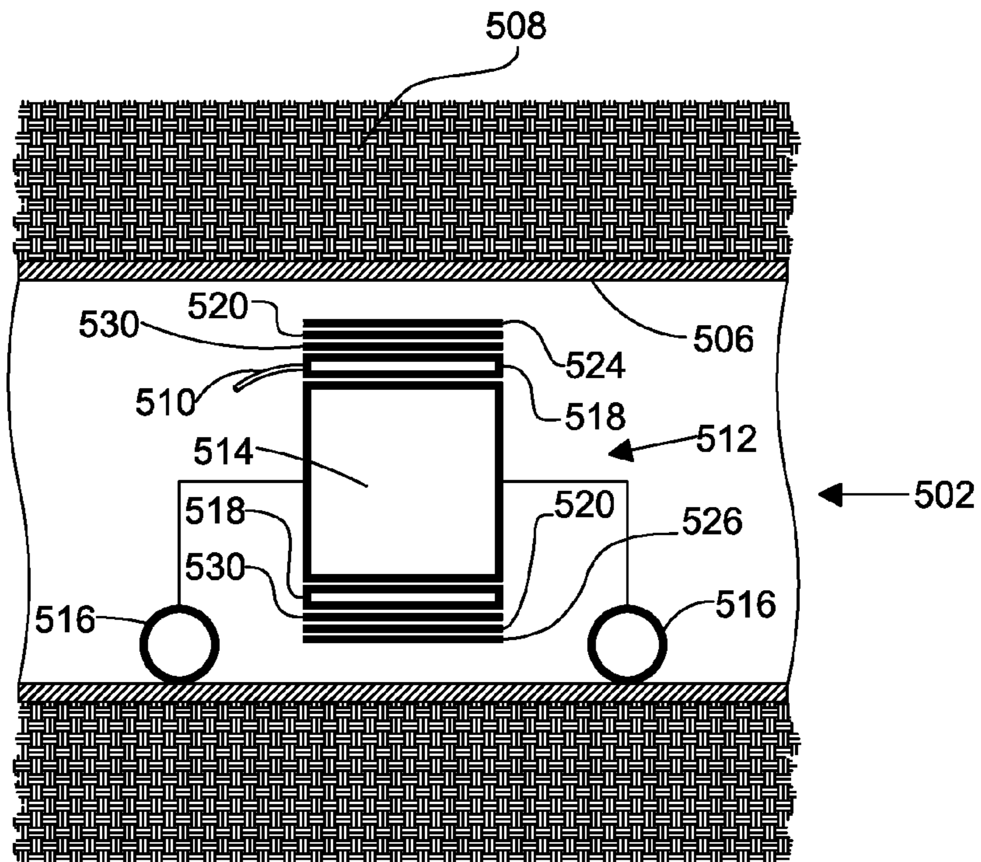
(A): Deflated Packer
