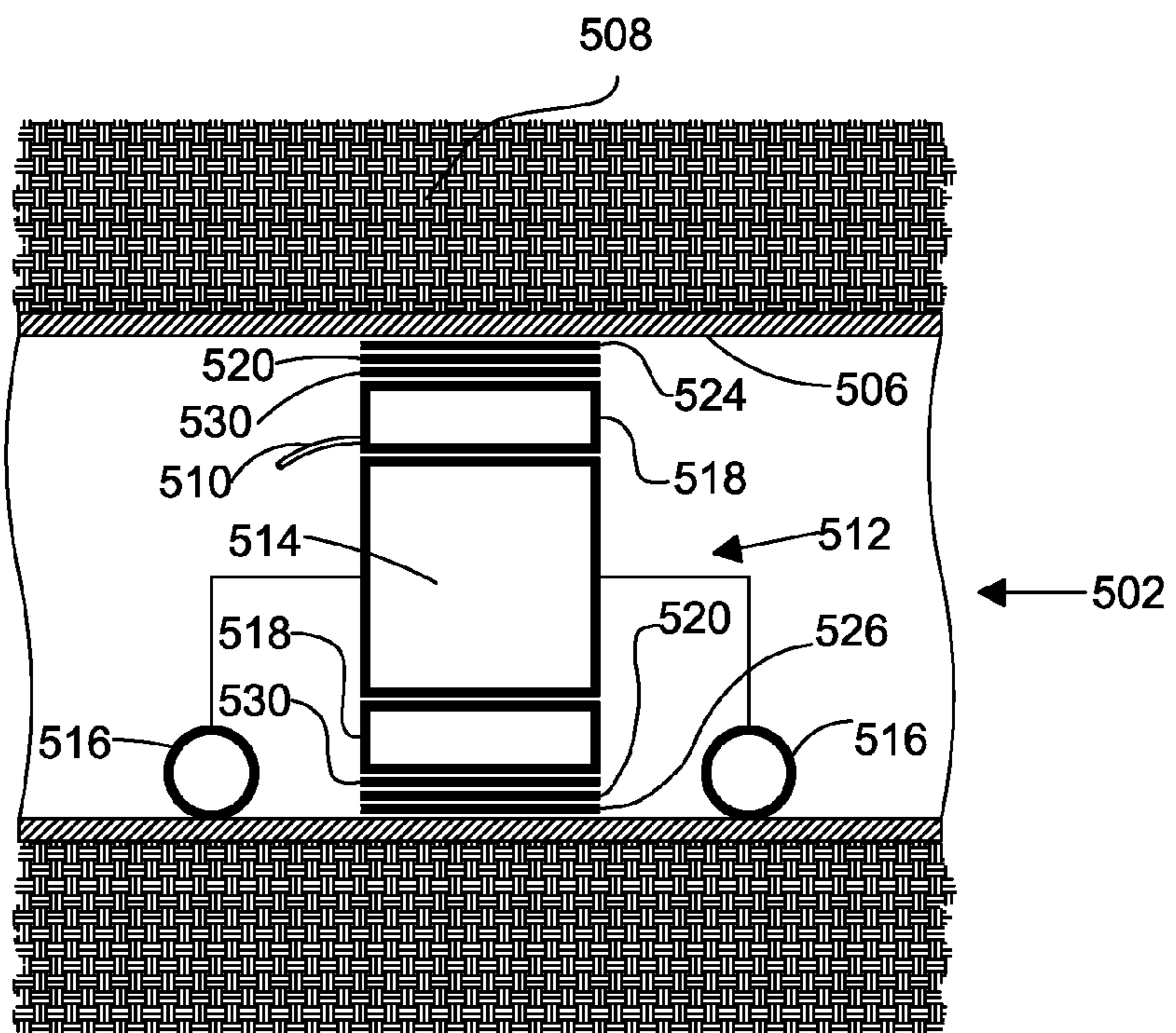
(B): Inflated Packer
