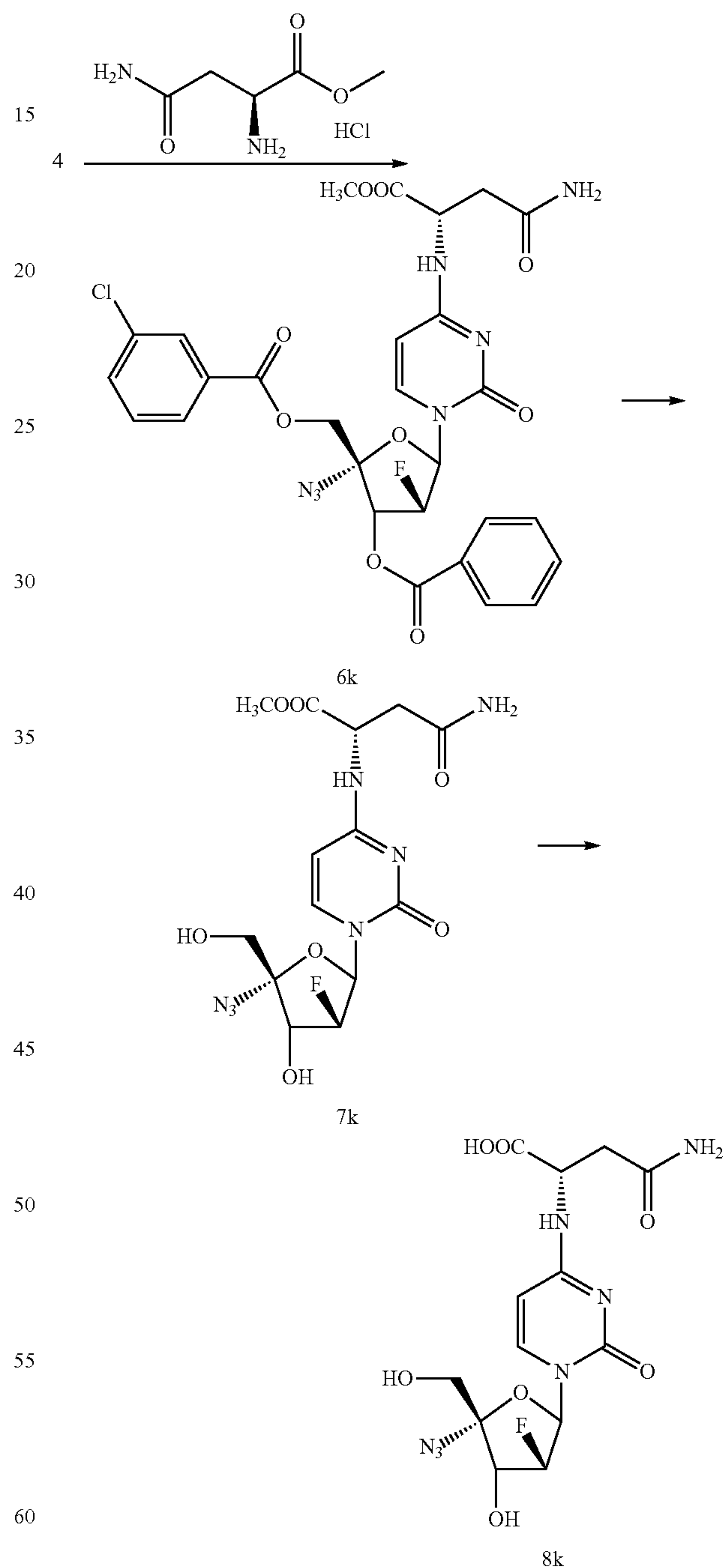
Scheme N. Synthesis of a pyrimidine nucleoside derivative with amino acid substitution at position 4.
