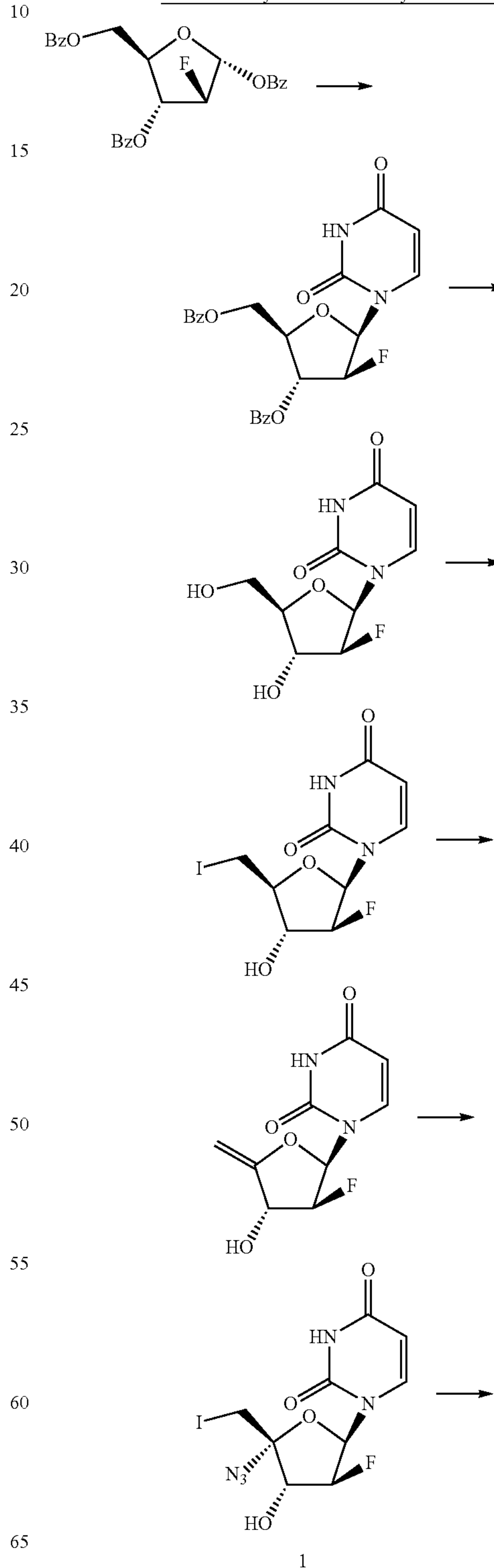
Scheme A. Synthesis of the key intermediate 3
