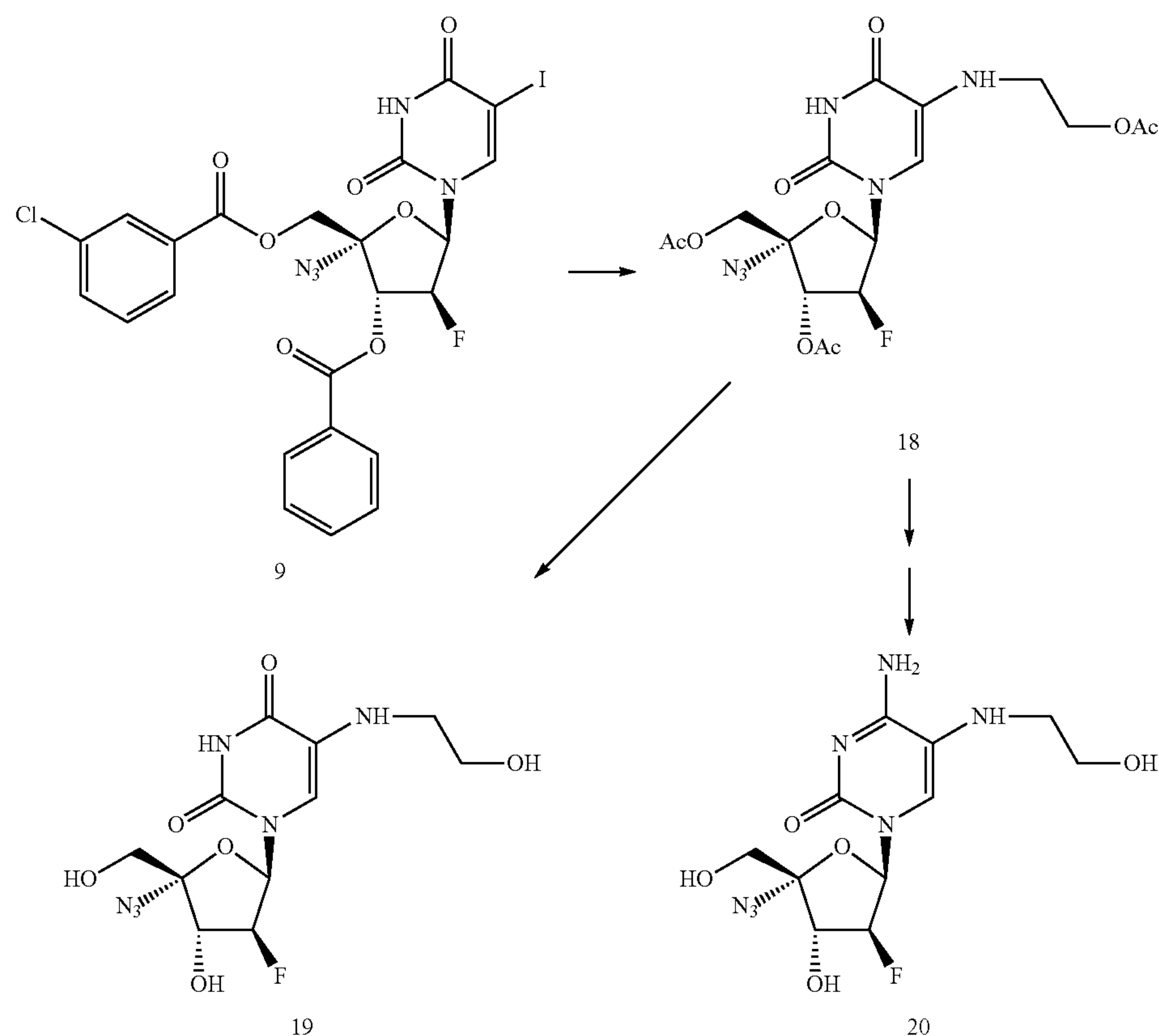
Scheme T. Synthesis of a pyrimidine nucleoside derivative with amino substitution at position 5.
