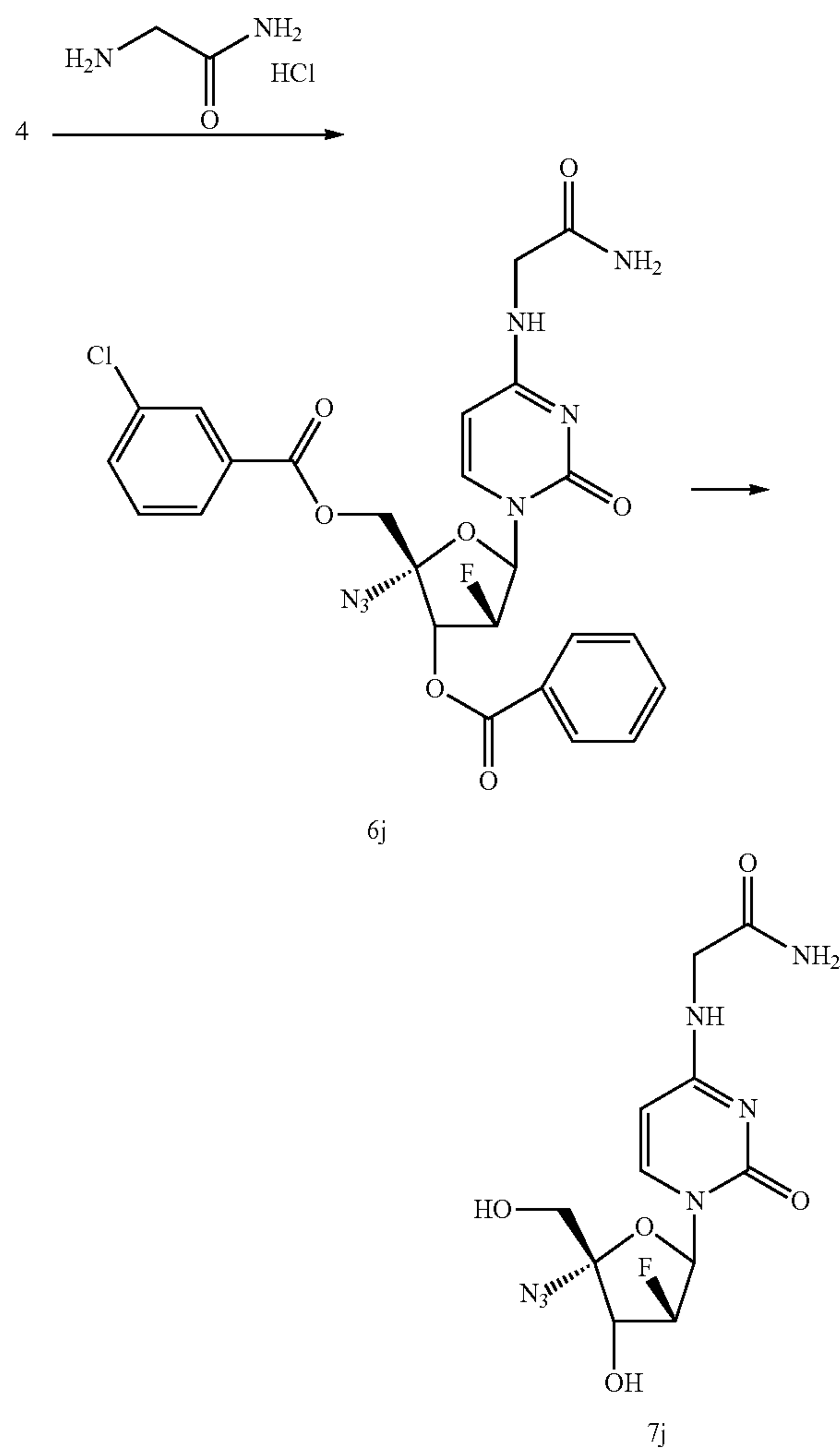
Scheme M. Synthesis of a pyrimidine nucleoside derivative with amino acid substitution at position 4.
