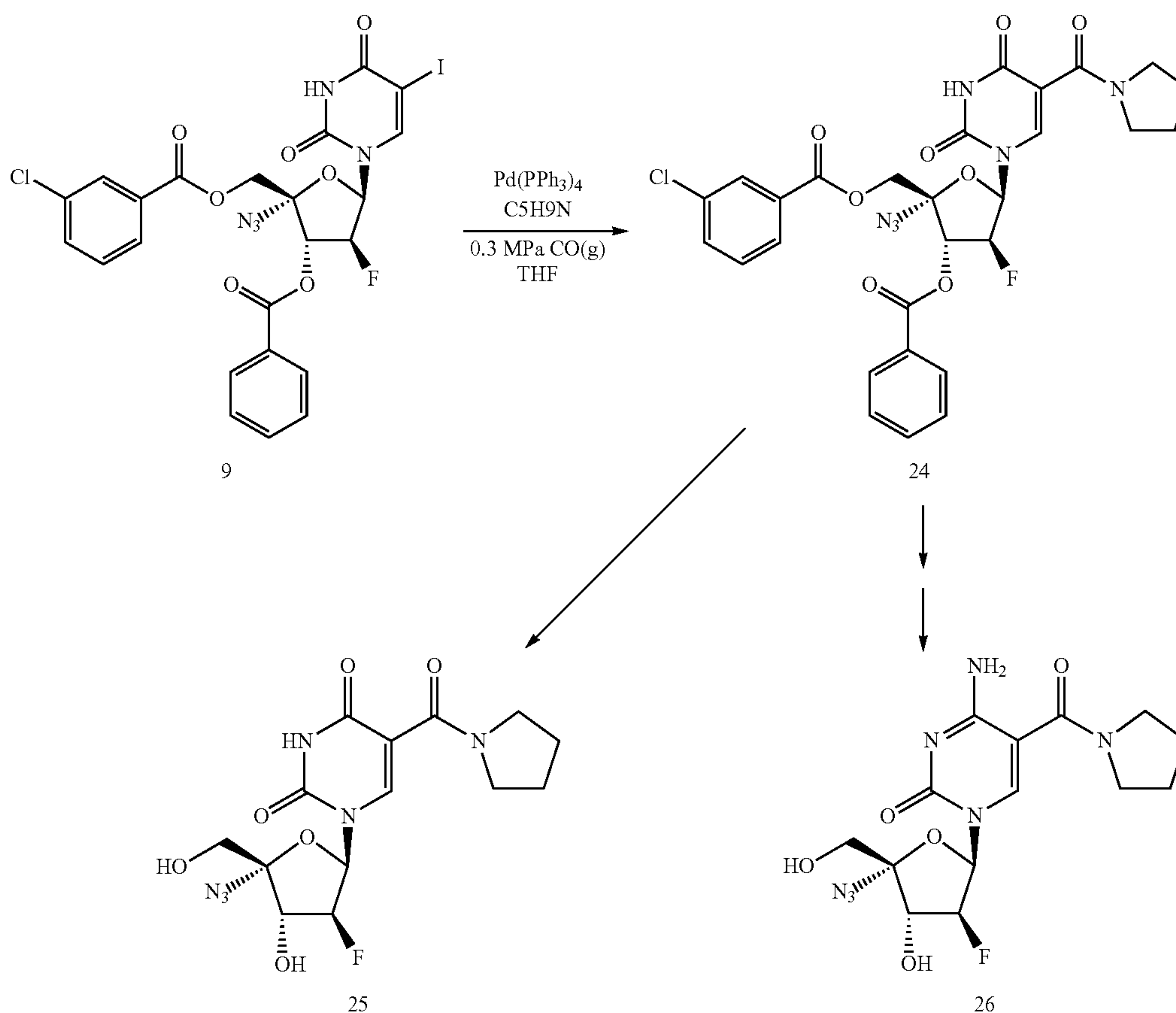
Scheme V. Synthesis of a pyrimidine nucleoside derivative with amidation at position 5.
