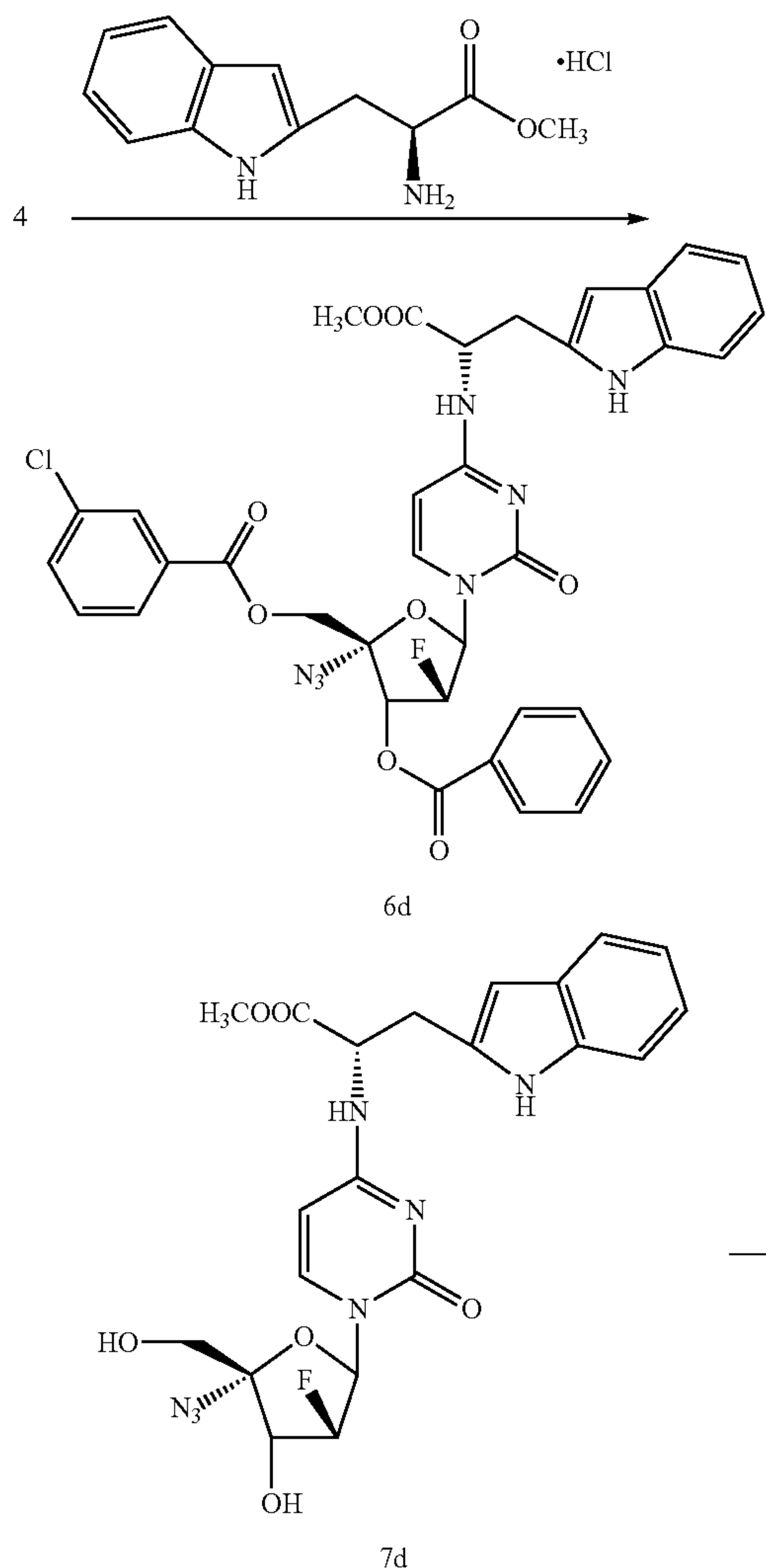
Scheme G. Synthesis of a pyrimidine nucleoside derivative with amino acid substitution at position 4.
