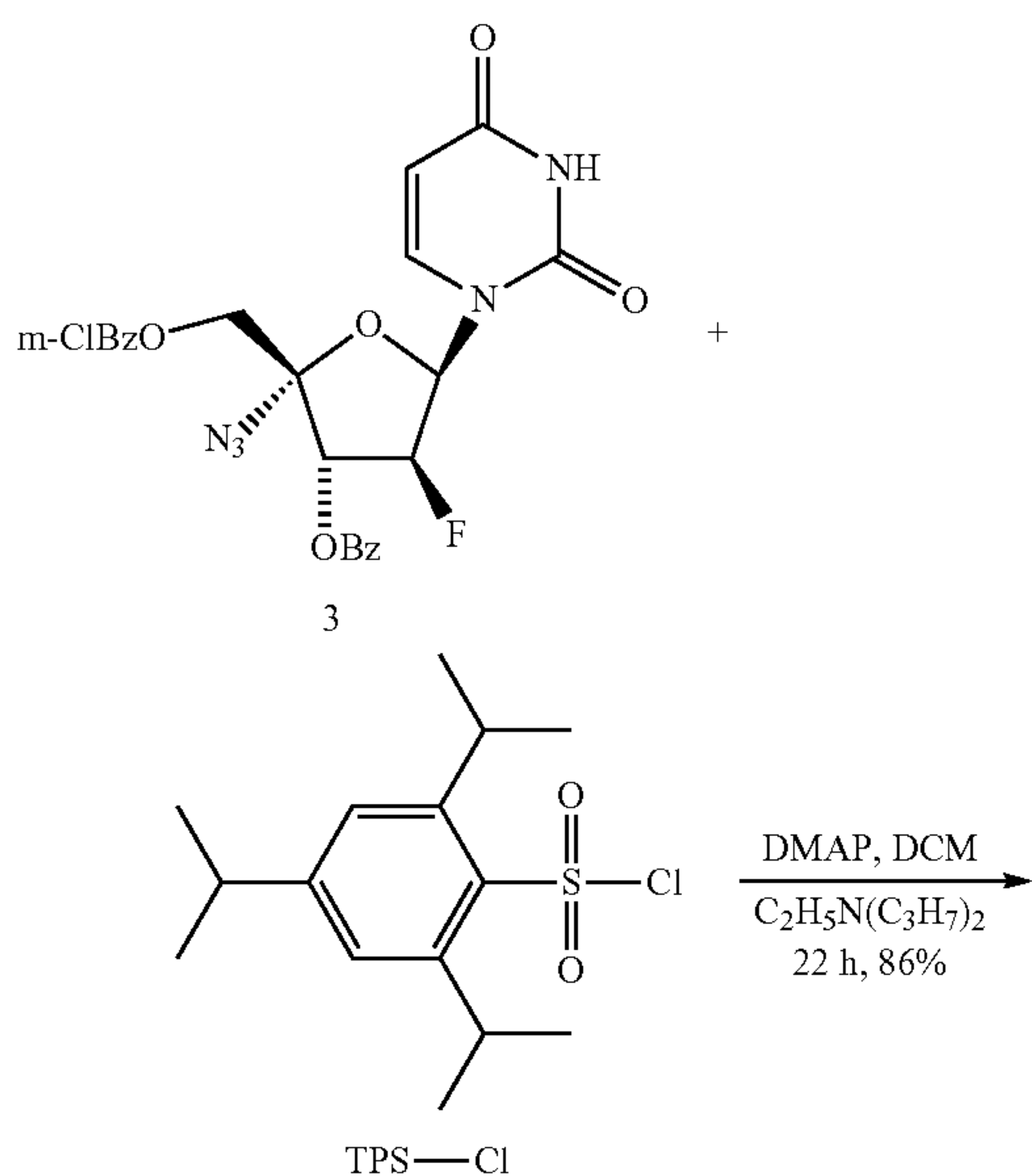
Scheme B. Synthesis of an active intermediate
