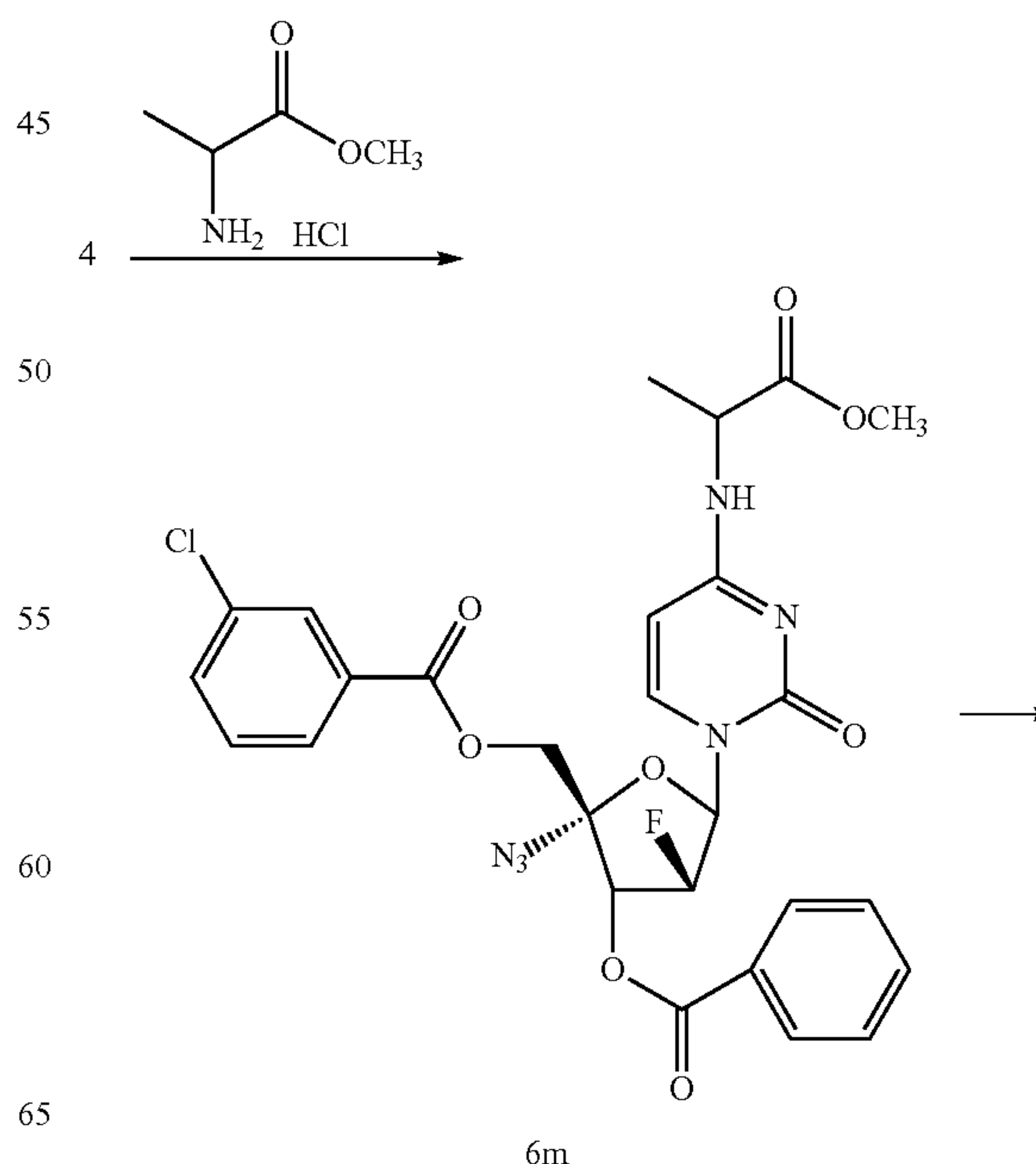
Scheme P. Synthesis of a pyrimidine nucleoside derivative with amino acid substitution at position 4.
