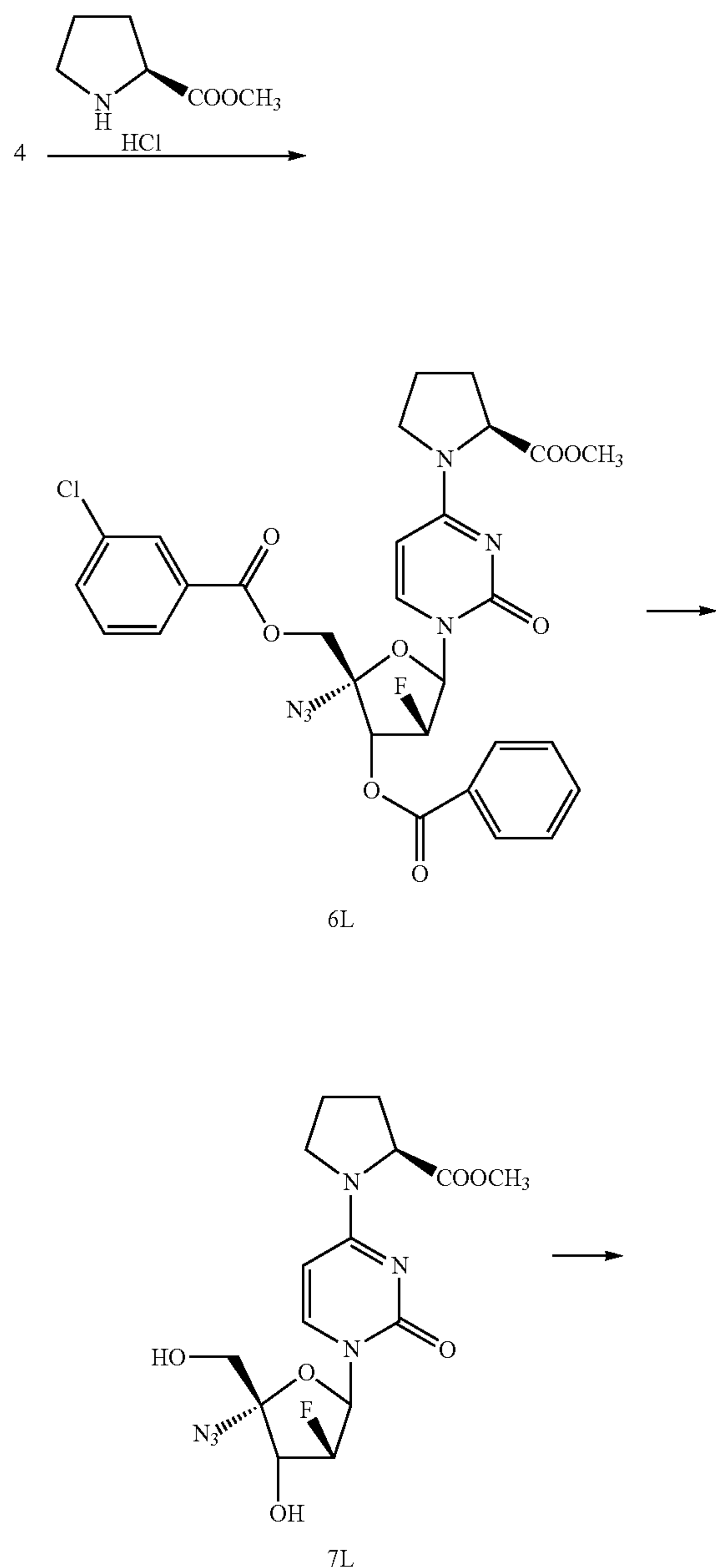
Scheme O. Synthesis of a pyrimidine nucleoside derivative with amino acid substitution at position 4.
