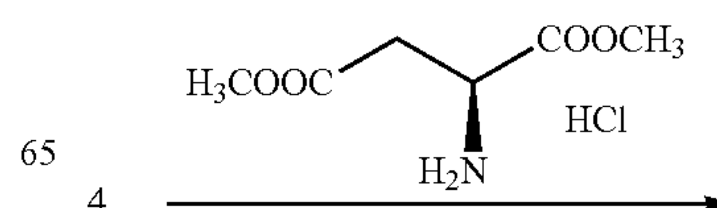
Scheme H. Synthesis of a pyrimidine nucleoside derivative with amino acid substitution at position 4.
