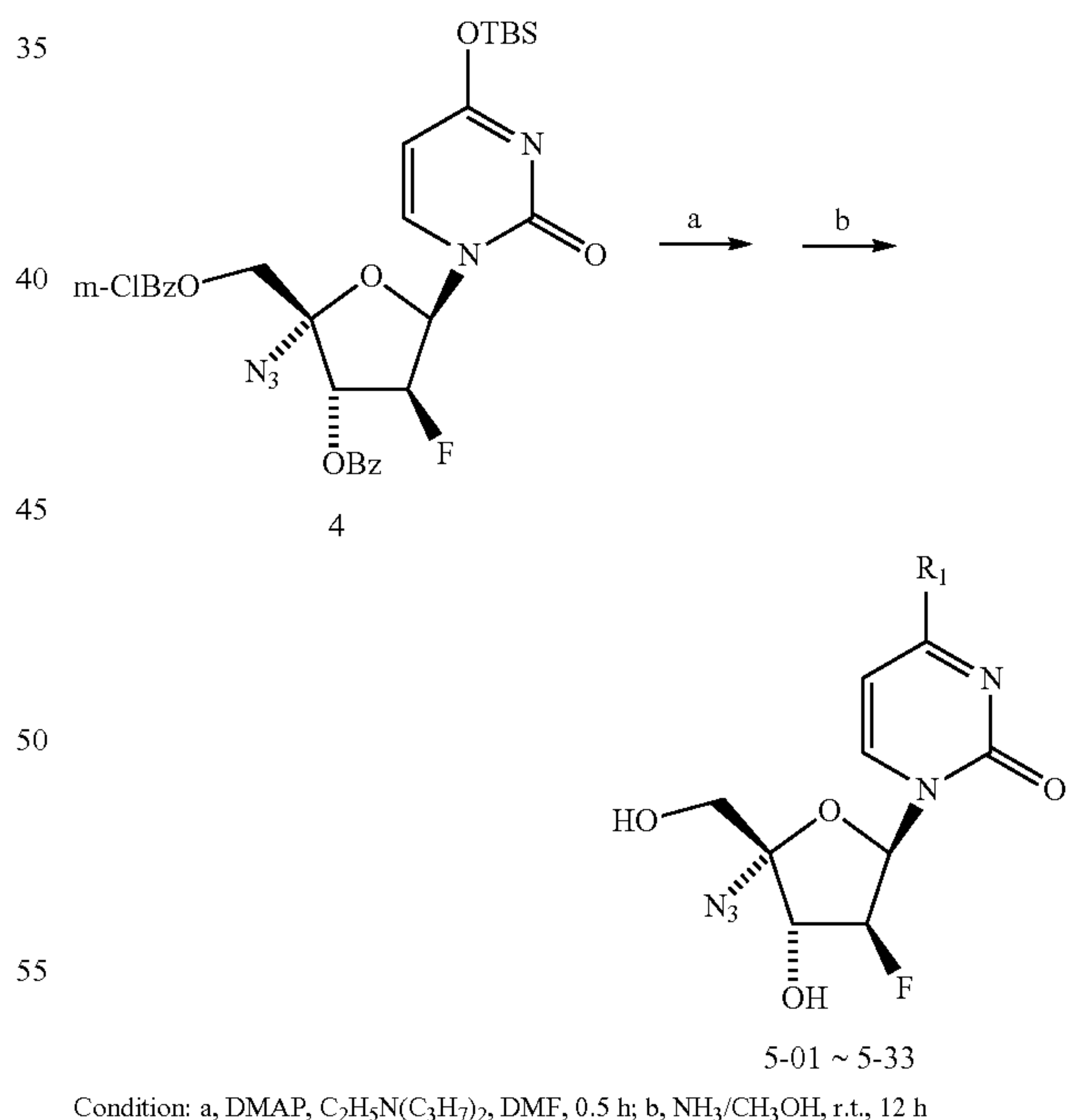
Scheme C. Synthesis of 4-substituted pyrimidine nucleoside 5-01 to 5-33
