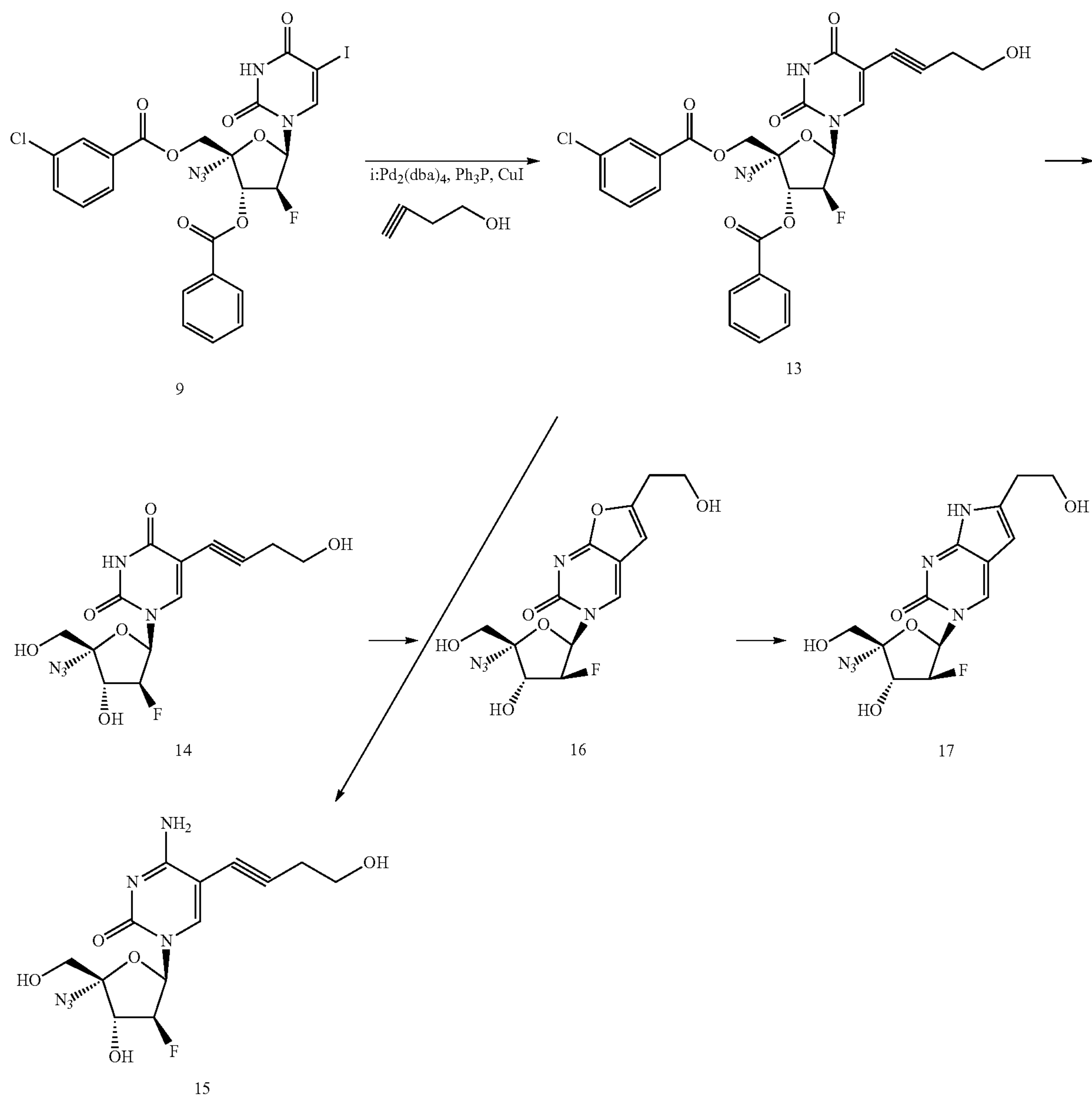
Scheme S. Synthesis of 5-substituted and bicyclic pyrimidine nucleoside derivatives.
