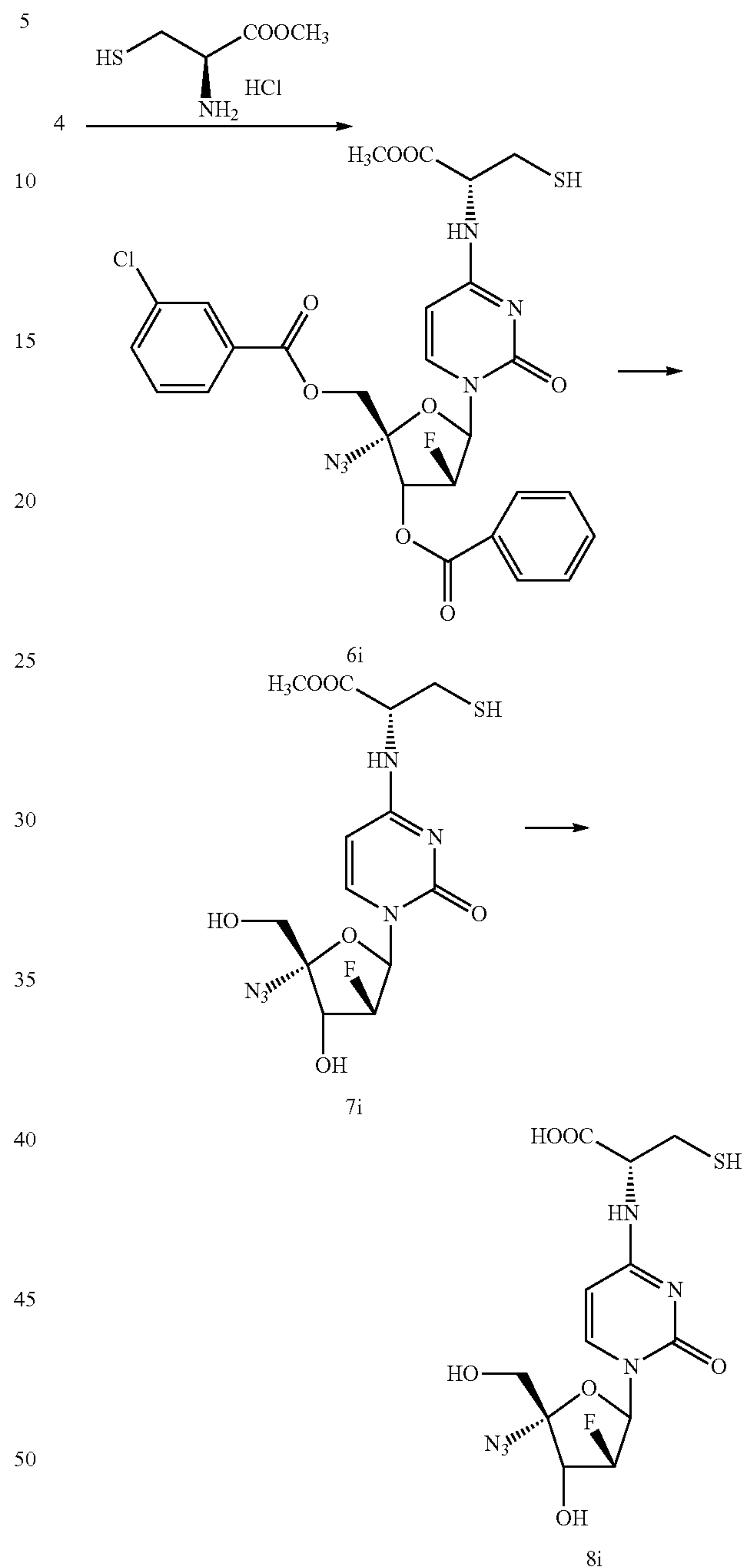
Scheme L. Synthesis of a pyrimidine nucleoside derivative with amino acid substitution at position 4.
