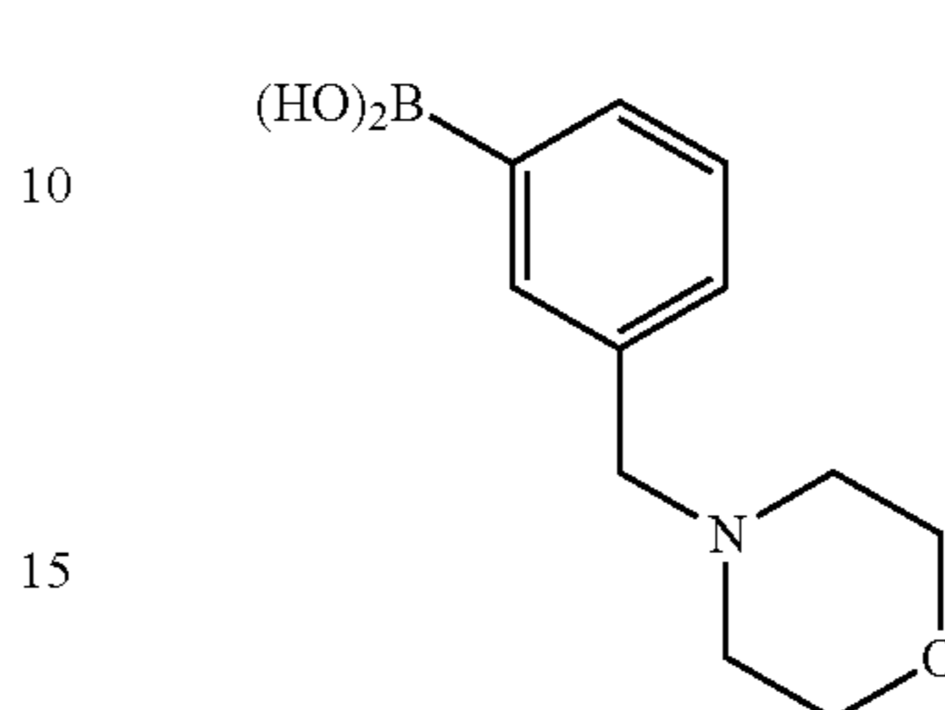
Scheme 2. Boronic acids selected for incorporation into novologue X scaffold.
