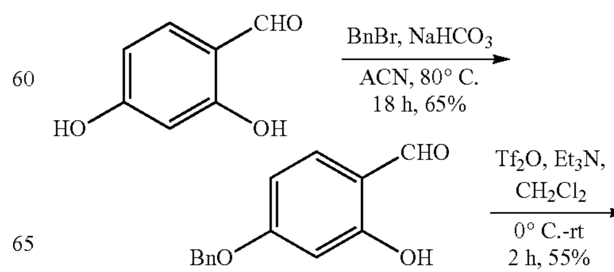
Scheme 6. Synthesis of phenol core intermediate 23.
