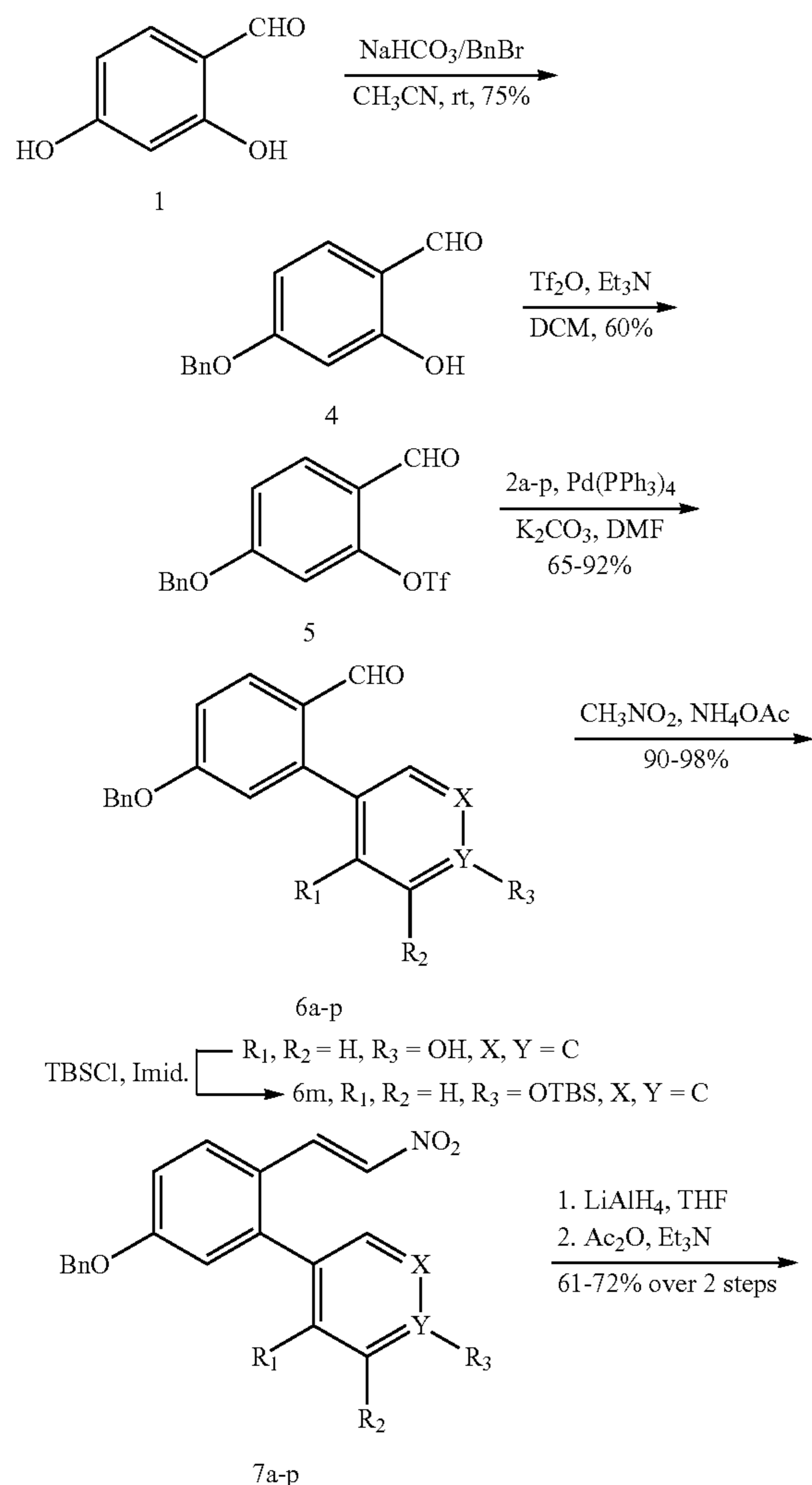
Scheme 3. Synthesis of ethyl acetamide side chain containing novologues.
