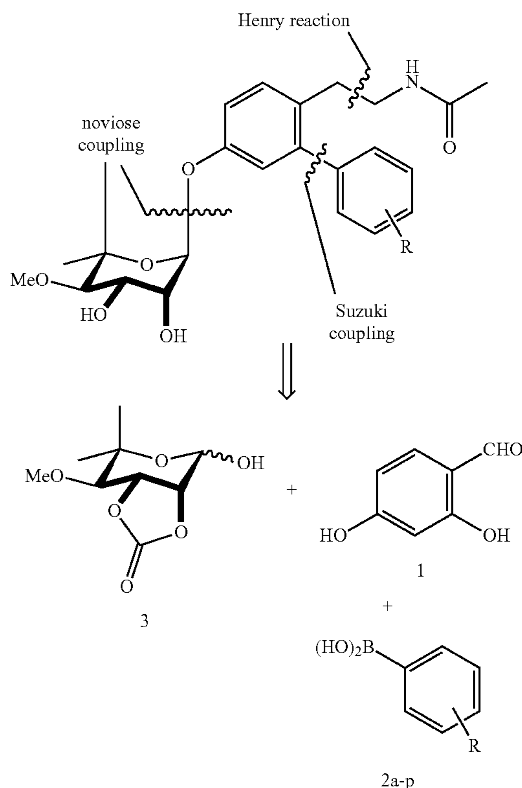
Scheme 1. Retrosynthetic analysis for the construction of novologue.
