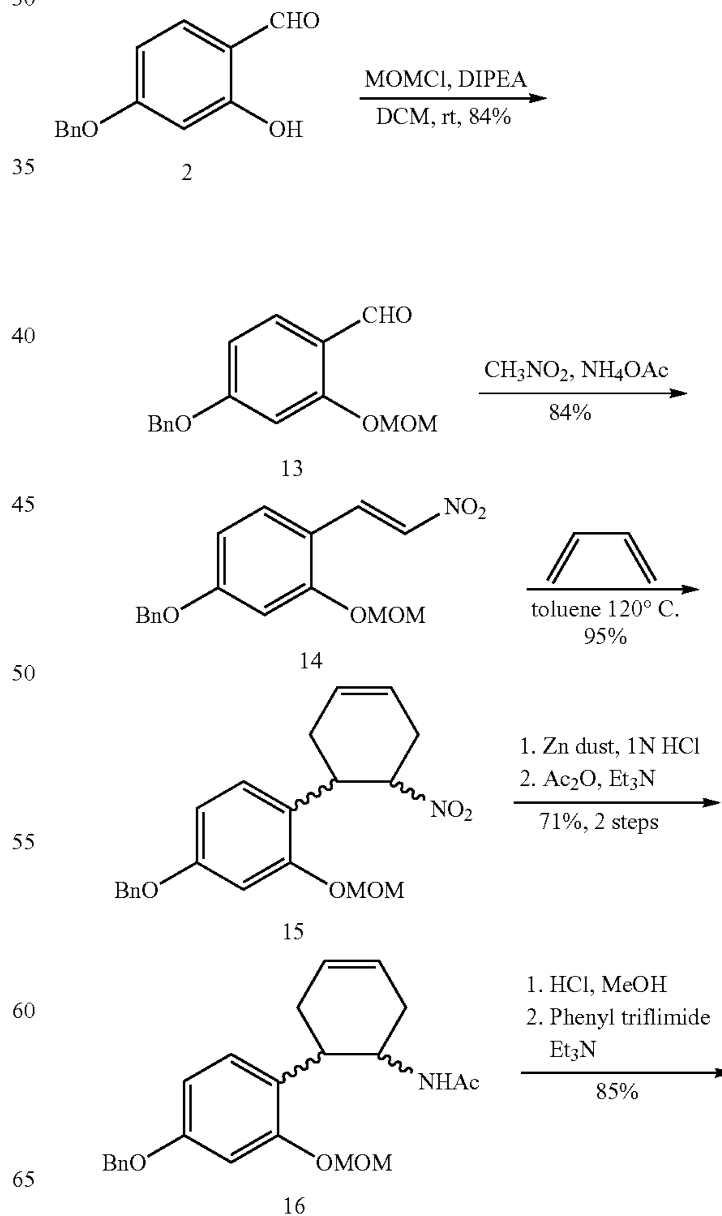
Scheme 4. Synthesis of cyclohexene containing novologues.
