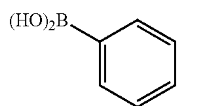
Scheme 2. Boronic acids selected for incorporation into novologue X scaffold.
