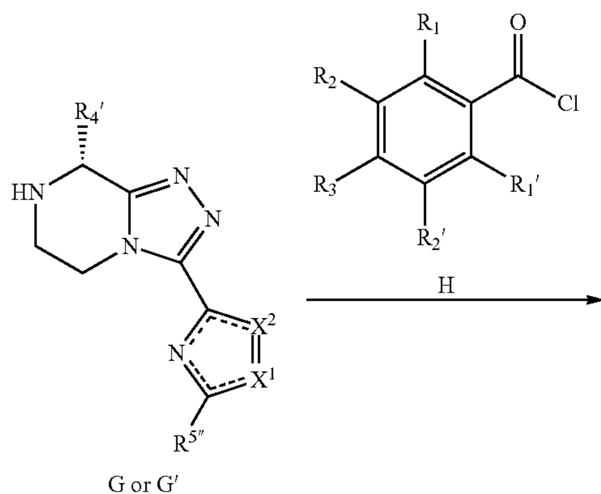
Scheme 16: Acylation.
