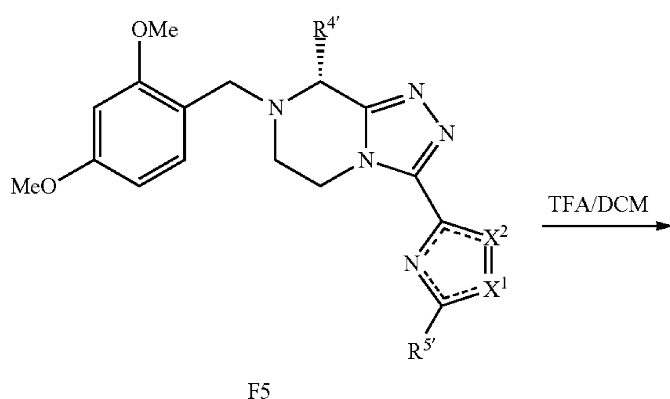
Scheme 14: DMB deprotection.
