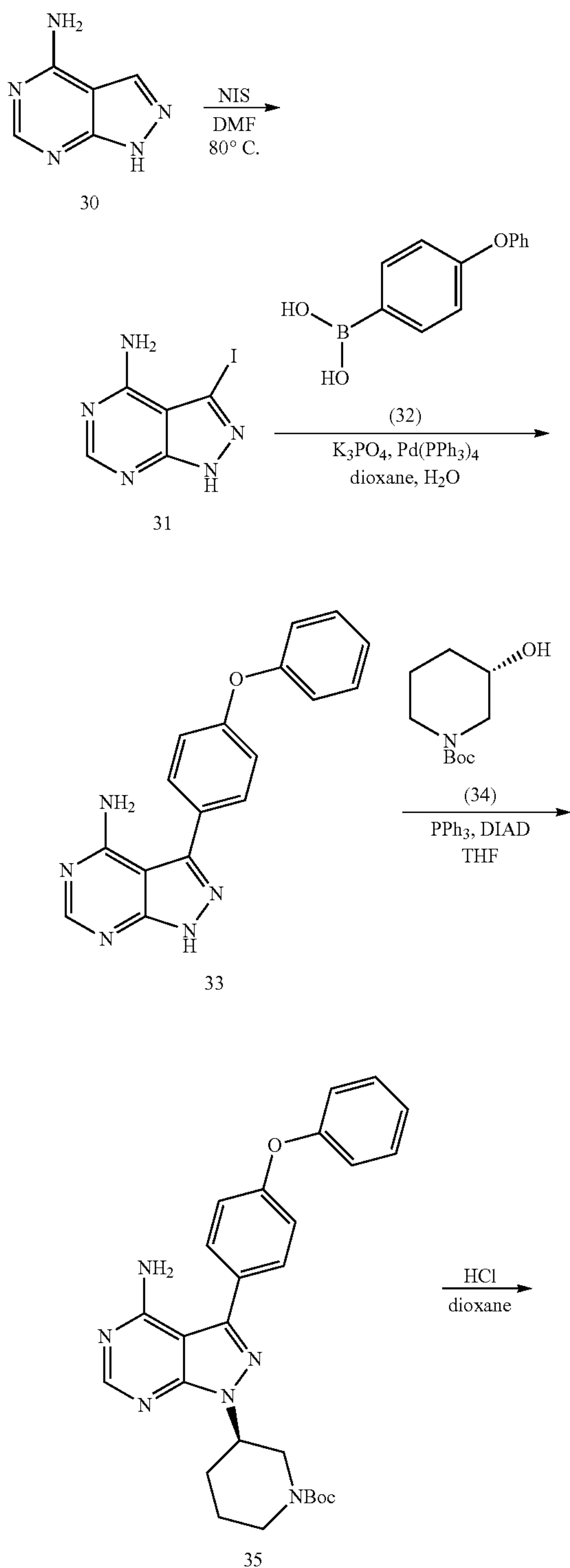
Scheme 5. Preparation of Compound 122
