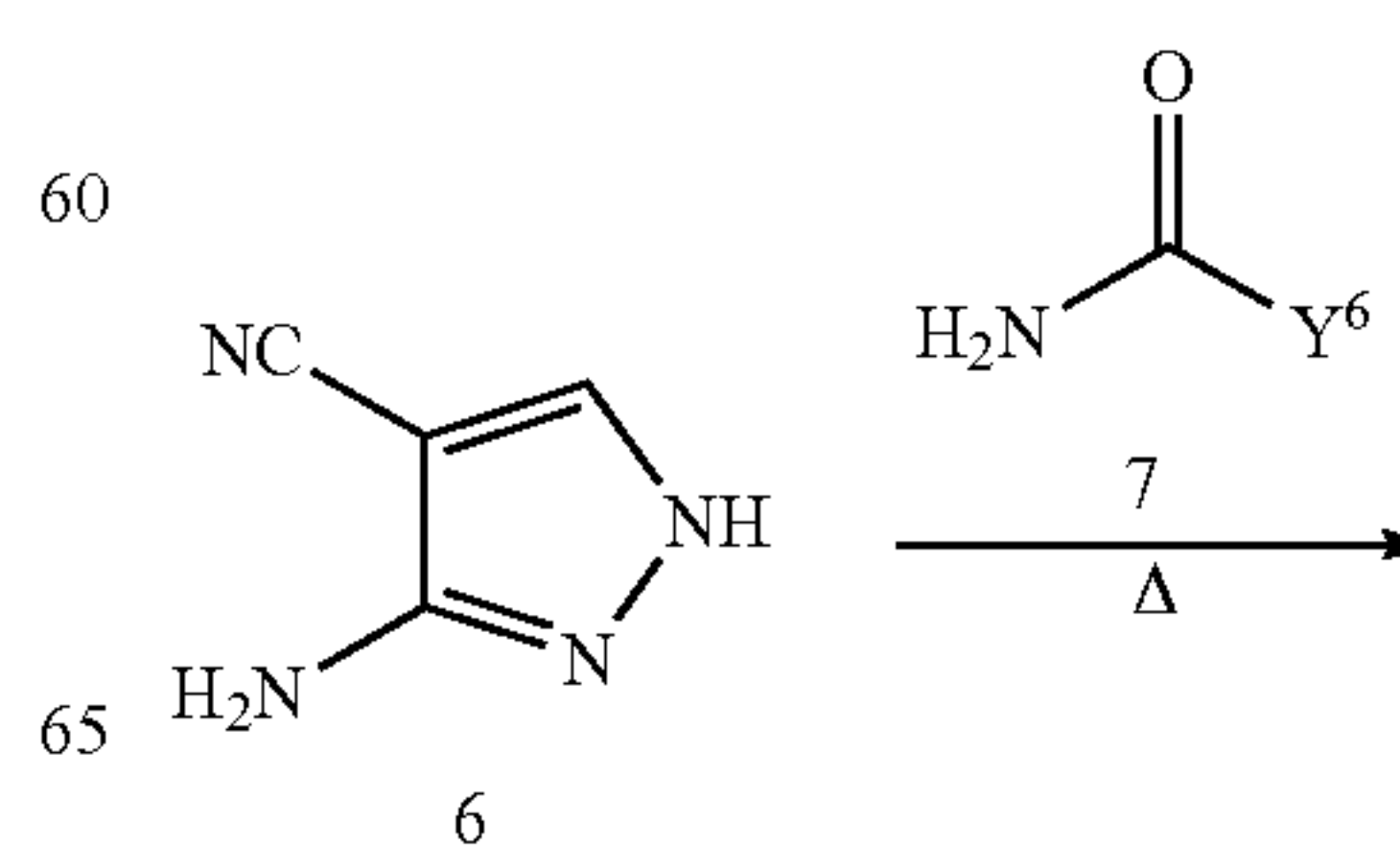
Scheme 2. Synthesis of compound 2 (Scheme 1):
